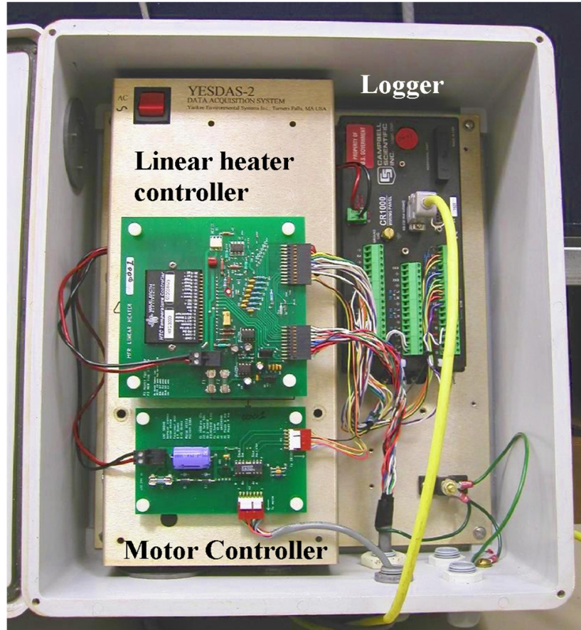
Figure 2. The Logger and system controller boards that comprise the new logging system for the ARM MFRSRs. Shown in this picture are the CR1000 data logger, the proportional (linear) heater controller, and the motor controller.
