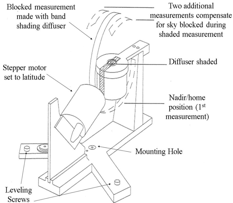
Figure 3. The graphics below are of a visible MFRSR. The main components are the head, which houses the filter detectors and amplification circuitry; the stepper motor with shadowband; and the mounting frame. The instrument is aligned such that the motor is toward the equator. The stepper motor and shadowband alternately shade and unshade the diffuser, allowing measurements of global (sometimes called total) and diffuse irradiance at six narrowband channels and one open channel to be made. Direct irradiance is calculated from the global and diffuse measurements.
