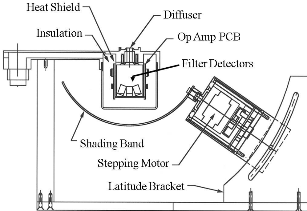
Figure 4. Cut-out view of the MFRSR.
