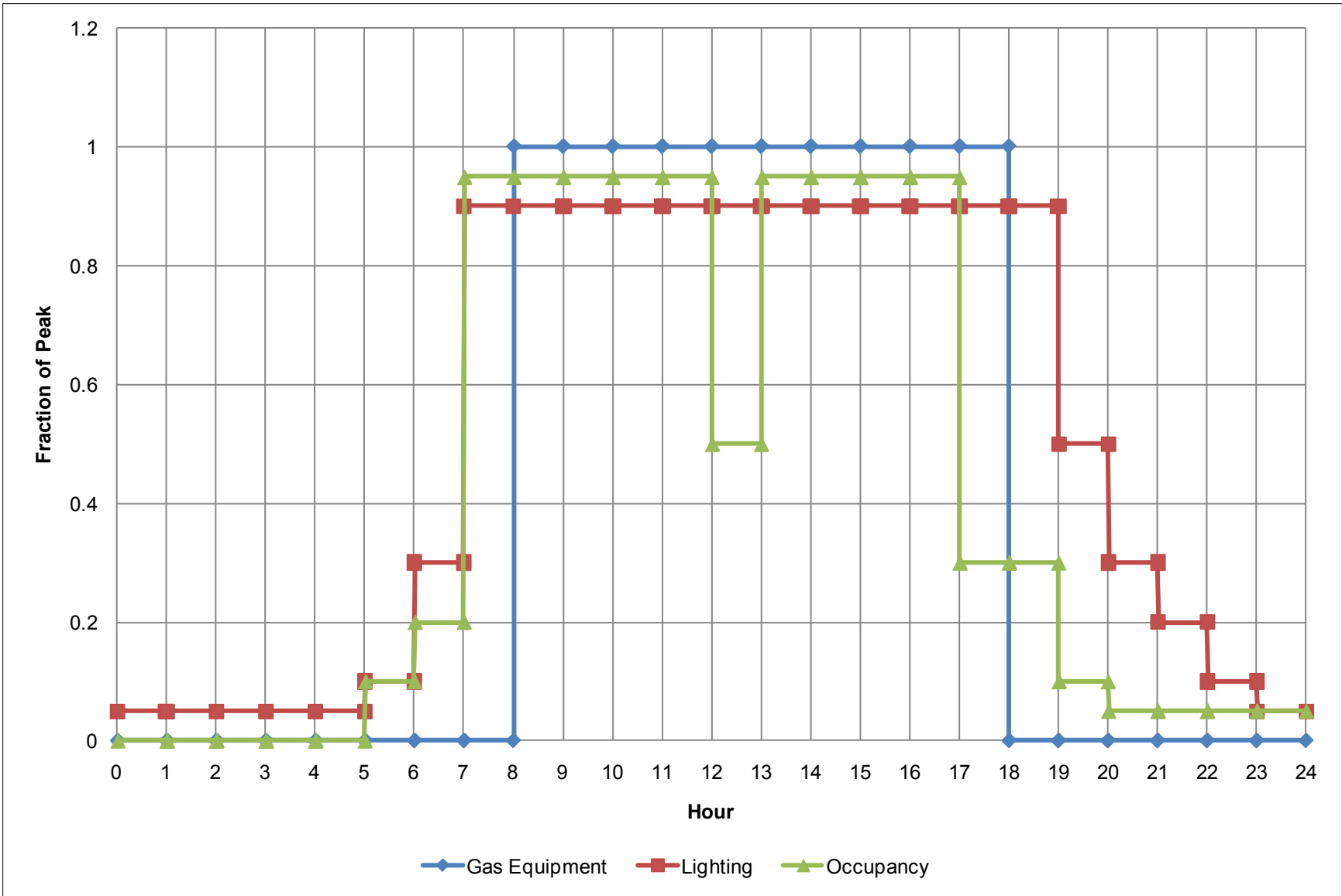
Figure E-9 Laundry zone occupancy, lighting, and equipment schedules (Credit: Daniel Studer/NREL)
