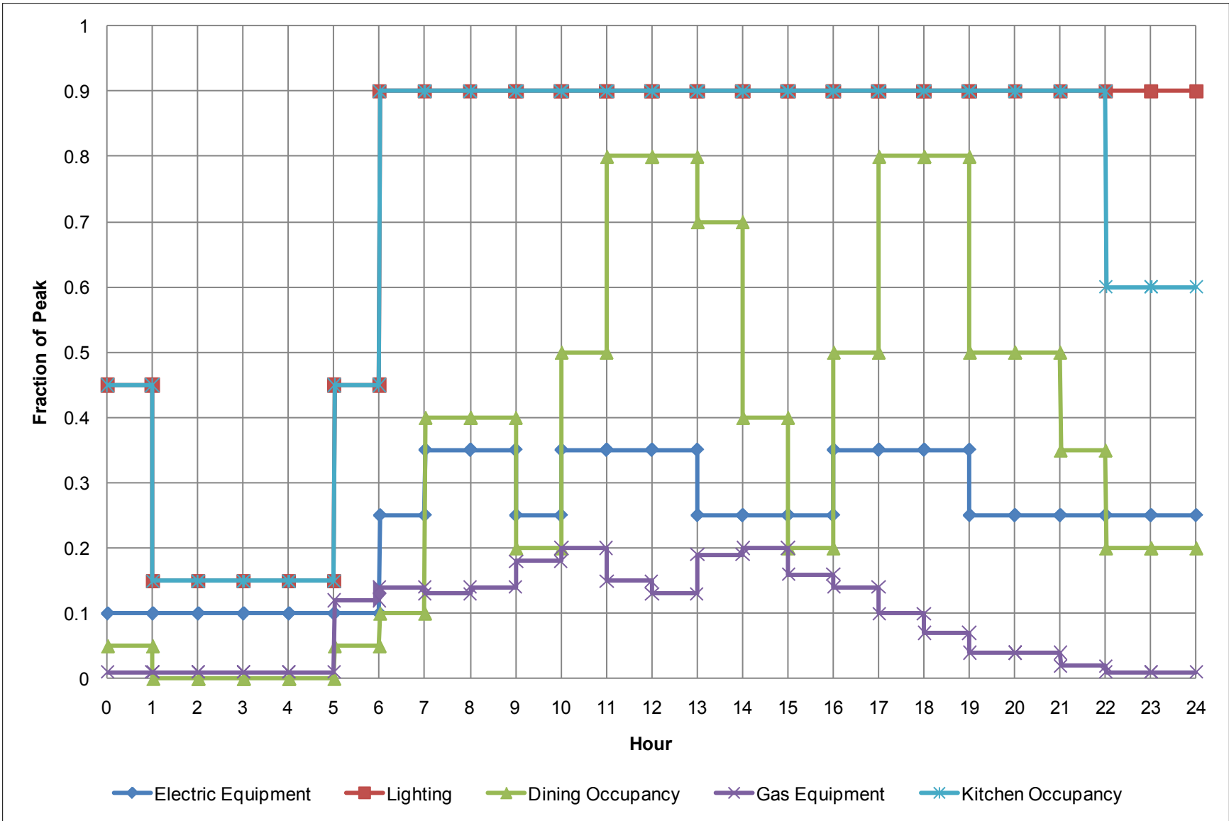
Figure E-7 Food service-related area occupancy, lighting, and equipment schedules (Credit: Daniel Studer/NREL)
