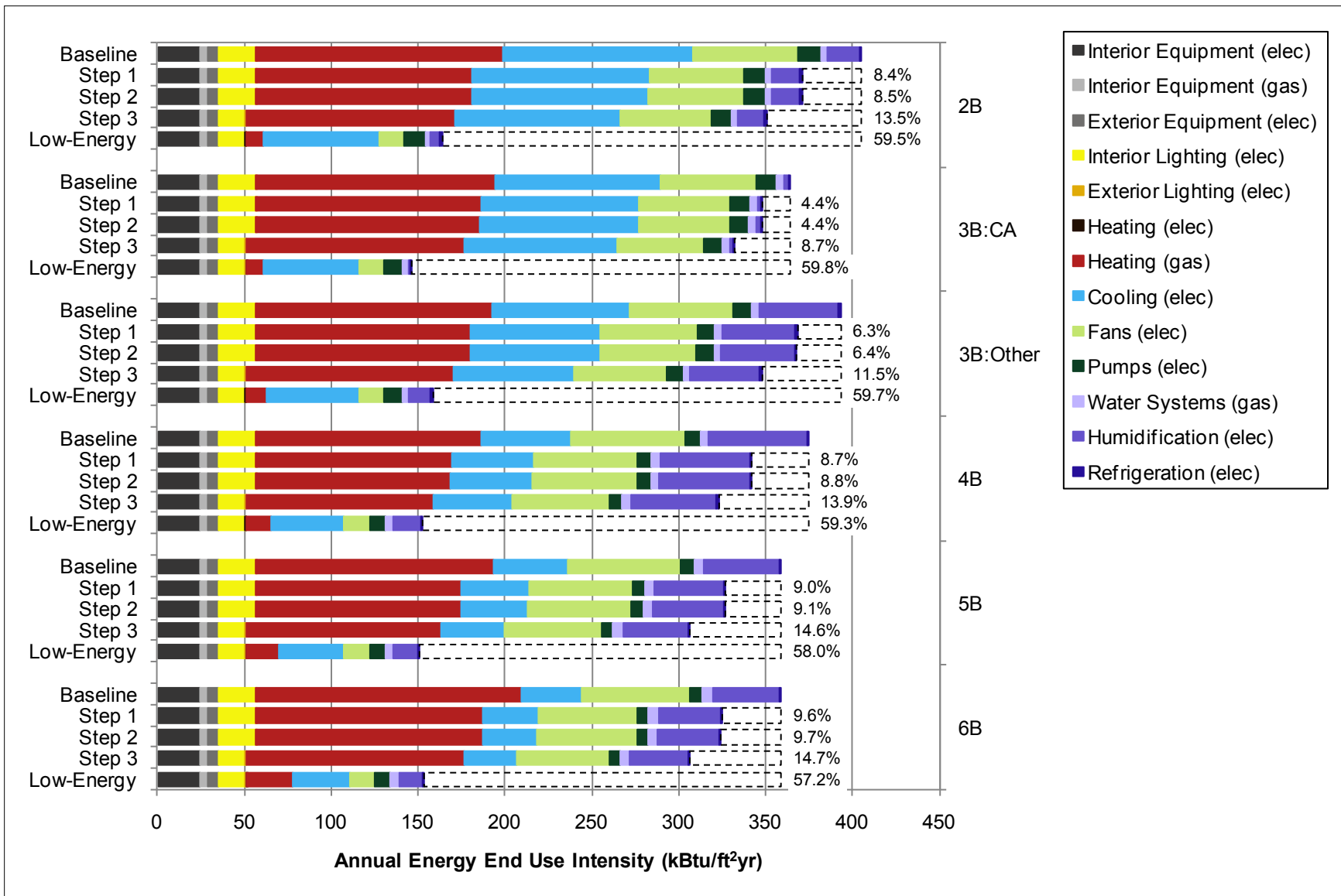
Figure 5-3 Bundle analysis results for arid climate zones (Credit: Eric Bonnema/NREL)
