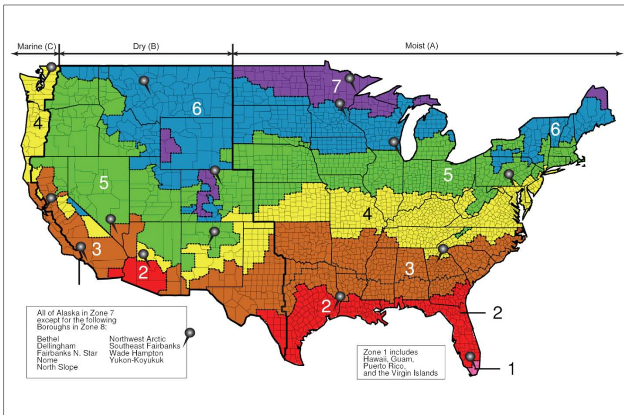
Figure 2-1 DOE climate zones and representative cities (Credit: (DOE 2005))
