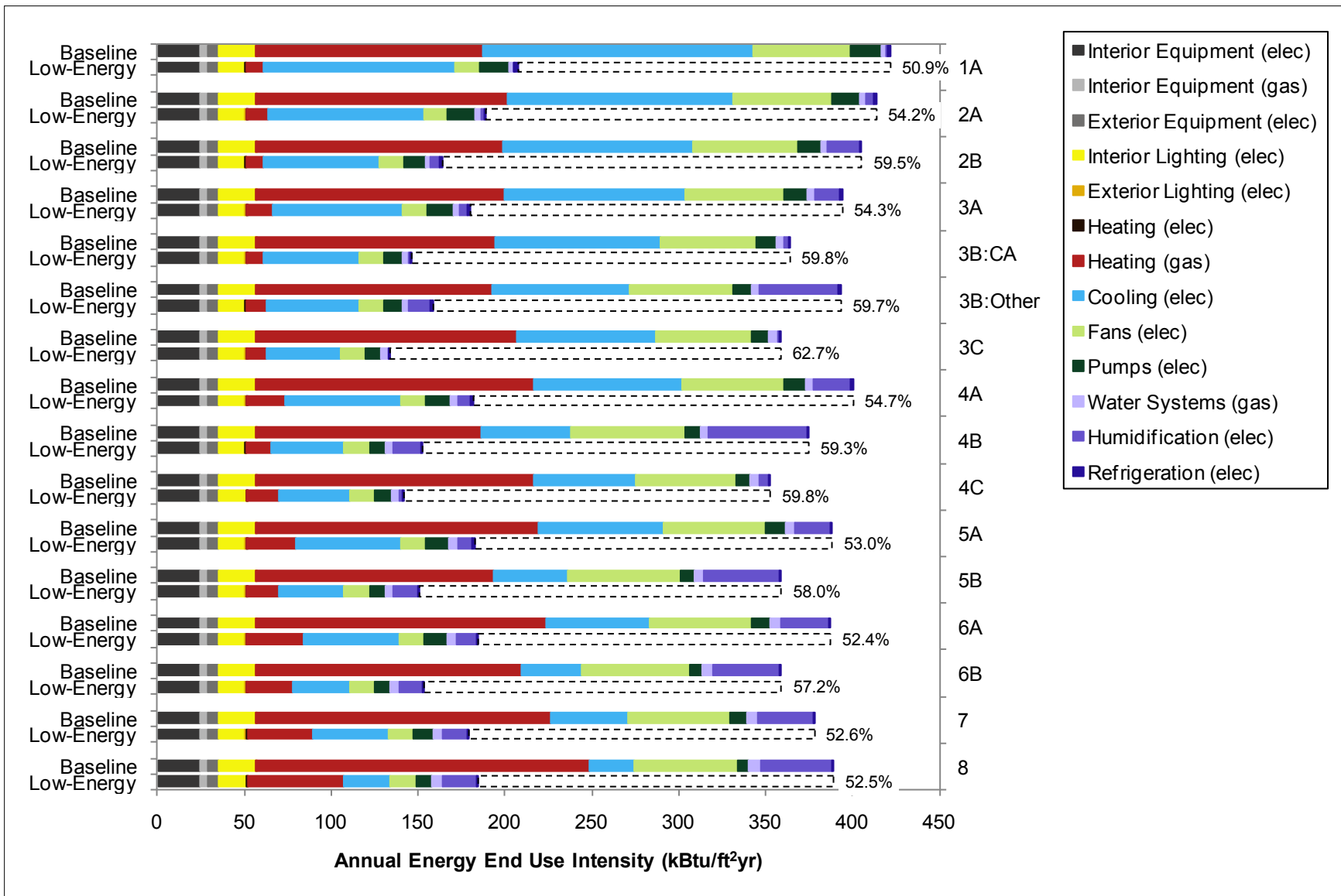
Figure 5-1 EUI by end use for baseline and low-energy models (Credit: Eric Bonnema/NREL)
