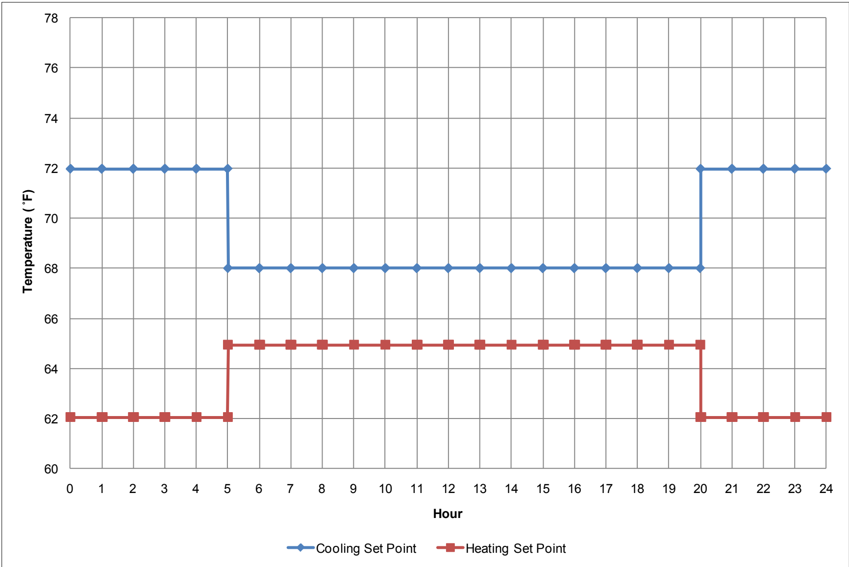
Figure E-10 Laundry zone set point schedules (Credit: Daniel Studer/NREL)
