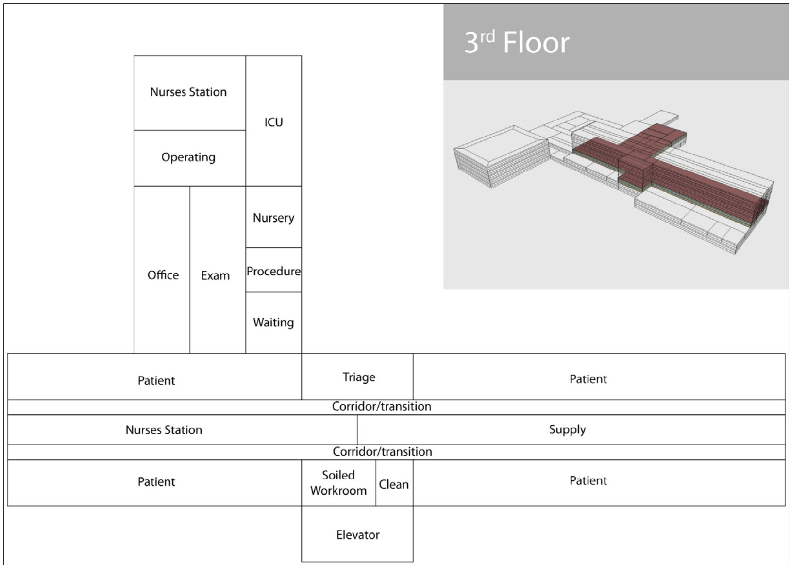
Figure 3-4 Large hospital prototype third floor plan (Credit: Marjorie Schott/NREL)
