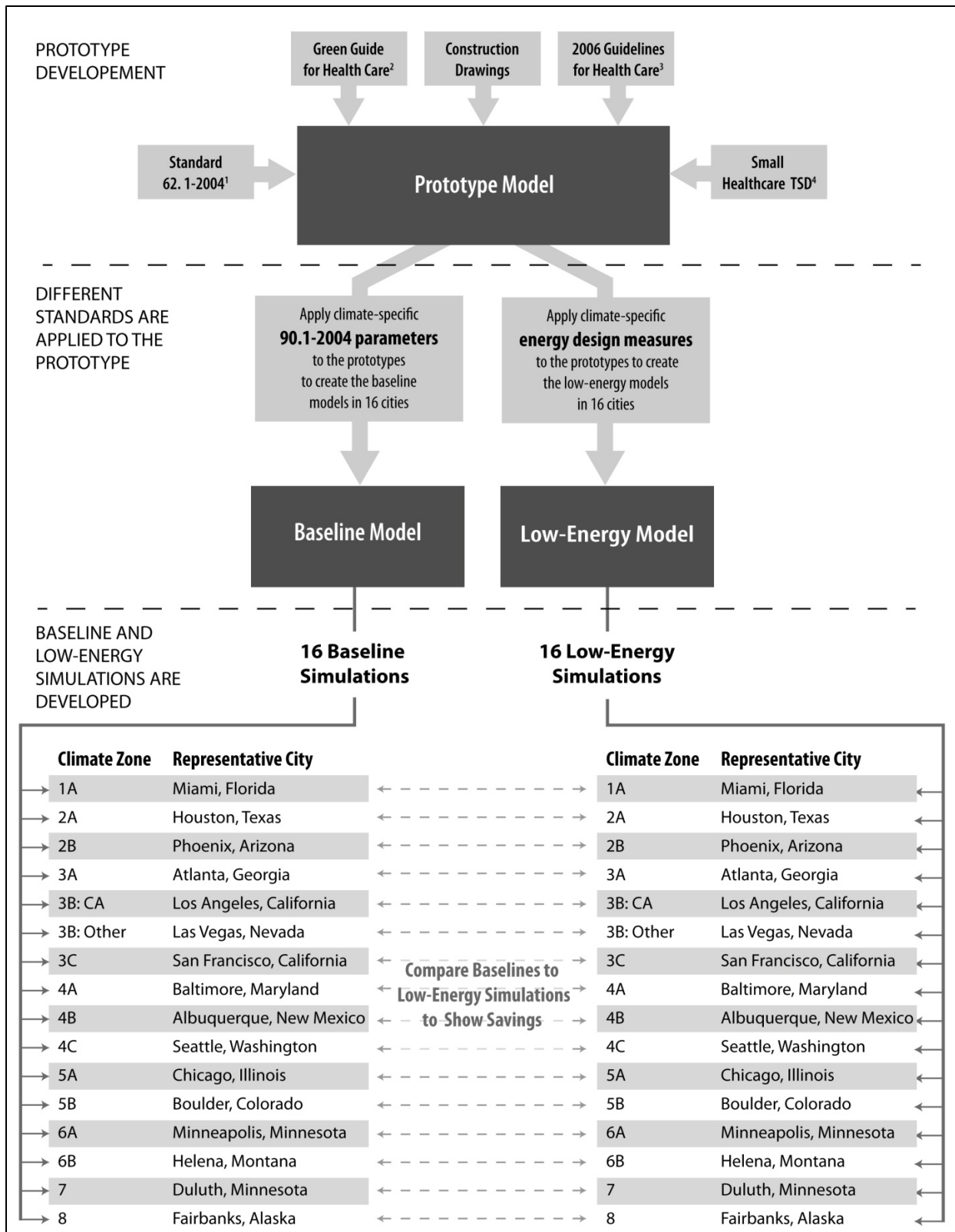
Figure 2-2 Flow diagram of modeling process (Credit: Marjorie Schott/NREL)
