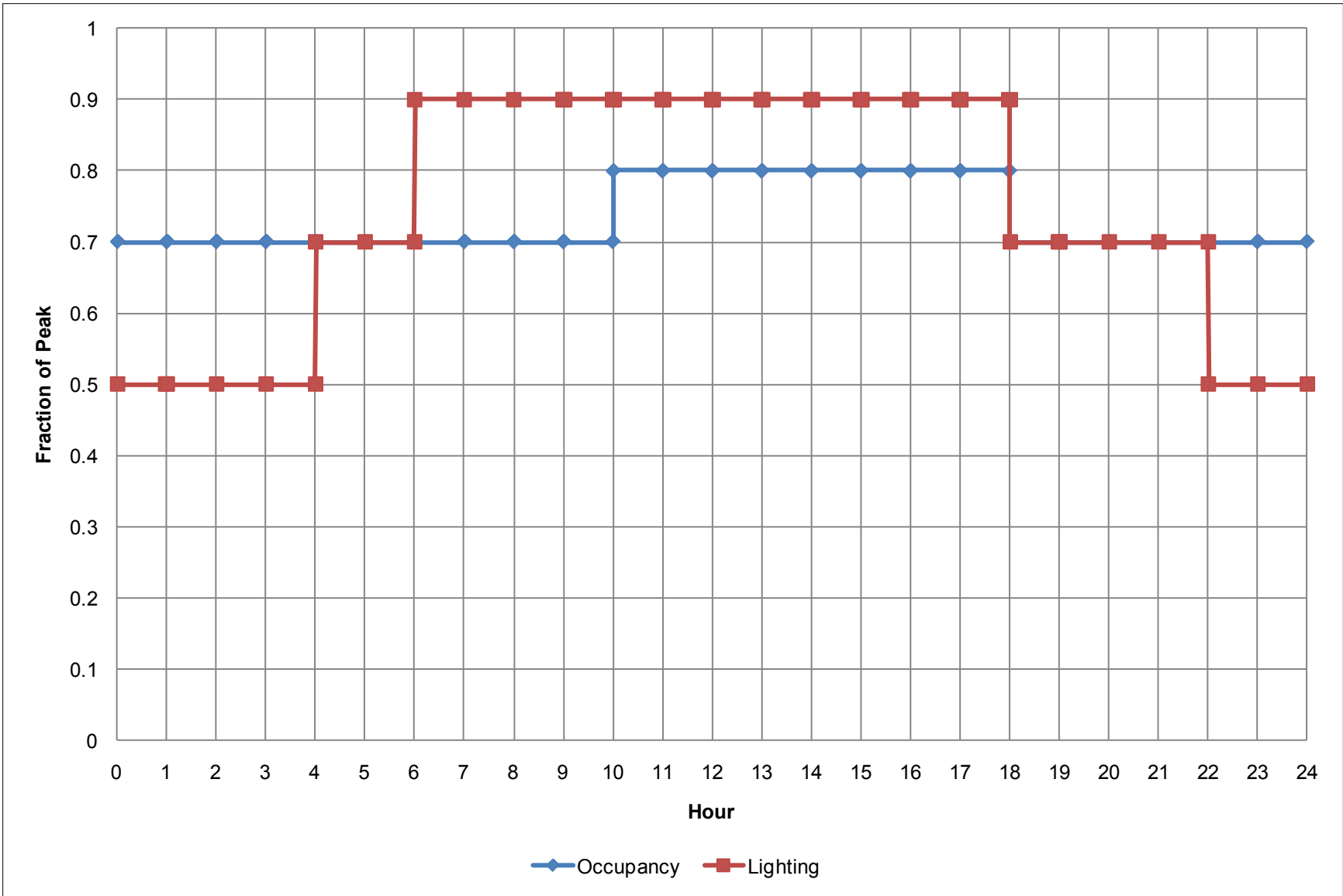
Figure E-2 Patient area occupancy and lighting schedules (Credit: Daniel Studer/NREL)
