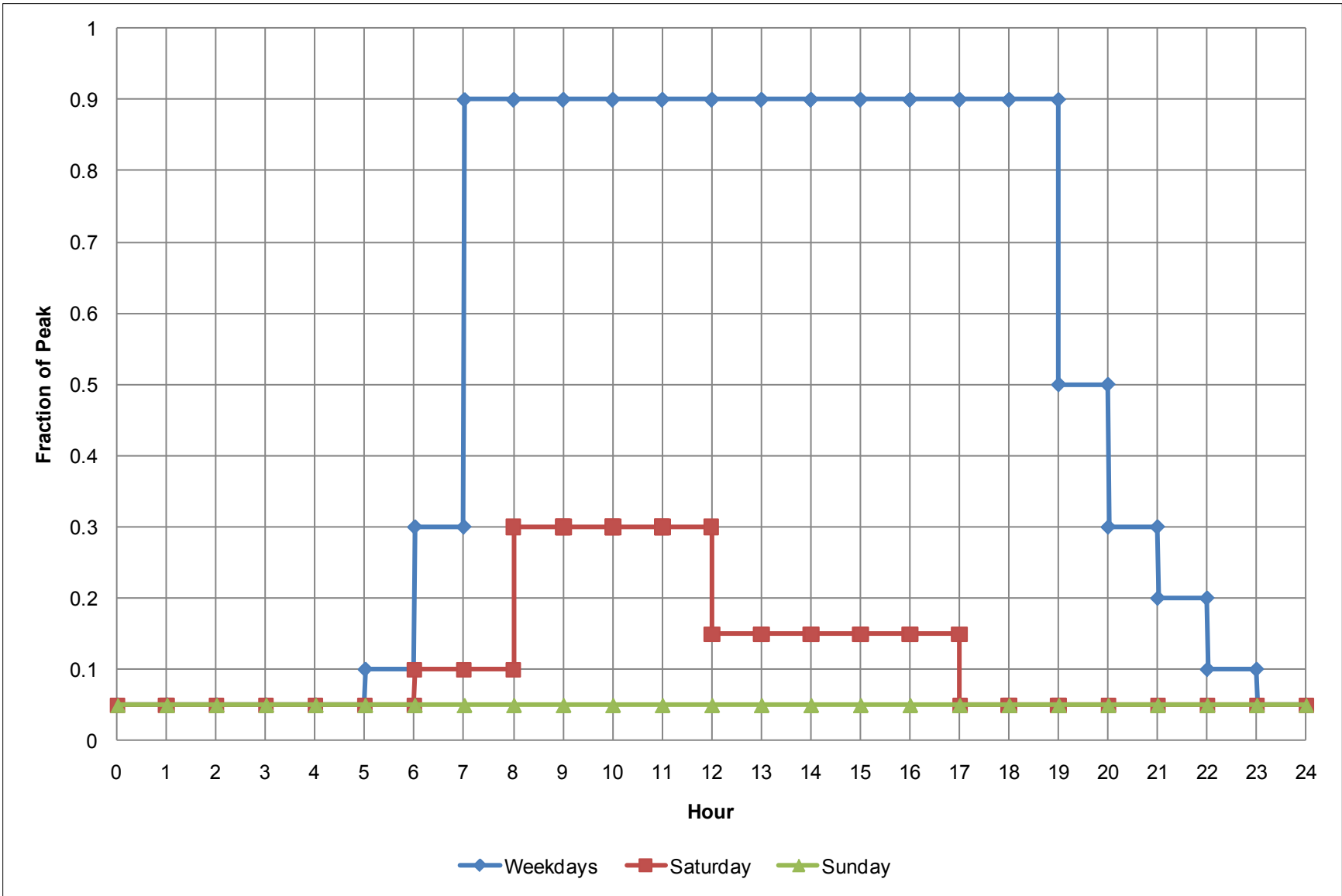
Figure E-4 Office lighting schedules (Credit: Daniel Studer/NREL)
