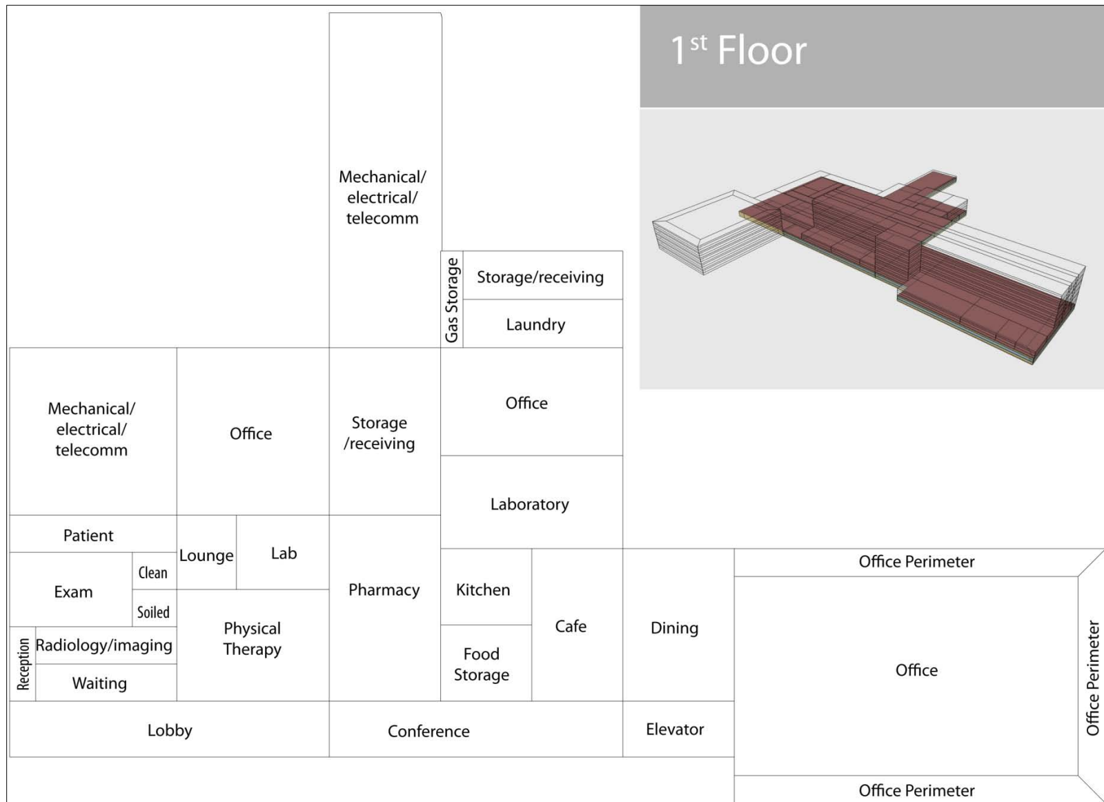
Figure 3-2 Large hospital prototype first floor plan (Credit: Marjorie Schott/NREL)
