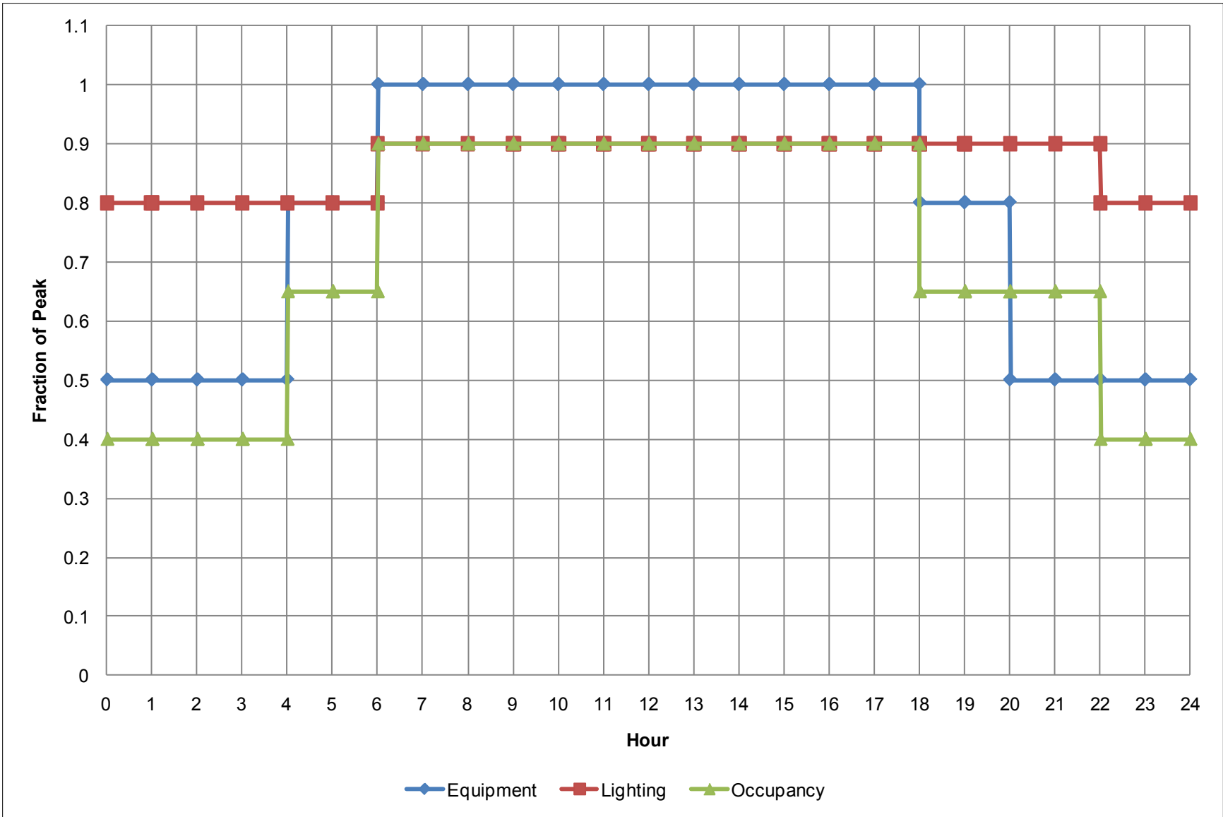
Figure E-1 24/7 occupancy, equipment, and lighting schedules (Credit: Daniel Studer/NREL)
