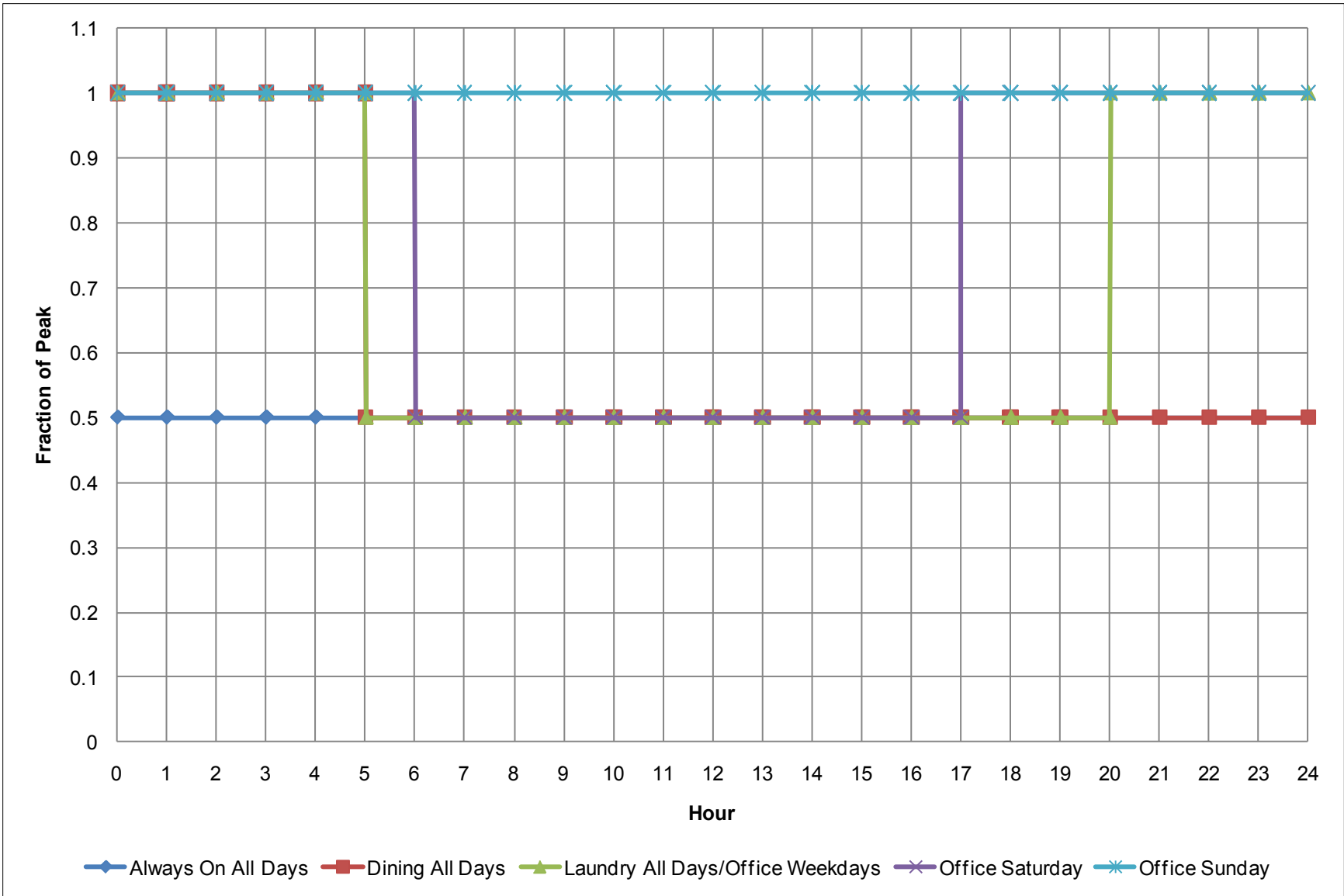
Figure E-11 Infiltration schedules (Credit: Daniel Studer/NREL)
