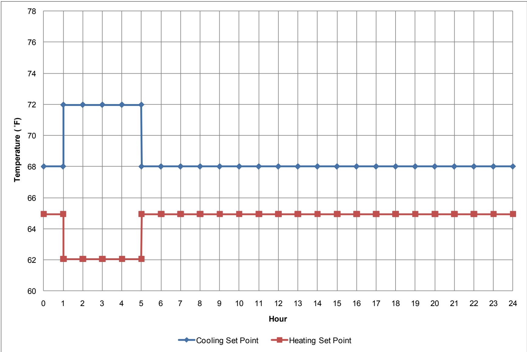
Figure E-8 Food service-related area set point schedules (Credit: Daniel Studer/NREL)
