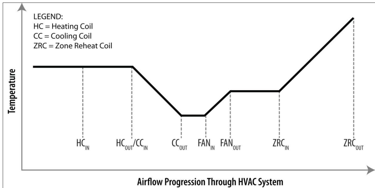
Figure 4-1 HVAC system temperature diagram (Credit: Marjorie Schott/NREL)
