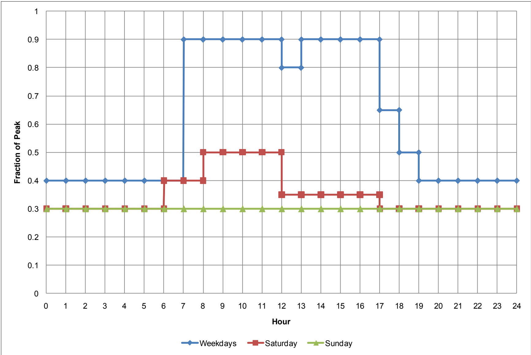
Figure E-5 Office equipment schedules (Credit: Daniel Studer/NREL)
