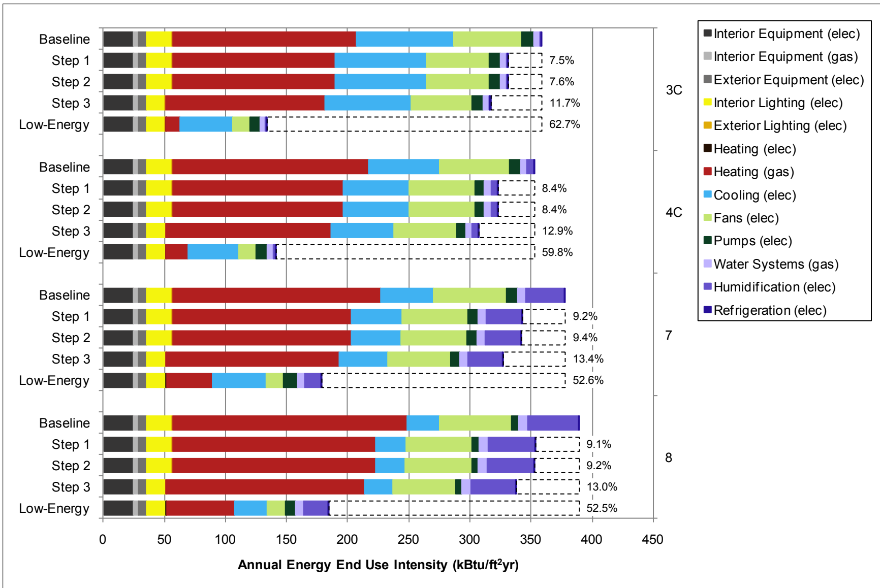
Figure 5-4 Bundle analysis results for marine and cold climate zones (Credit: Eric Bonnema/NREL)
