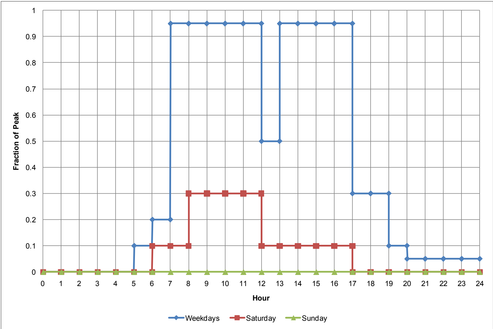
Figure E-3 Office occupancy schedules (Credit: Daniel Studer/NREL)
