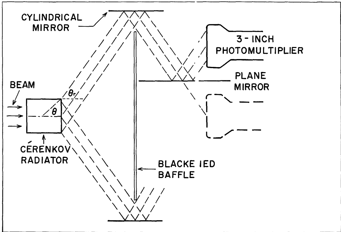
VELOCITY-SELECTING ČERENKOV COUNTER (C 2)
