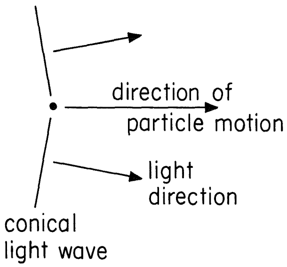
slower particle
