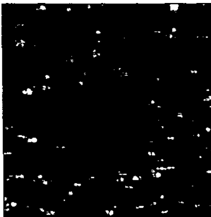
Figure 1. Locations of individual rhodamine 6G molecules on a silica surface imaged by near-field scanning optical microscopy. The image size is approximately 8 \mu\text{m} by 8 \mu\text{m} . The image is formed by transmitting light through a 0.25 \mu\text{m} aperture, scanning the aperture -10 nm above a silica surface, and detecting fluorescence at each position. Achieving single-molecule sensitivity on a surface allows observation of the unique orientation, photobleaching behavior, and fluorescence lifetime of individual molecules that are otherwise buried in ensemble measurements. 6
