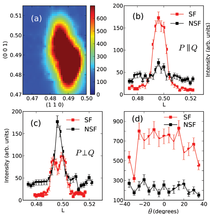
FIGURE 2: Neutron diffraction measurements of the (111) oriented BiFeO 3 film. (a) Reciprocal space map taken in the HHL zone using unpolarized neutrons; (b,c) intensity profiles taken with (b) P \parallel Q (neutron polarization) \parallel Q (scattering vector), and (c) P \perp Q ; (d) changes in scattering intensities with the polarization rotated by an angle \theta within the scattering plane relative to the scattering wave vector direction. The red and black squares represent spin-flip and non-spin-flip scattering, respectively. The data have been corrected for spin transport.
