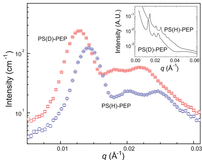
FIGURE 3: SANS profiles obtained from 15 % volume fraction PS(D)-PEP (red) and PS(H)-PEP (blue) in an isotopic squalane mixture (42 % C_{30}H_{62} and 58 % C_{30}D_{62} volume fractions) at 30 °C. Inset shows the corresponding SAXS patterns.
