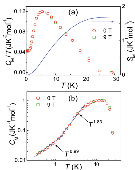
FIGURE 3: (a) The temperature dependences of the reduced heat capacity C_M/T and the magnetic entropy S_M ; (b) The temperature dependence of C_M (open symbols). The solid lines are fits as described in the text.
