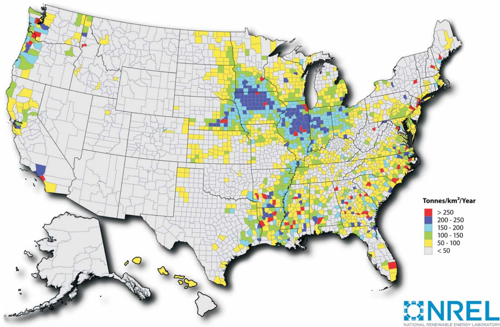
Figure 4.19 Biomass Resources
