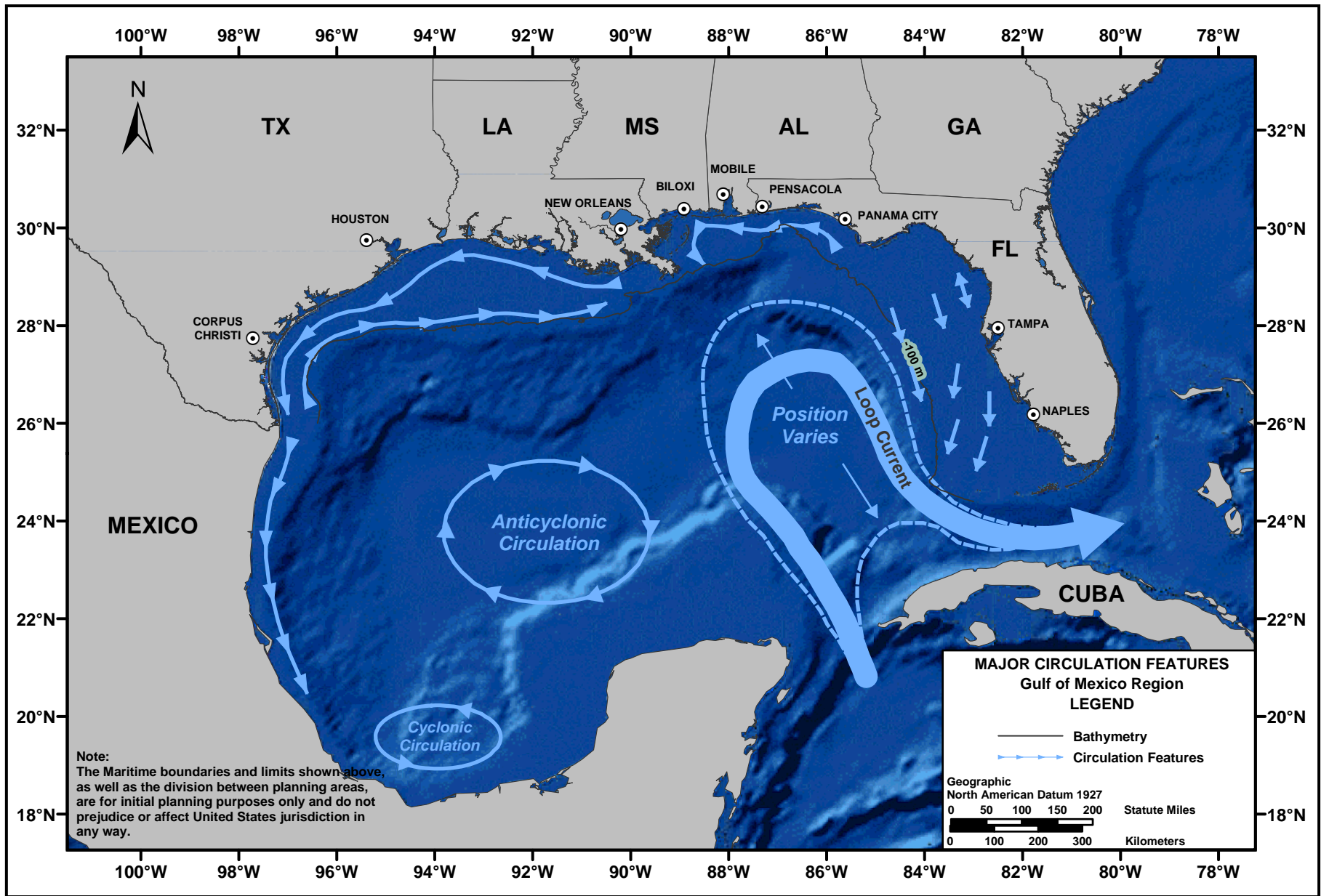
Figure III-4. Major Circulation Features -- Gulf of Mexico
