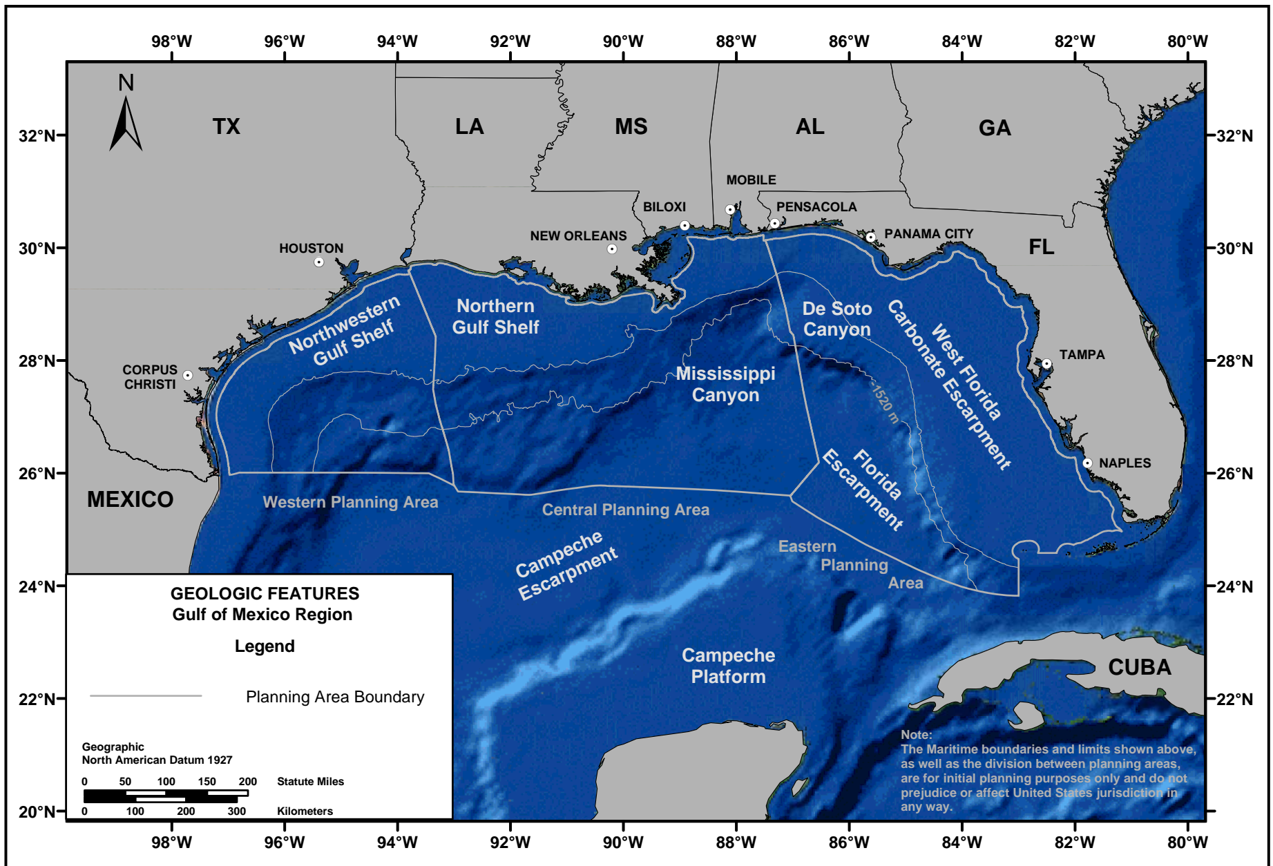
Figure III-1. Geologic Features -- Gulf of Mexico
