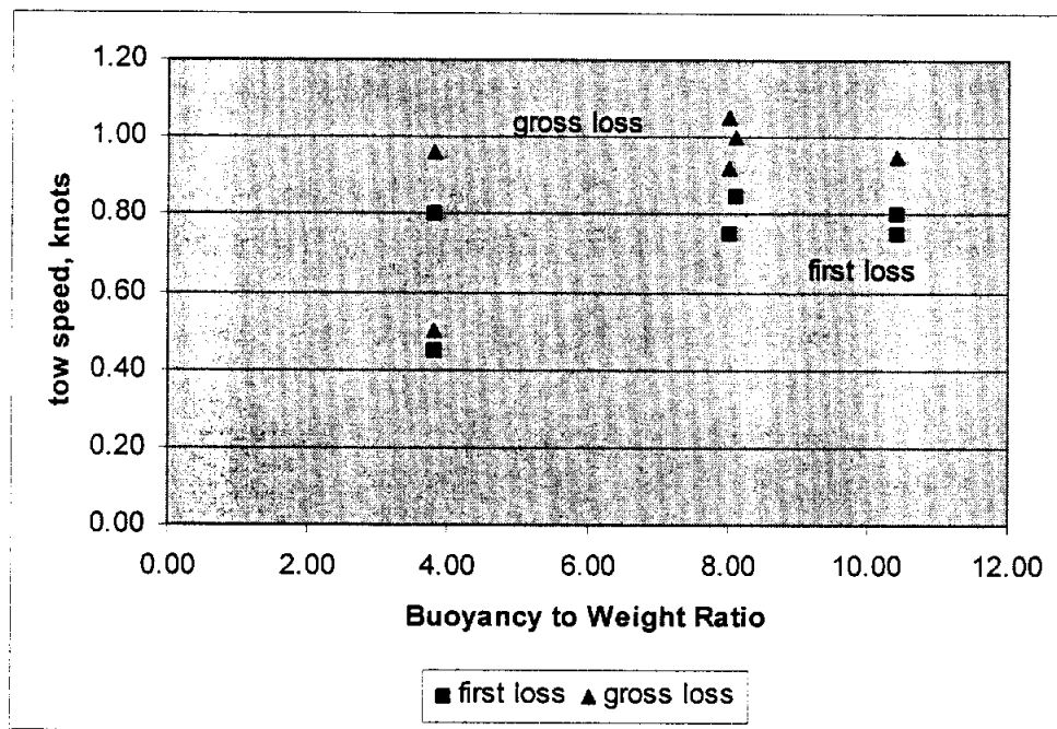
Figure 9: First and gross loss tow speeds, curtain boom, harbor chop
