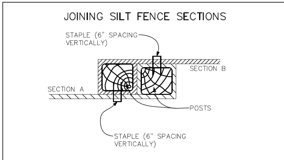
Figure 5-7: Silt Fence Joint Detail
