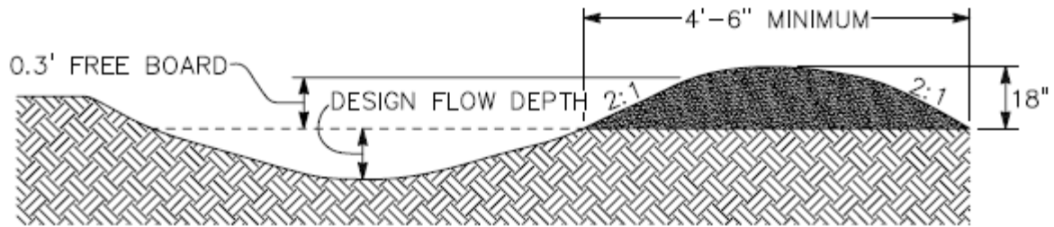
Typical Parabolic Diversion
