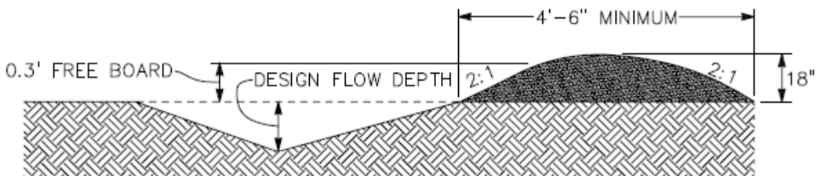
Typical Vee-Shaped Diversion
