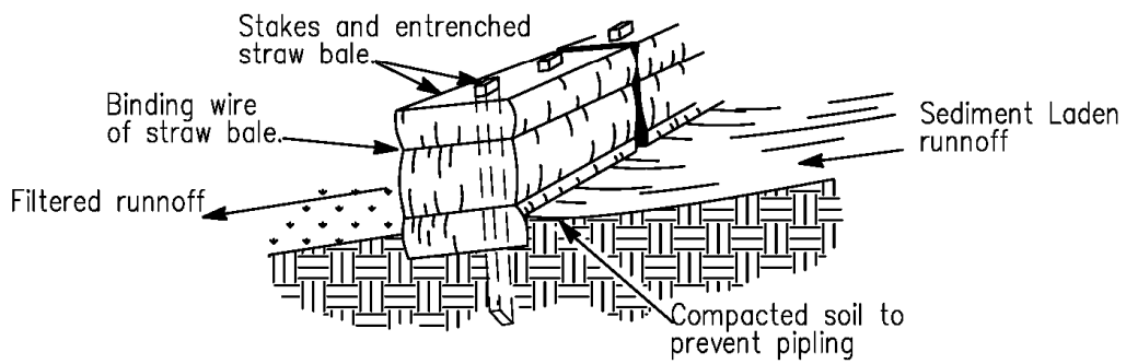
B. Cross-section of a properly installed straw bale.
