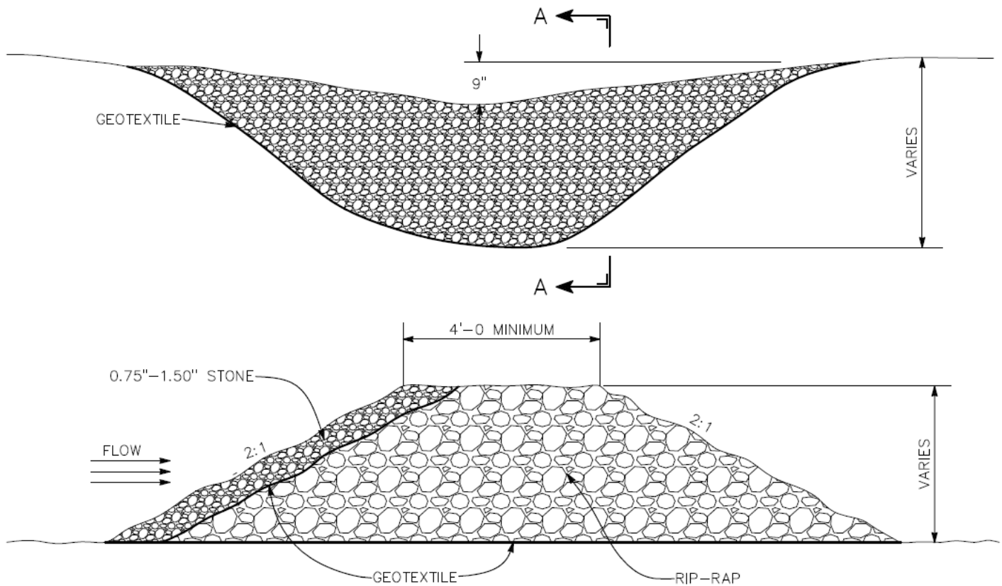
SECTION A-A DETAIL: ROCK FILTER DAM
