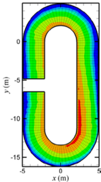
Exhibit 10.9. Open raceway pond example of physics-based algae cultivation system modeling and analysis. Such analysis can enable both performance prediction and pond system design optimization after appropriate refinement and validation with monitored field system data (Adapted from James and Varun, in press)
