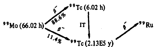
Fig. M-1 Decay diagrams for selected radioisotopes (continued).
