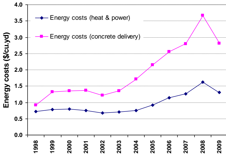
Figure 2. Energy costs per cubic yard of ready mixed concrete, 1998-2009
