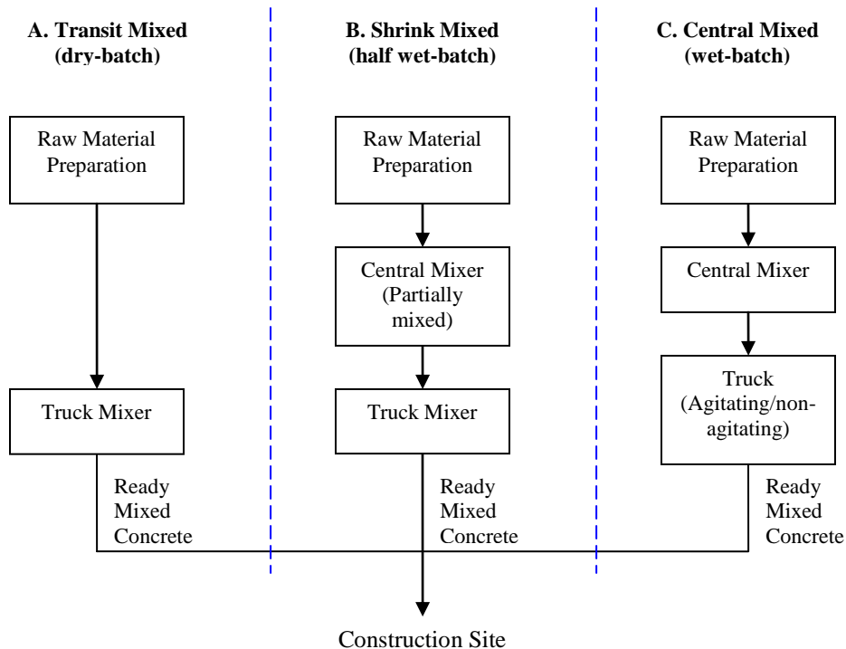
Figure 4. Ready mixed concrete production
