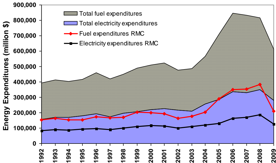
Figure 3. Energy expenditures in the U.S. concrete industry (excluding concrete delivery)
