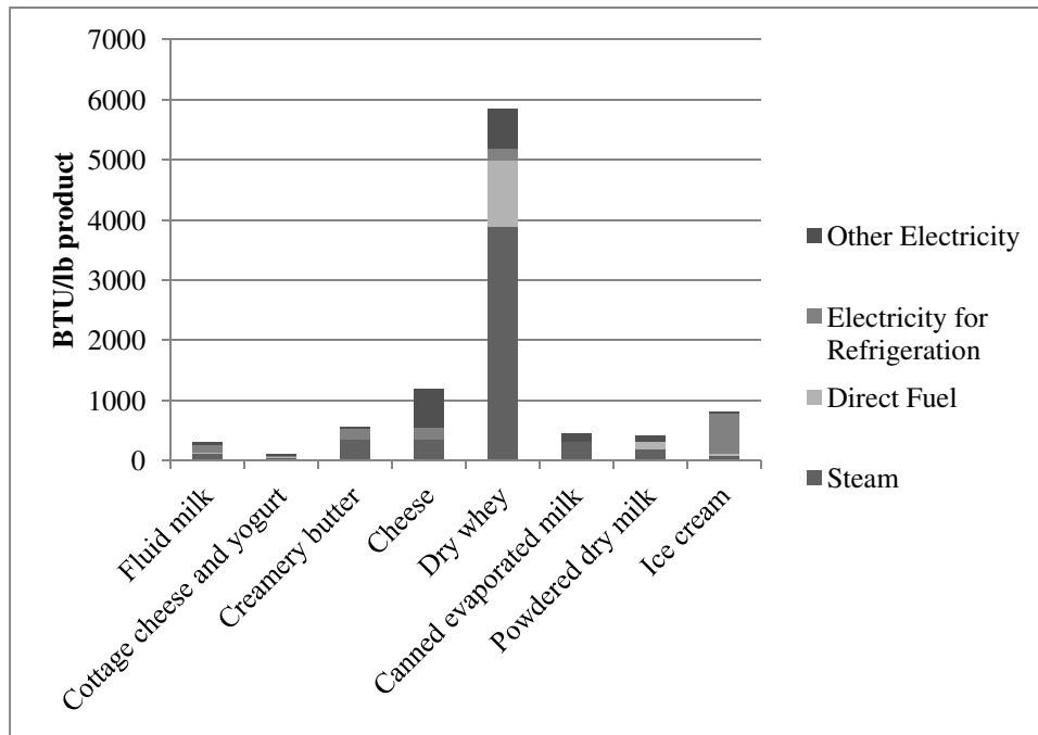
Figure 4.5. Comparison of process energy intensities of several dairy products
