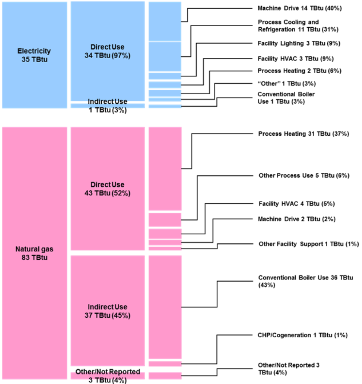
Figure 4.3. Estimated energy consumption and end uses in the U.S. dairy processing industry, 2006
