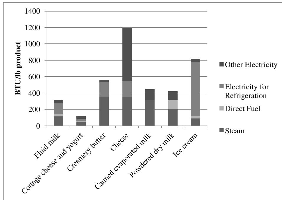
Figure 4.6. Comparison of process energy intensities of several dairy products, excluding dry whey
