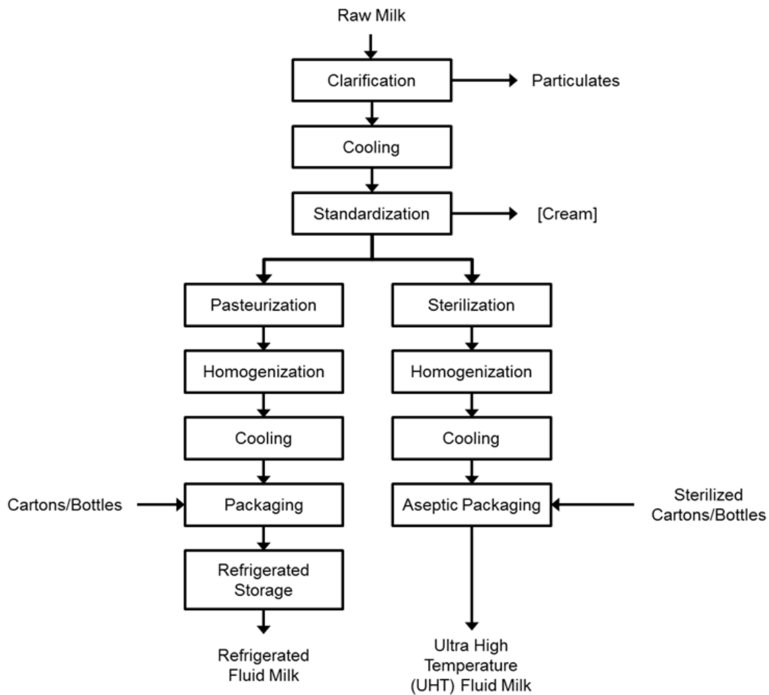
Figure 3.1. Process diagram for fluid milk production
