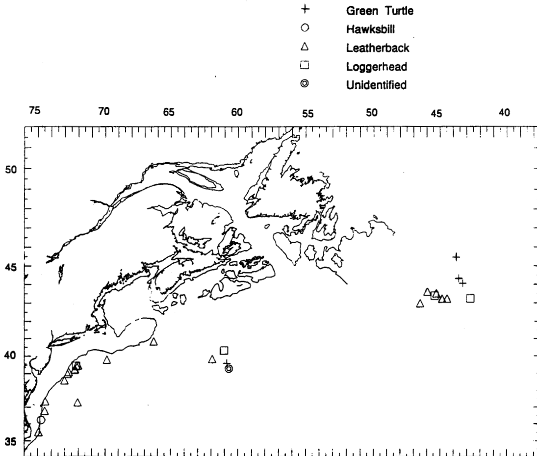
Figure 4. Sea turtle interactions by species from NEFSC observed pelagic longline trips in 1992.
