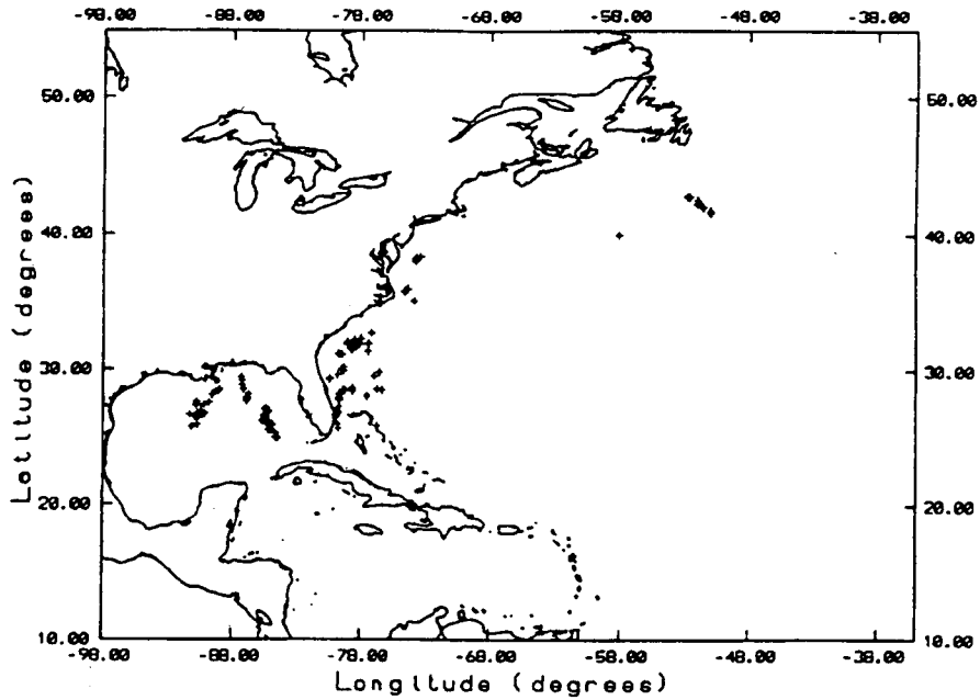
Figure 2 Location of sets from 31 pelagic longline trips observed during 1992.
