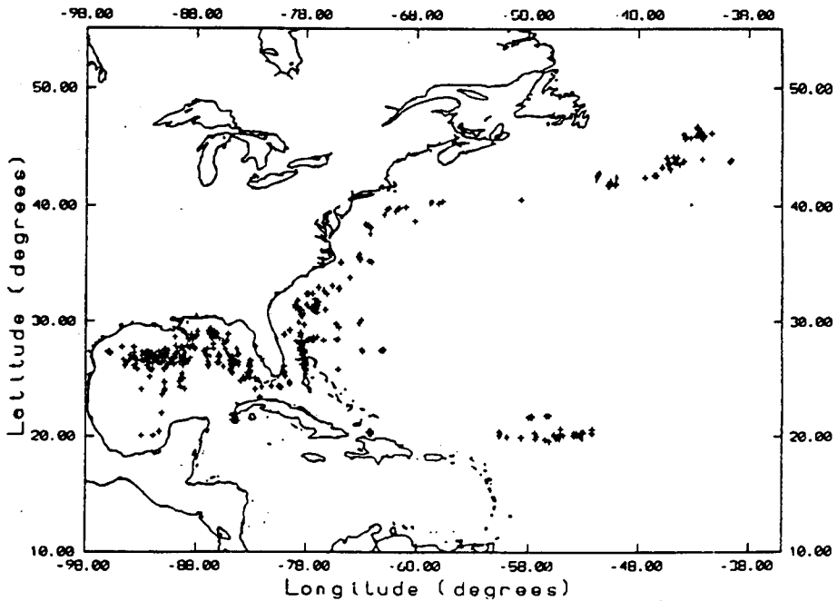
Figure 3 Location of sets from 75 pelagic longline trips observed during 1993.
