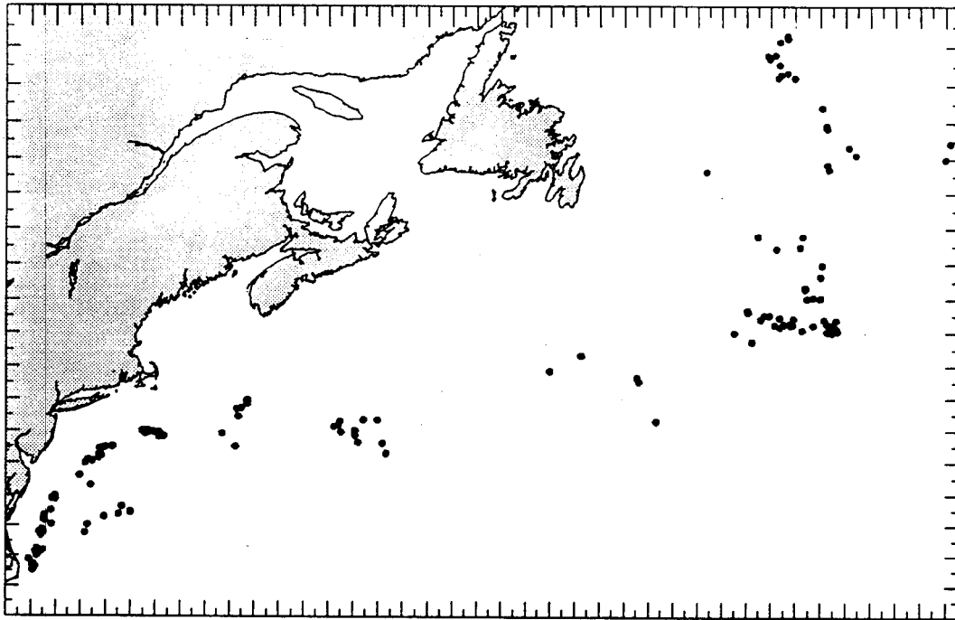
Figure 3. Location of NEFSC observed pelagic longline hauls from 1992.
