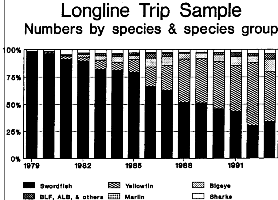
Figure 2. Proportional species composition (weight) for sampled U.S. Atlantic longline trips sampled between 1978 and 1993.
