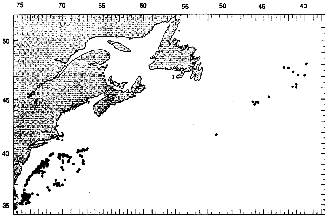
Figure 5. Location of NEFSC observed pelagic longline hauls from 1993.
