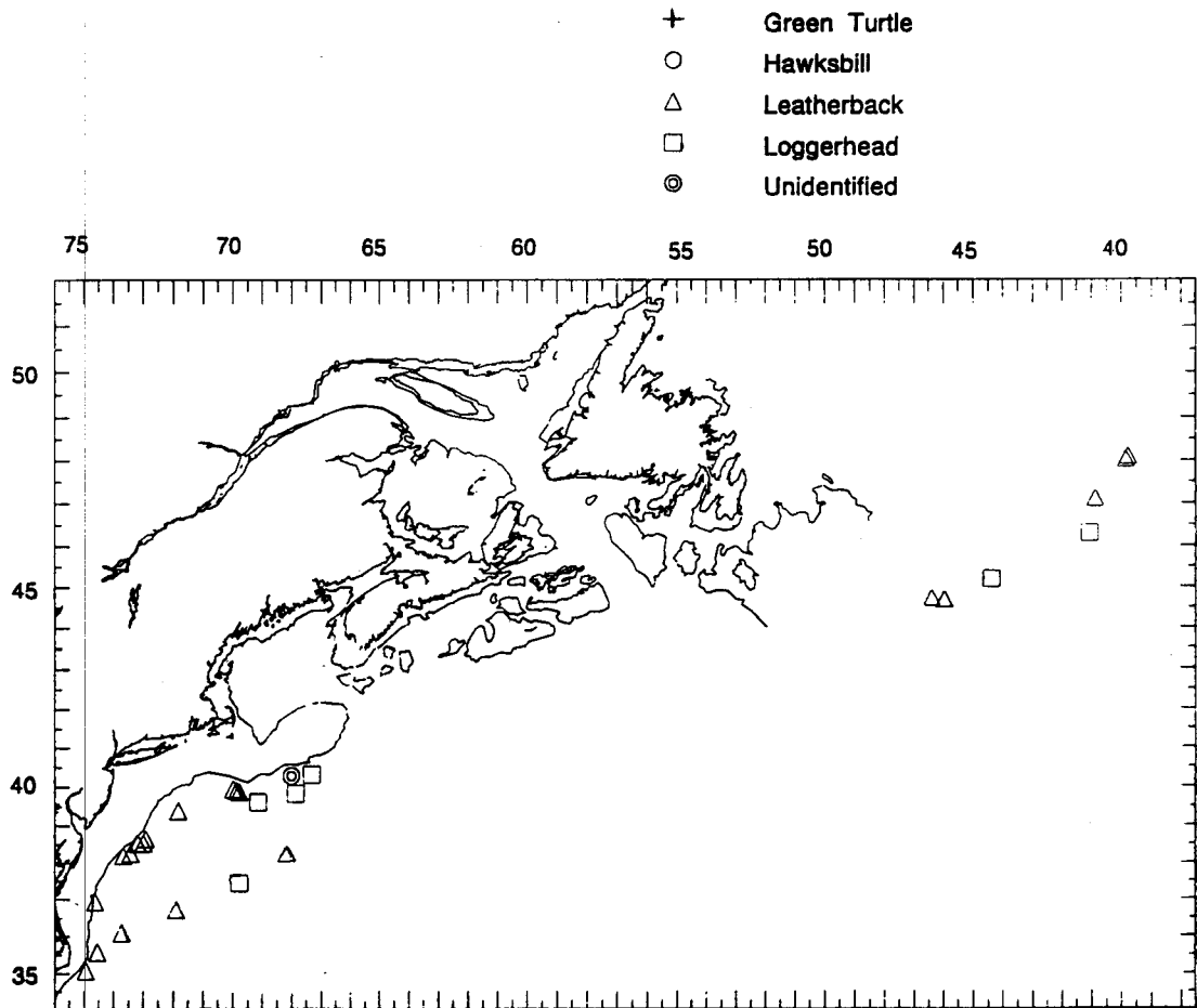
Figure 6. Sea turtle interactions by species from NEFSC observed pelagic longline trips in 1993.
