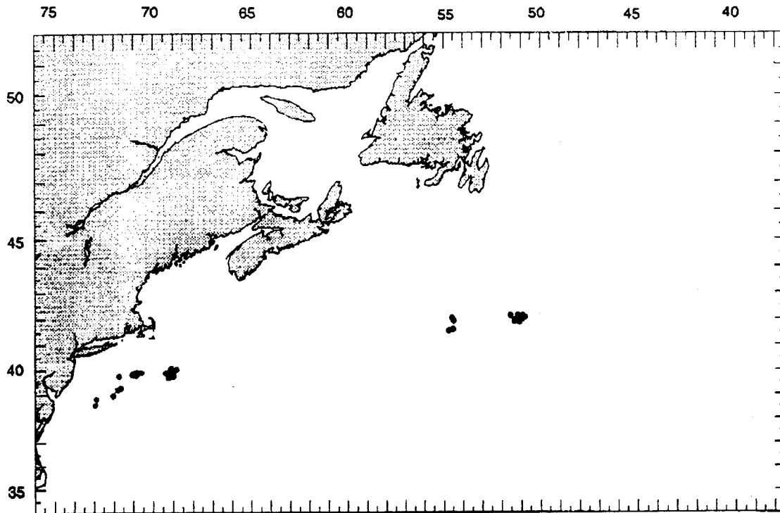
Figure 1. Location of NEFSC observed pelagic longline hauls from 1991.
