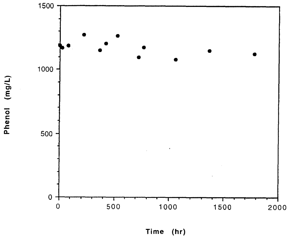
FIGURE 6 Phenol Concentrations During PVT-1
