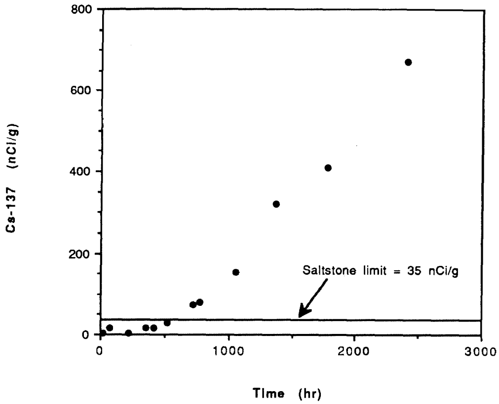
Figure 1. Cs-137 Concentration During PVT-1
