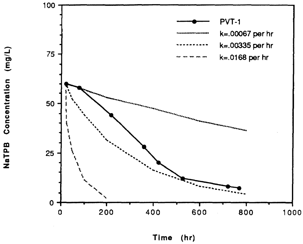
Figure 2. NaTPB Concentration During PVT-1
