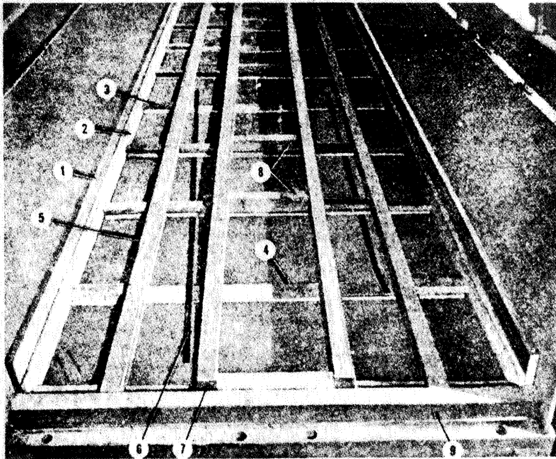
1. Side-wall reinforcement, 2" x 12" on edge 2. Sockwa plate, 1" x 5" on edge 3. Spacers, 2" x 4", nailed to sleepers 4. Sleepers, 1" x 6", nailed to floor 5. Intermediate stiffers, 8" x 4" 6. Floor and aft strapping, 1 1/2" x 6,000' strength and positioned under sleepers 7. Center brace, 4" x 4" 8. Center brace, 6" x 4" 9. End cross plate, 4" x 4"
