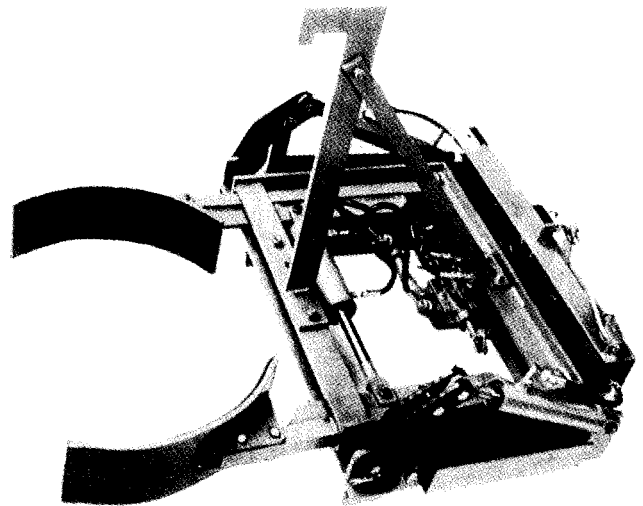
Figure 4-49 Drum-handling adaptor
