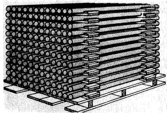
Figure 4-76. Binder block dunnage used in the storage of pipe
