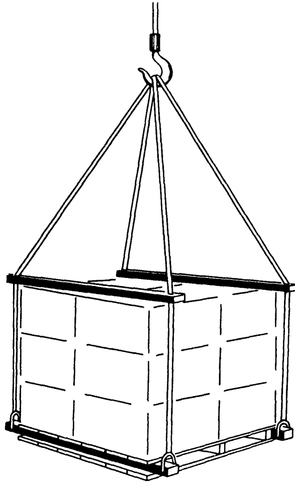
Figure 4-61 Pallet sling.
