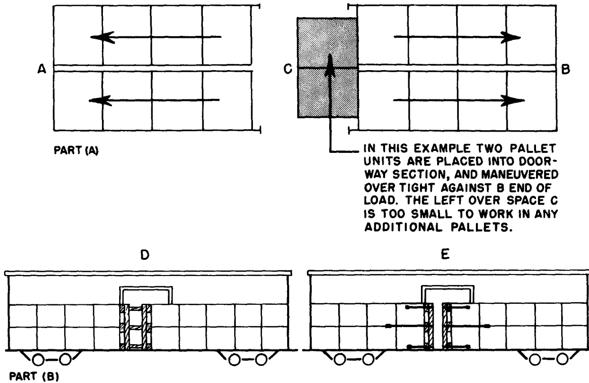
Figure 3-22 Palletized loads
