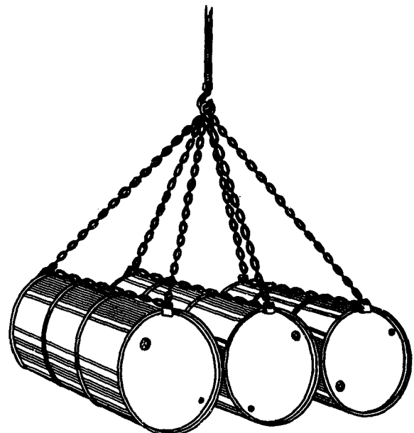
Figure 4-46 Drum-handling sling
