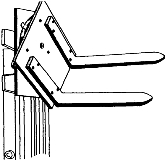
Figure 4-56 Revolving carriage.
