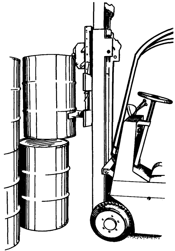
Figure 4-48 Drum-handling attachment single-drum type, vertical carry.
