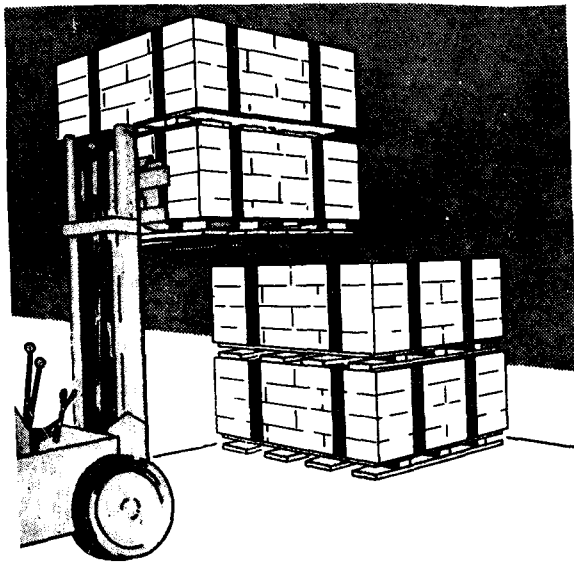
Figure 4-119. A double pallet load must be tiered with an overhang of no more than 2 inches in any direction
