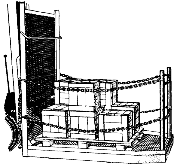
Figure 4-58 Safety pallet.
