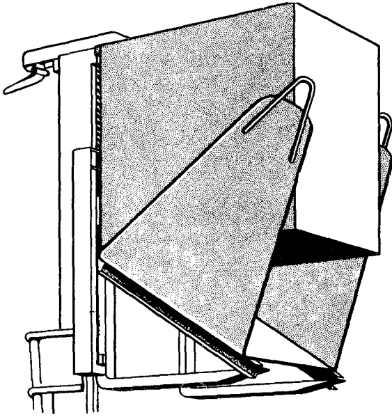
Figure 4-50 Bottom-dumping hopper
