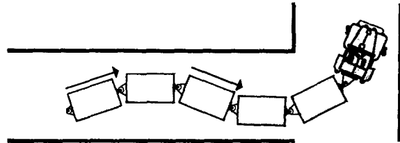
Figure 4-124 Right way to turn corners with a tractor-trailer train.
