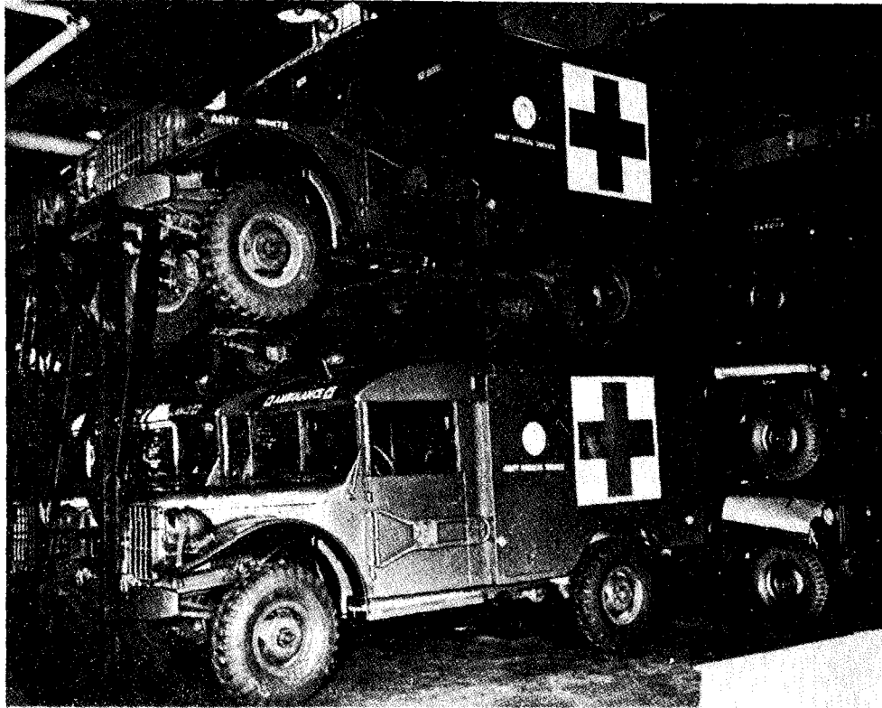
Figure 5-20 Suspension-type racks for stacking vehicles in storage
