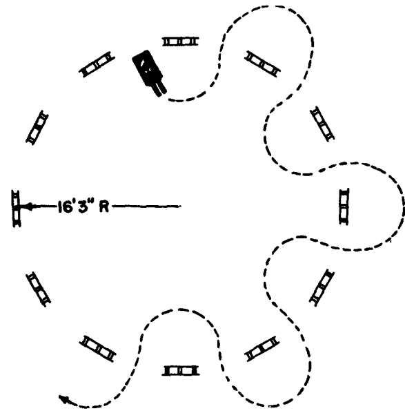
Figure 4-126. In this operational test, the trainee weaves in and out between pallets in a circle having 16-foot, 3-inch radius.
