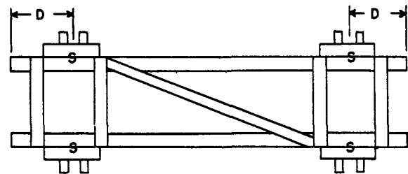
NOTE: DISTANCE "D" NOT MORE THAN 30". "S" REPRESENTS SNUBBING DEVICES.
