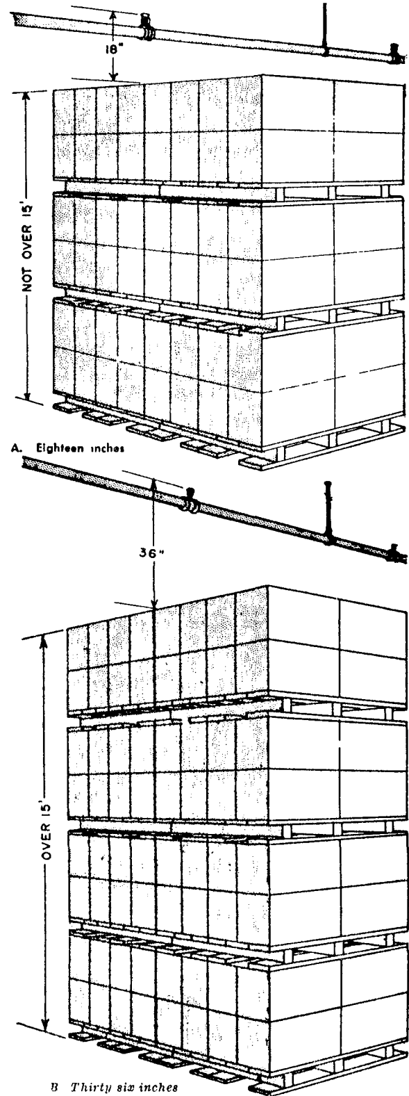
Figure 6-1 Overhead stack clearance at sprinkler head
