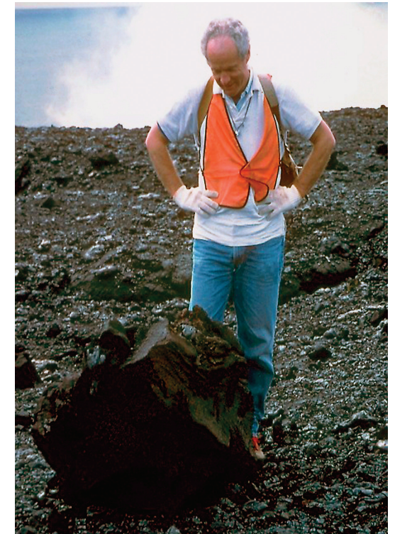
Above: Aerial view in November 1992 of a lava delta, only four days old, formed at Kamoamoa Bay as flows from Pu‘u ‘Ō‘ō entered the sea, producing steam clouds and extending the shoreline 600 feet seaward. A much larger delta was active at East Lae‘apuki during 2005–2007 (see text). Right: A scientist looks at a large block of solidified lava that was hurled more than 50 feet inland during a littoral explosion. The blast was triggered by collapse of an active lava bench in 1989. (USGS photographs by Christina Heliker.)
