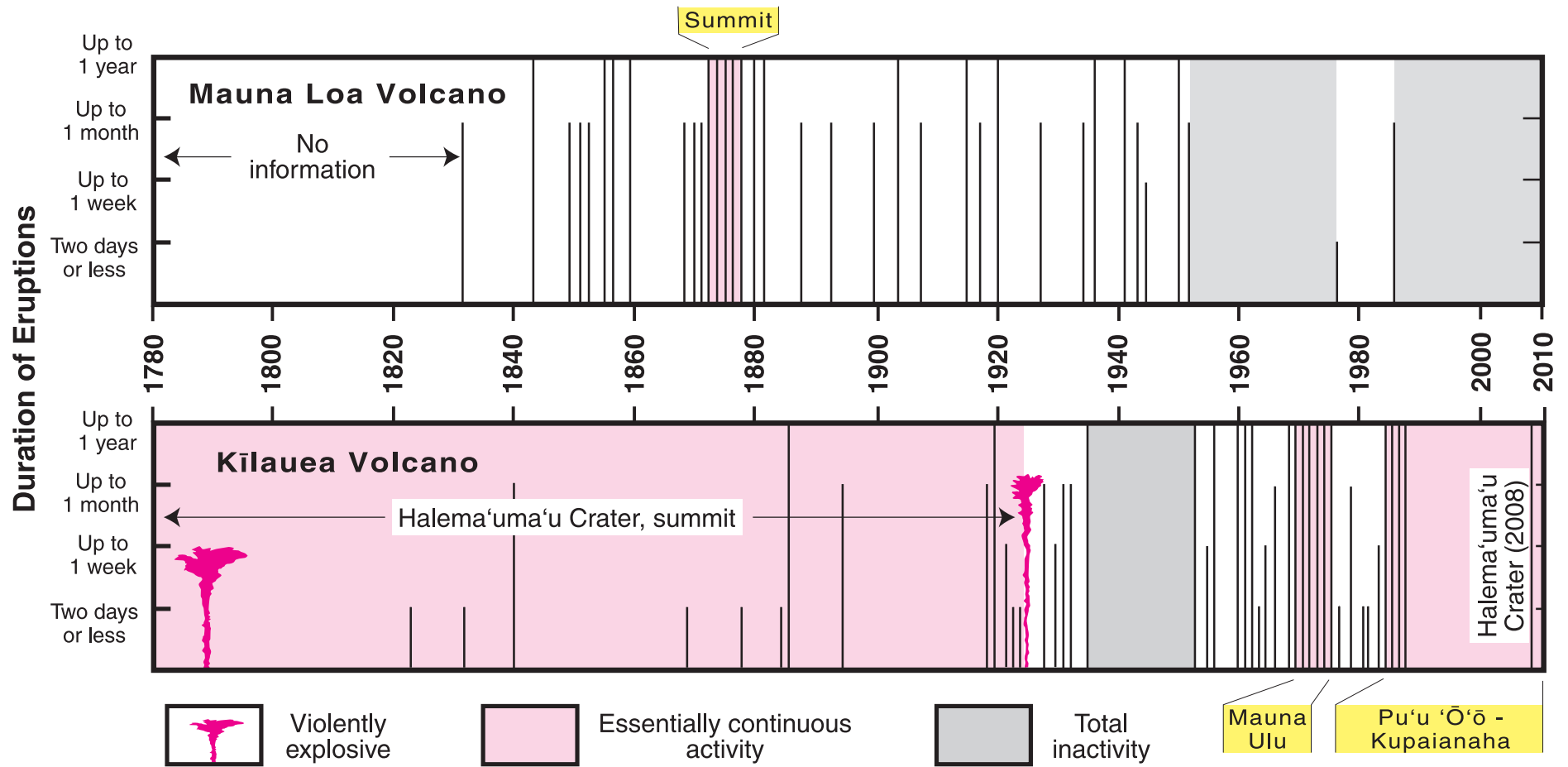
Graph summarizing the eruptions of Mauna Loa and Kilauea Volcanoes during the past 200 years. The Pu'u 'O'o- Kupaianaha eruption has continued into the 21st century. Information is sketchy for eruptions before 1823, when the first missionaries arrived on the Island of Hawai'i. The total duration of eruptive activity in a given year, shown by the length of the vertical bar, may be for a single eruption or a combination of several separate eruptions.
