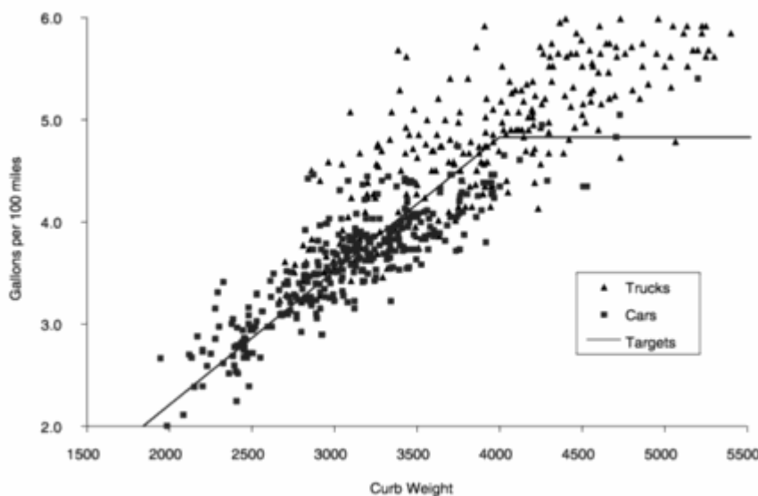
Figure 2: Illustration of the fuel economy function under the NAS alternative attribute system example (NAS report, p. 109).
