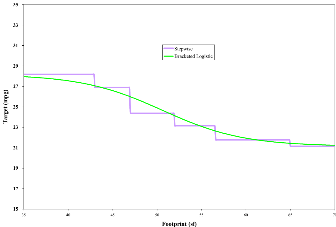
Figure 13: Final “optimized” curve compared to the proposed step function
