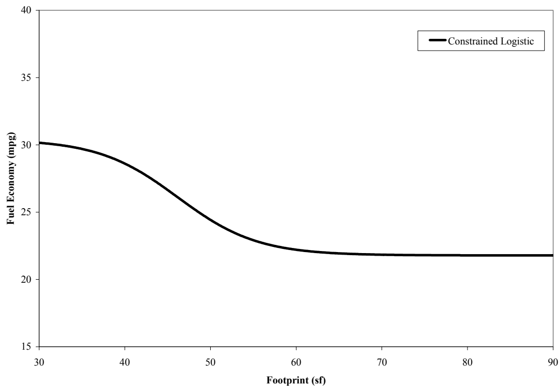
Figure 8: Constrained logistic function
