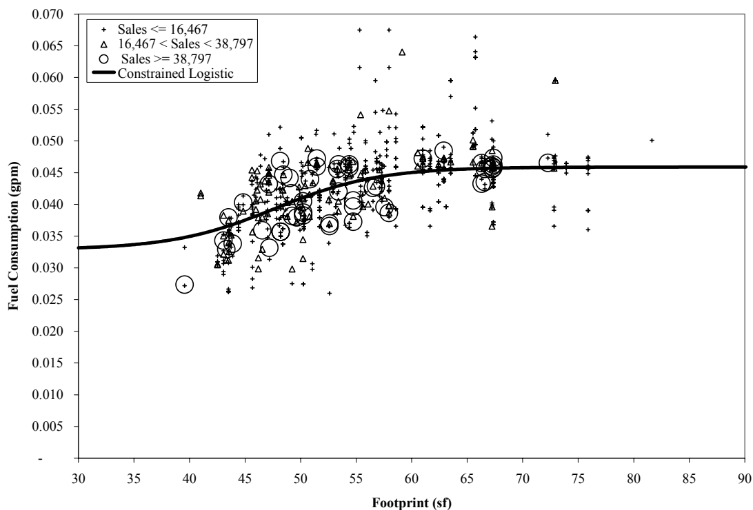
Figure 7: Constrained logistic function fit through sales weighted “socially optimized” light truck fleet (gpm as a function of footprint)
