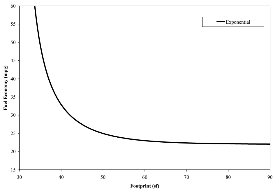
Figure 5B: Exponential function fit through sales weighted “socially optimized” light truck fleet (mpg as a function of footprint)
