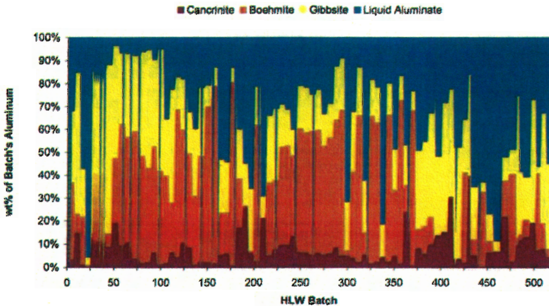
Figure 2 Partitioning of Aluminum per TFCOUP 6 Batch (Figure 4.1-3 of 2008 WTP Tank Utilization Assessment)
