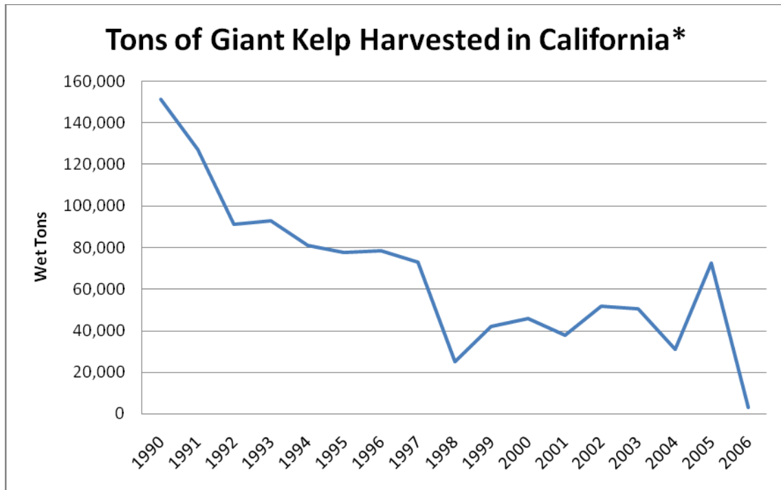
Figure 2.6. Tons of Giant Kelp Harvested in California (NMFS Southwest Regional Office 2008)
