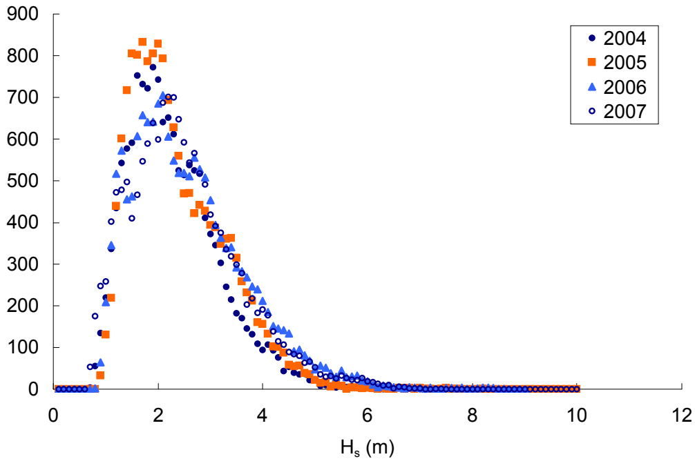
Figure 3.3. The distribution of significant wave height H_s for the years 2004 to 2007 at the CDIP Pt Reyes Buoy.
