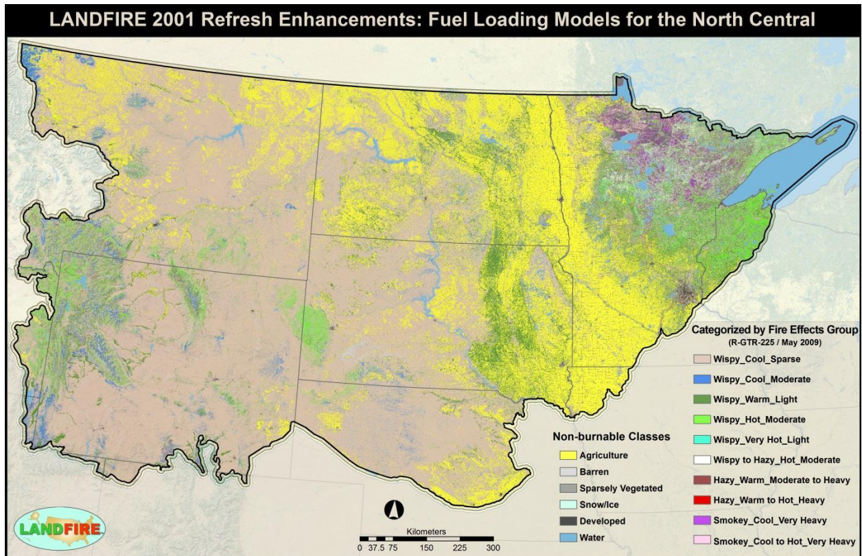
Figure 14 – LF 2001 Fuel Loading Models for the NC GeoArea. FLM categories are from Rocky Mountain Research Station General Technical Report 225.
