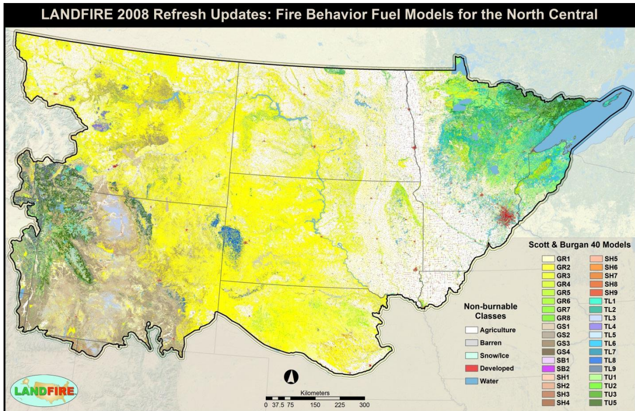
Figure 13 – LF 2008 Fire Behavior Fuel Model 40 for the NC GeoArea.
