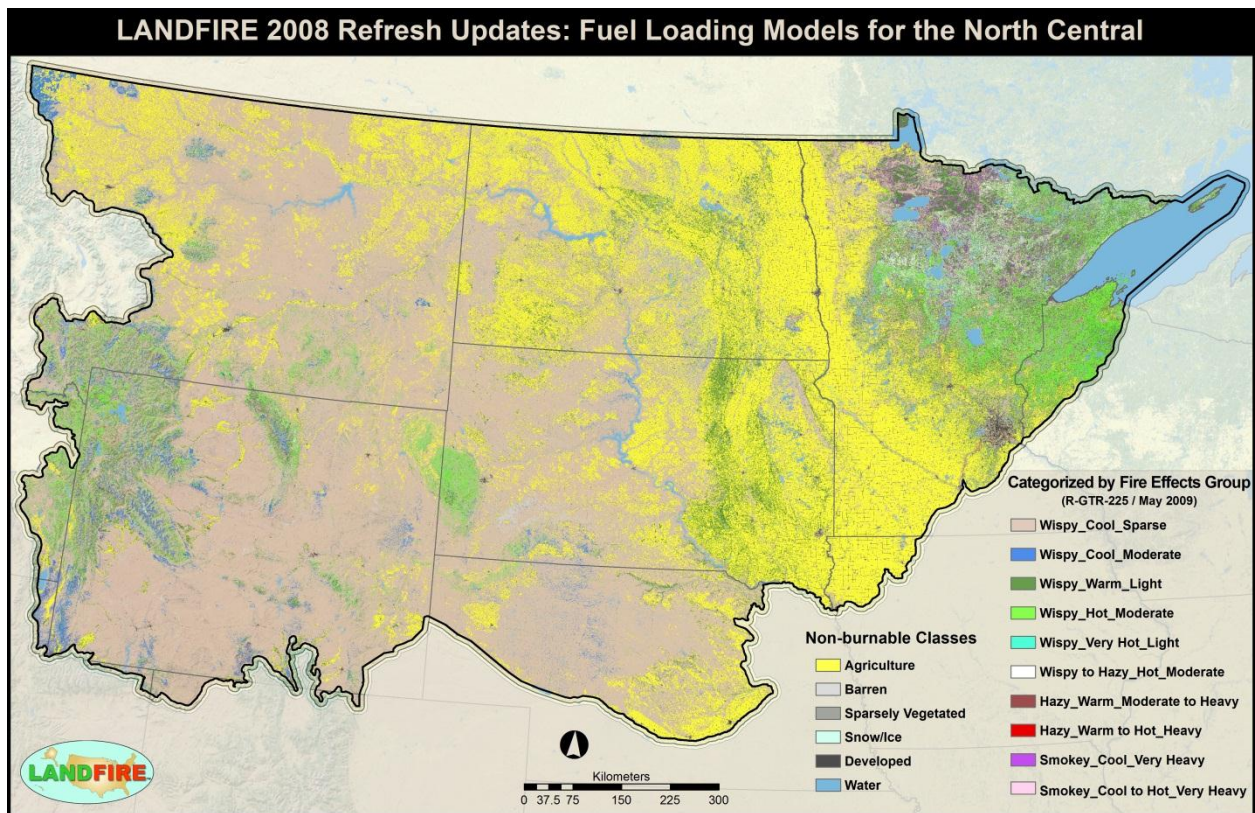
Figure 15 – LF 2008 Fuel Loading Models for the NC GeoArea. Categories are from the Rocky Mountain Research Station General Technical Report 225.
