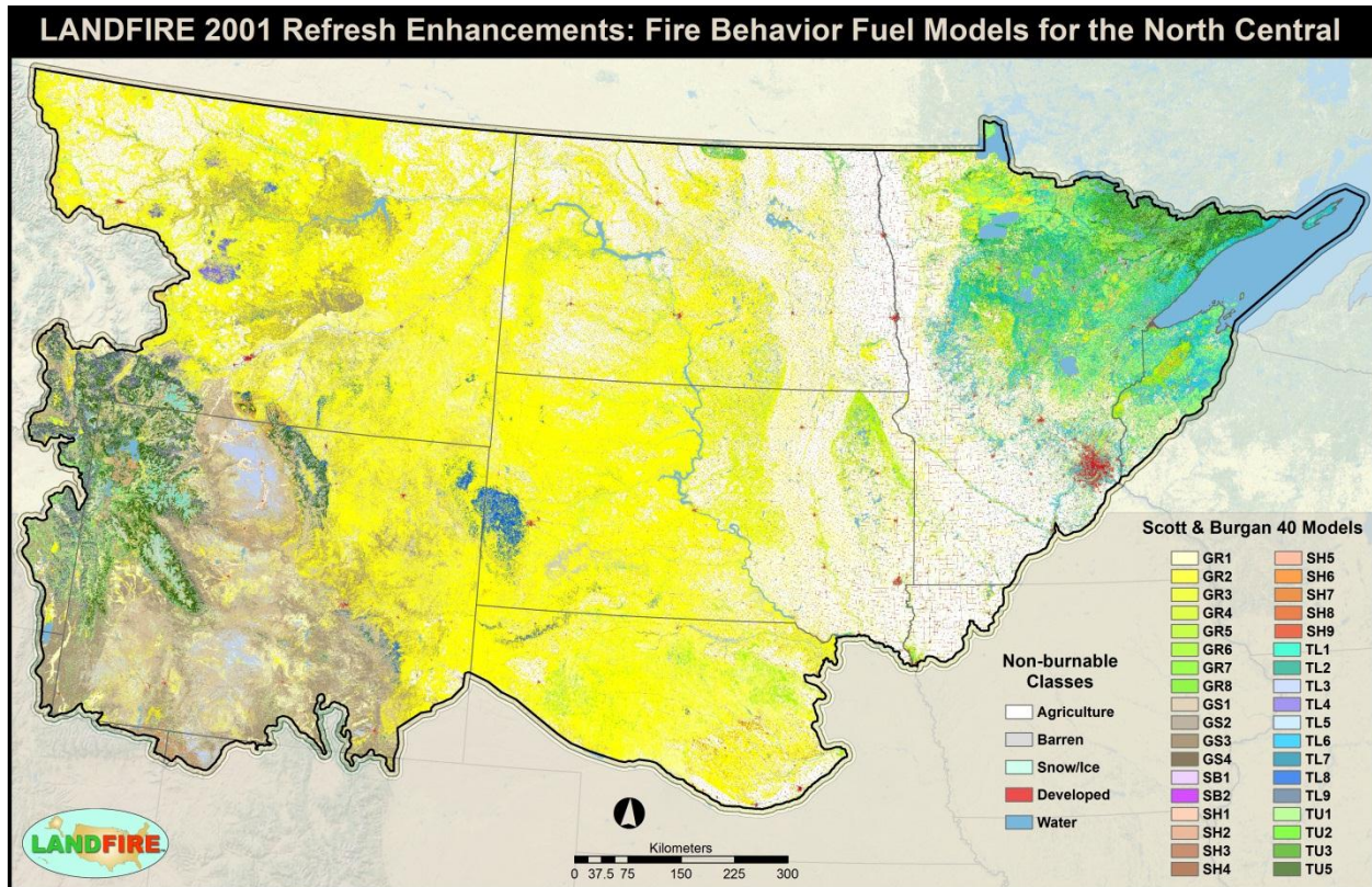
Figure 12 – LF 2001 Fire Behavior Fuel Model 40 for the NC GeoArea
