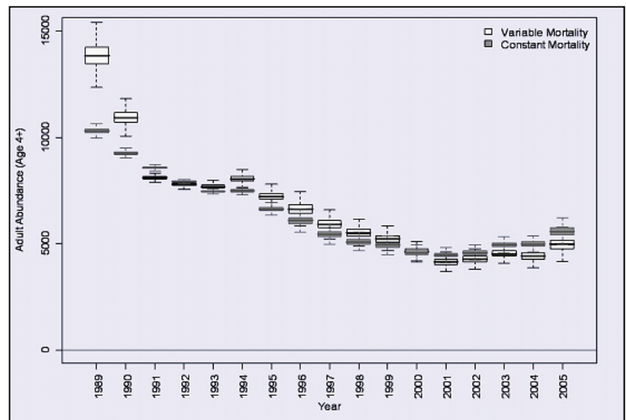
ASMR models of GC adult (4+ yrs.) HBC population through 2005. Source Data: U.S. Geological Survey
