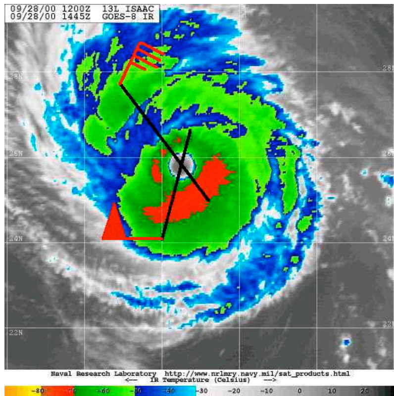
Plate 5: An idealized representation for finding the center of a tropical cyclone based upon peripheral wind observations. Two ship observations (indicated by the red wind barbs) roughly indicate the tropical cyclone center (where the two black lines cross) assuming cyclonic flow with a 20^\circ inflow angle.
