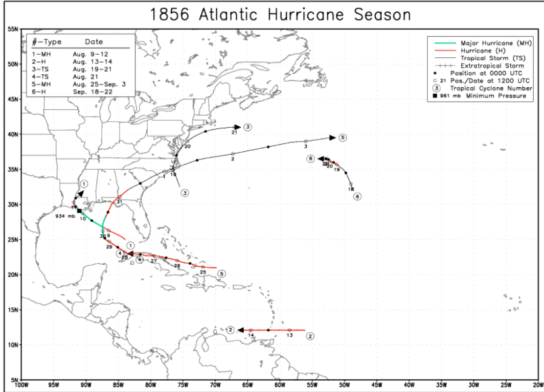
Plate 4 Reconstructed Atlantic tropical cyclone tracks and intensities for 1856.
