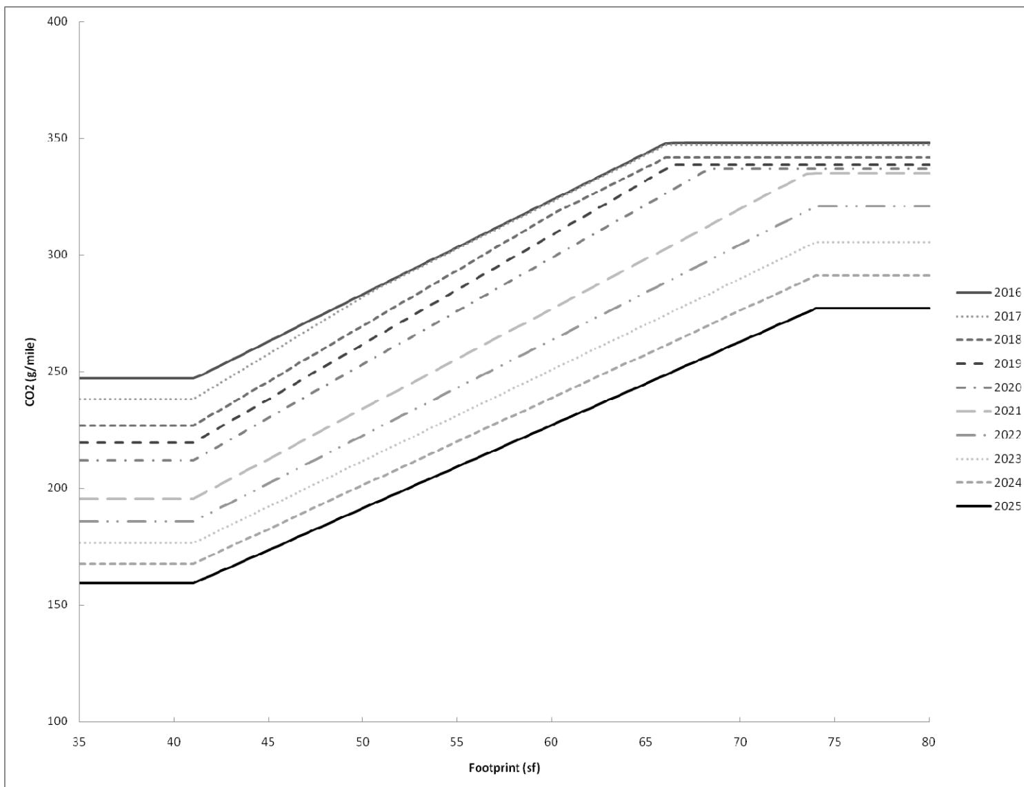
Figure III-2 – Truck Curves
