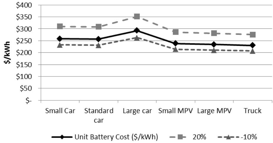
PHEV40 Battery system DMC Range (MY2021)
