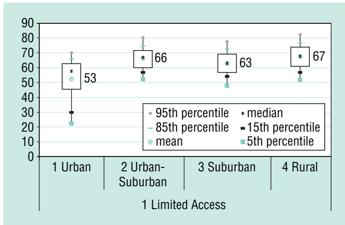
Figure 2. Travel Speeds (in MPH) on Limited Access Roads by Urbanicity
