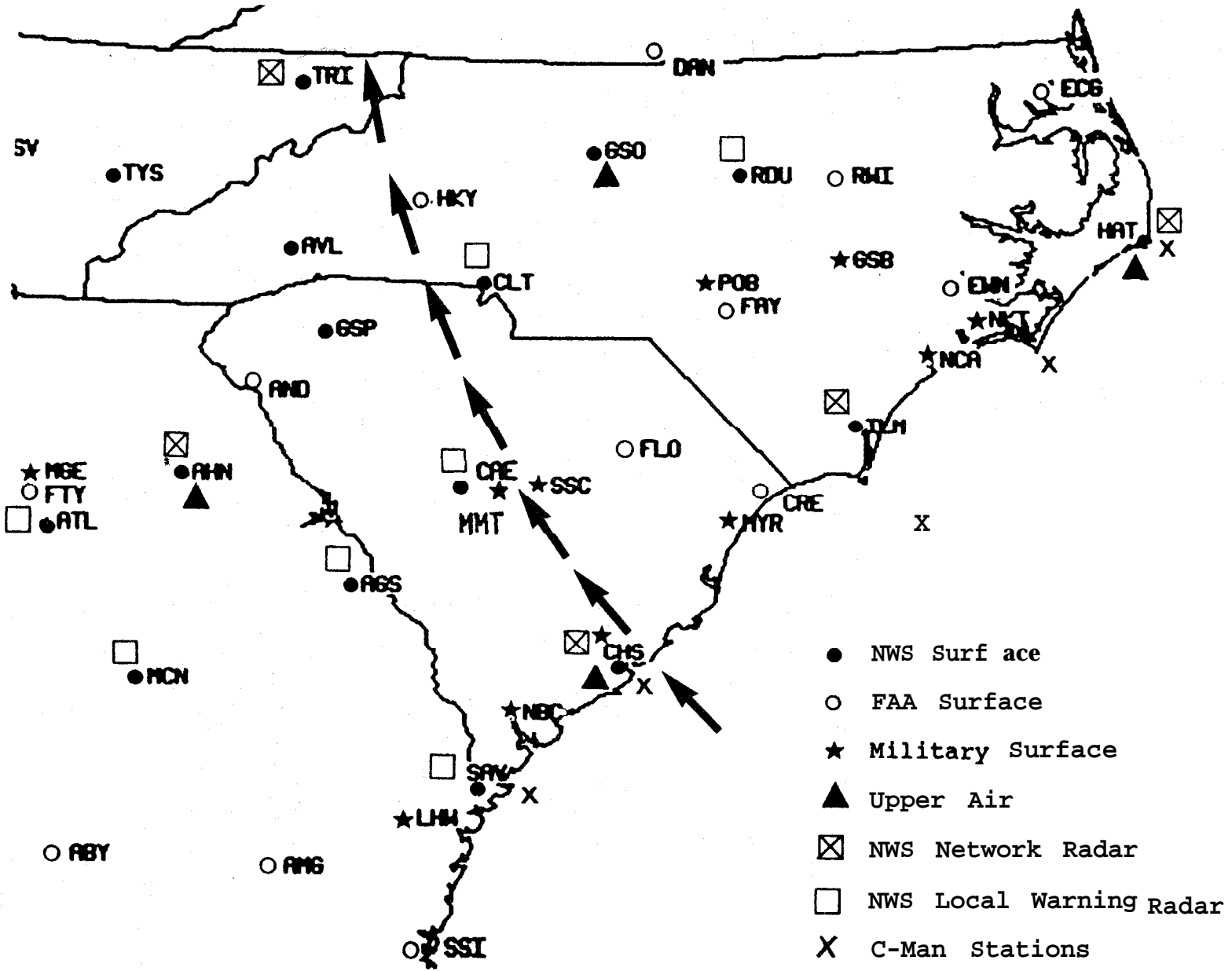
Figure 3-1. Locations and types of data reporting stations available to NWS in area affected by Hurricane Hugo. Arrows show the track of the storm center.
