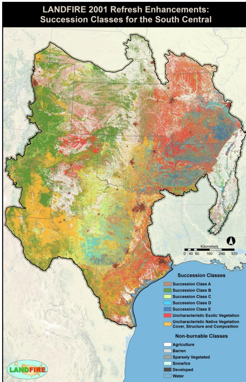
Figure 16 – Map of LF 2001 enhancements of the Succession Classes layer for the SC GeoArea.
