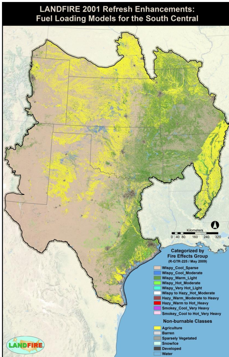
Figure 14 – LF 2001 Fuel Loading Models for the SC GeoArea. FLM categories are from Rocky Mountain Research Station General Technical Report 225.
