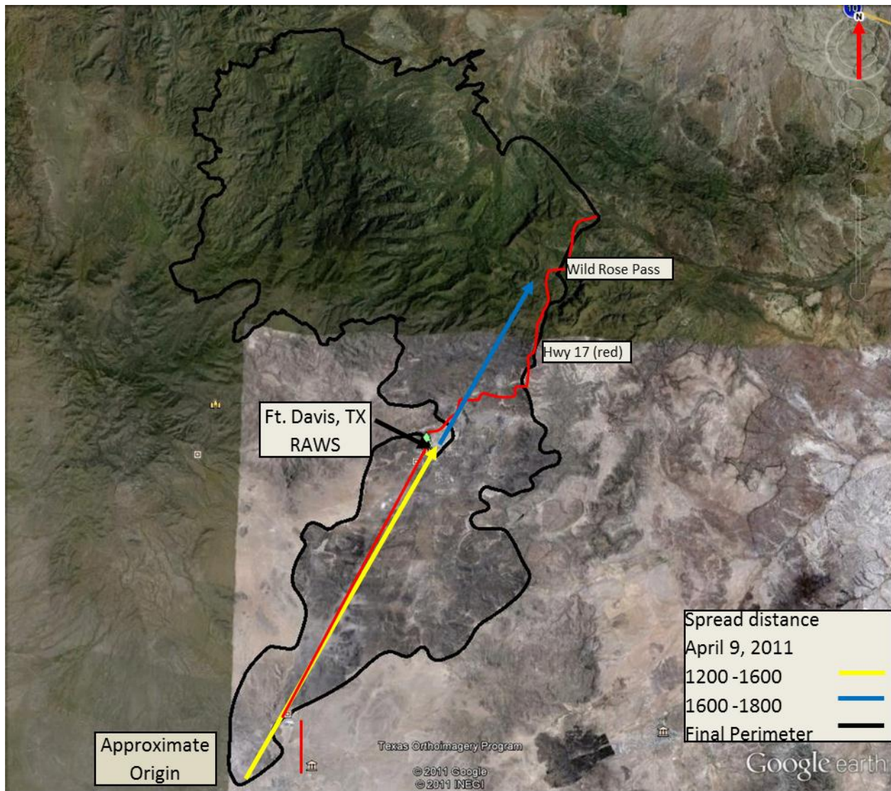
Figure 21 – Rock House Fire Spread up to Simulation Period. The fire perimeter covers an area that extends nearly 43 miles from south to north.
