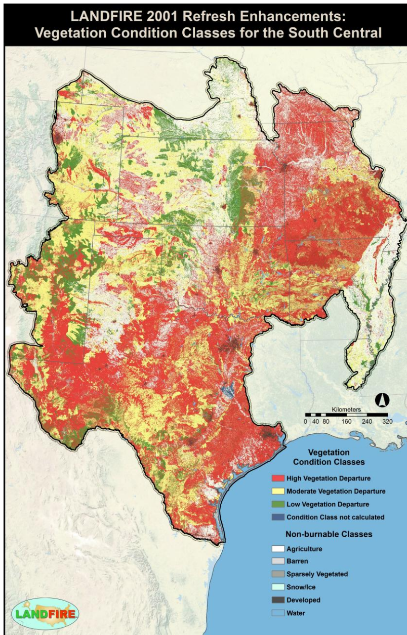
Figure 17 – Map of Vegetation Condition Class for the SC GeoArea from LF 2001 enhancements.
