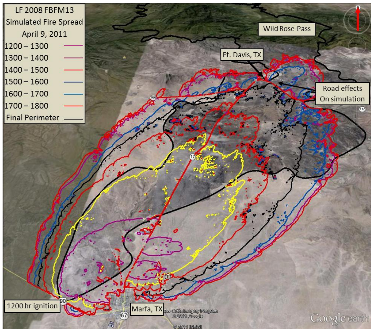
Figure 24 – LF 2008 FBFM13 Fire Simulation Rock House Fire April 9, 2011. The fire perimeter covers an area that extends nearly 43 miles from south to north.
