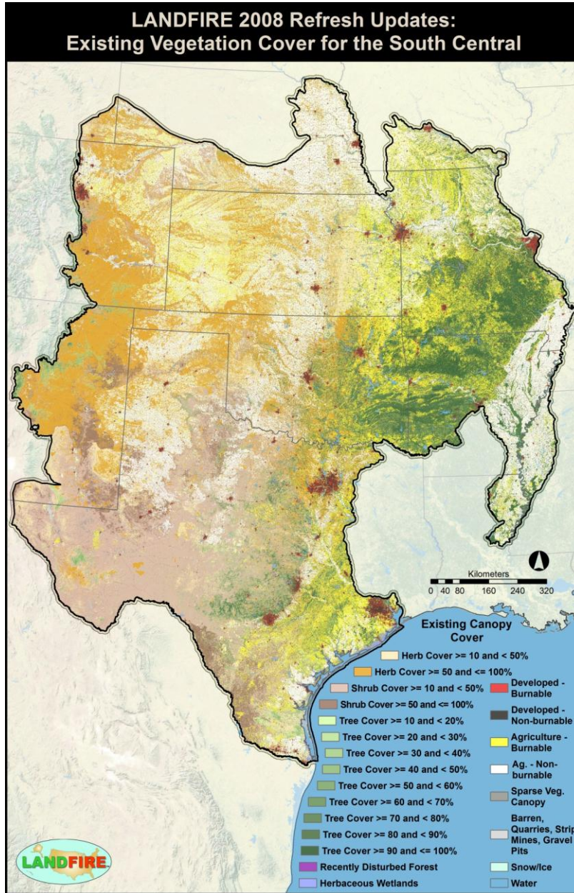
Figure 10 – Map of Existing Vegetation Cover for the SC accounting for vegetation changes with disturbances for 1999 - 2008.
