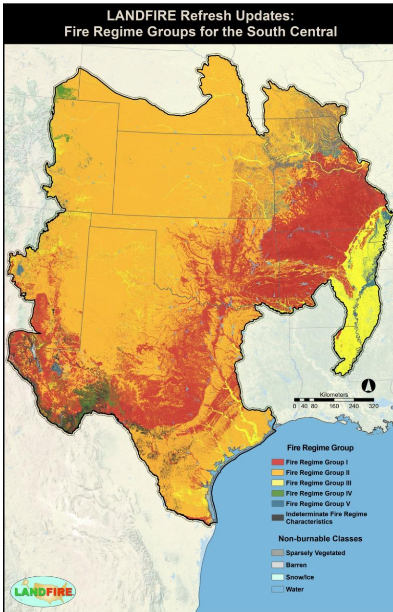
Figure 4 – Map of the SC GeoArea depicting LF Fire Regime Groups in the absence of modern human intervention with possible aboriginal fire use.
