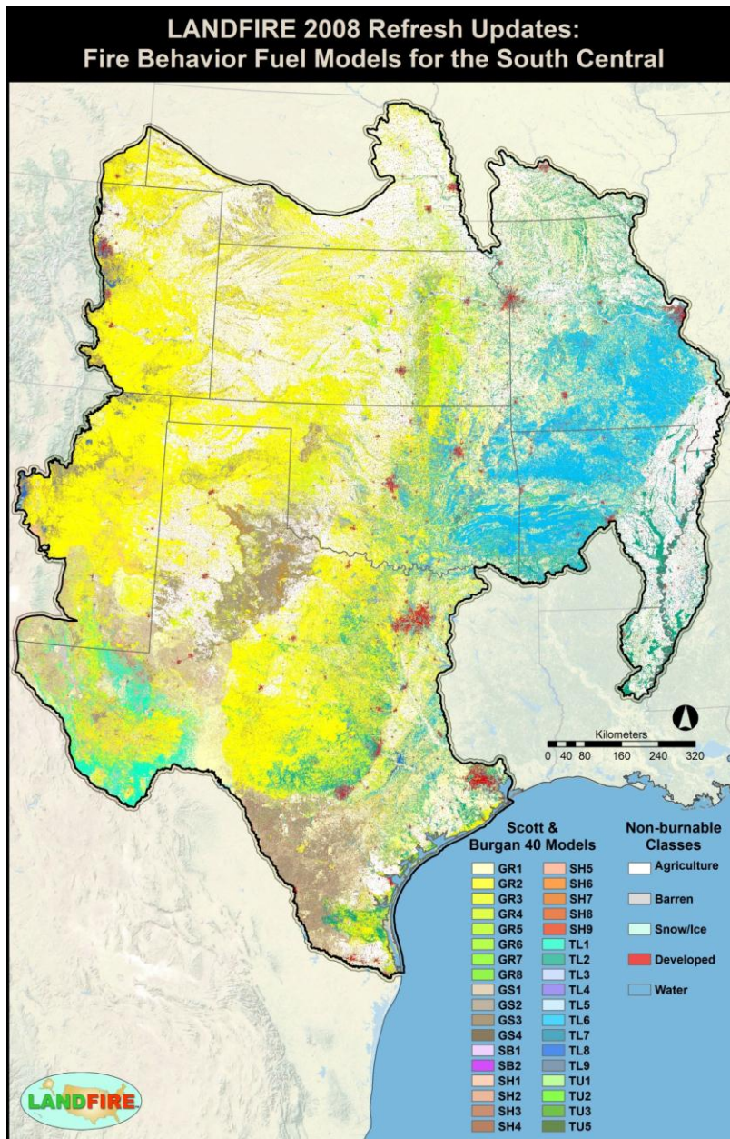
Figure 13 – LF 2008 Fire Behavior Fuel Model 40 for the SC GeoArea.
