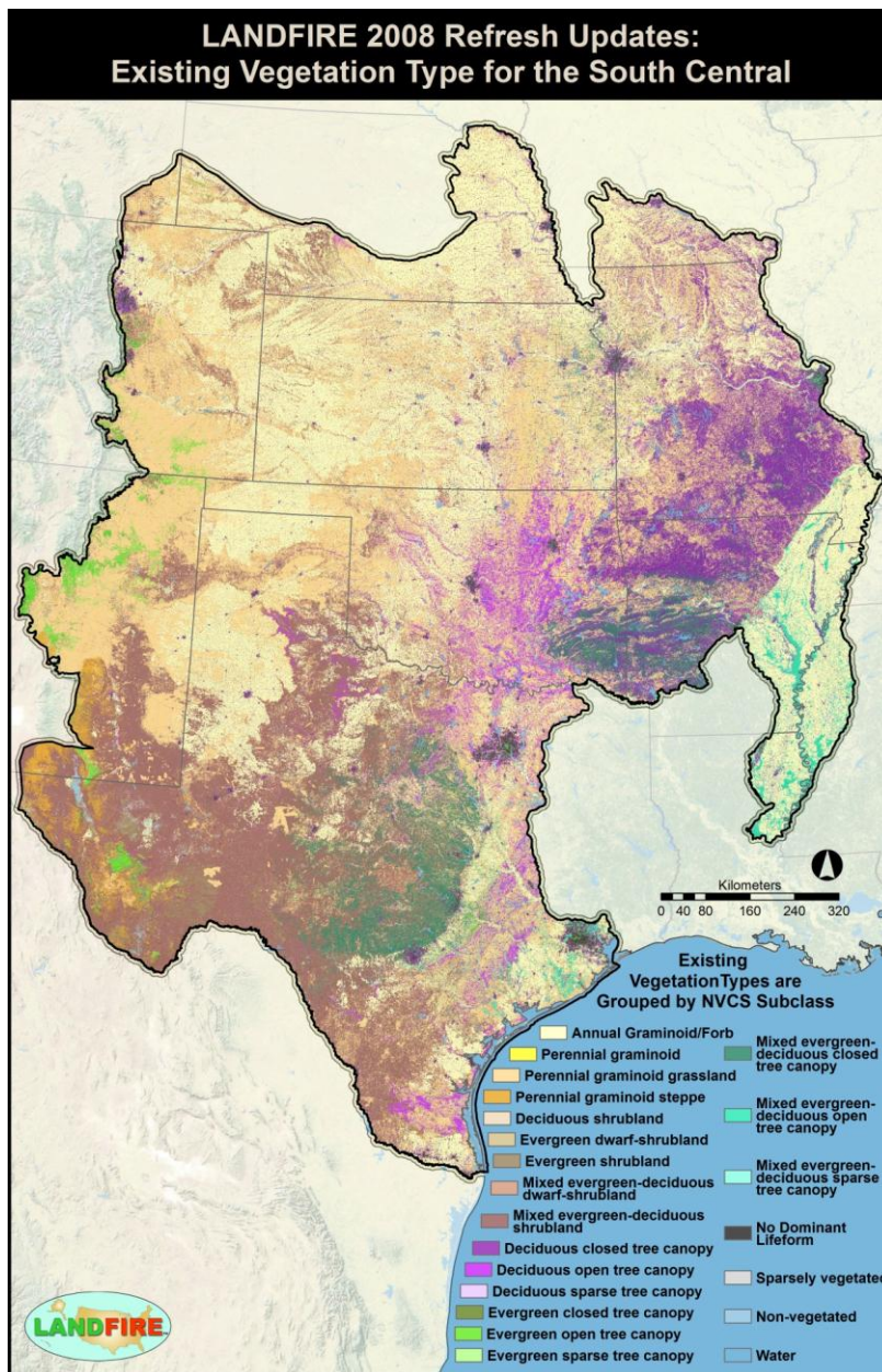
Figure 9 – Map of Existing Vegetation Type layer for the SC GeoArea depicting vegetation changes with disturbances for 1999 - 2008.
