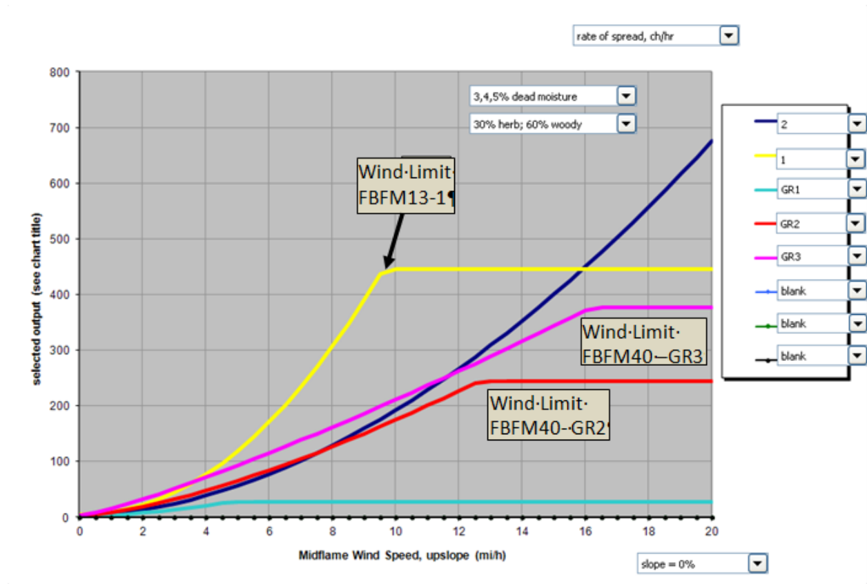
Figure 23 – Comparison of Rates of Spread and Wind Limits between FBFM40 and FBFM13 Models.
