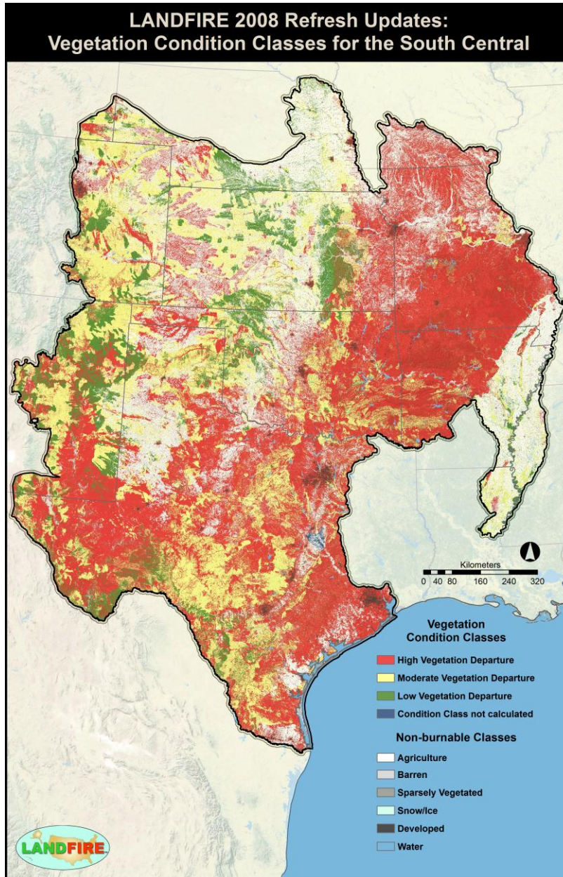
Figure 19 – Map of Vegetation Condition Class for the SC GeoArea from LF 2008 updates.
