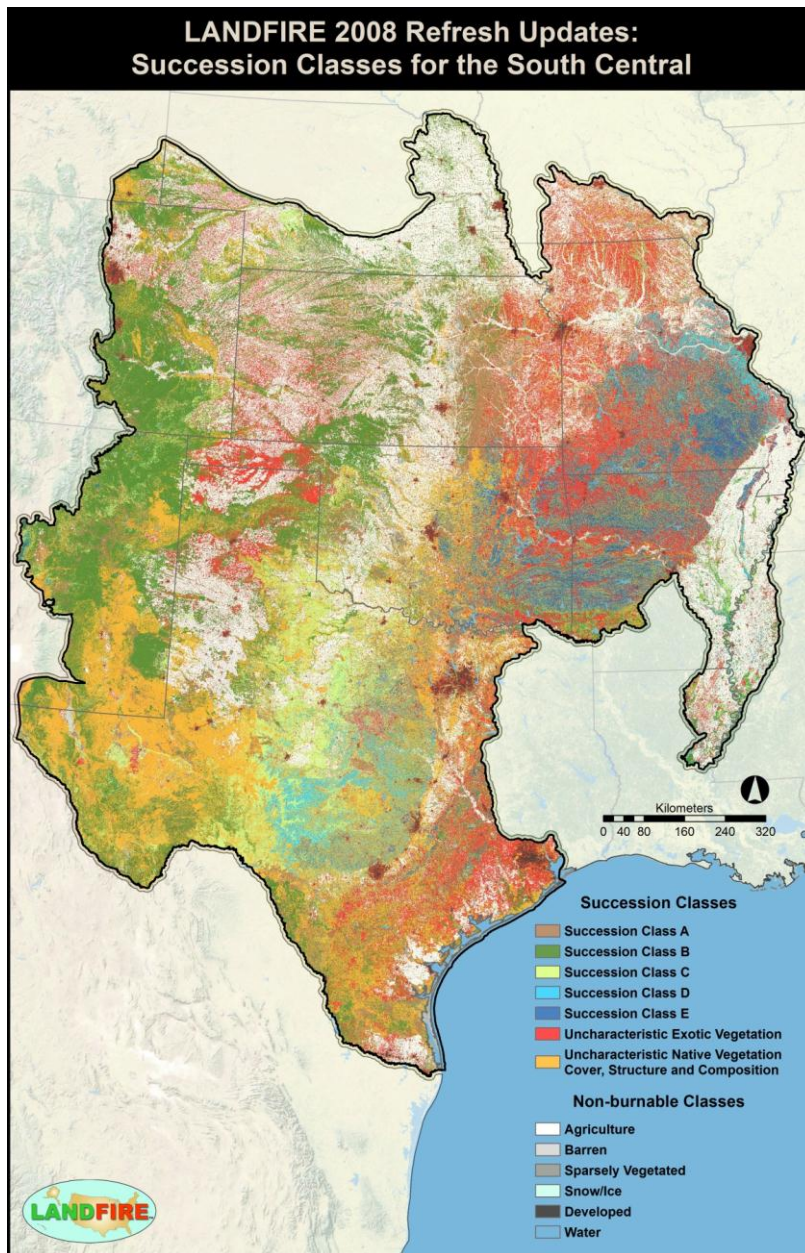
Figure 18 – Map of LF 2008 updates of the Succession Classes layer for the SC GeoArea.
