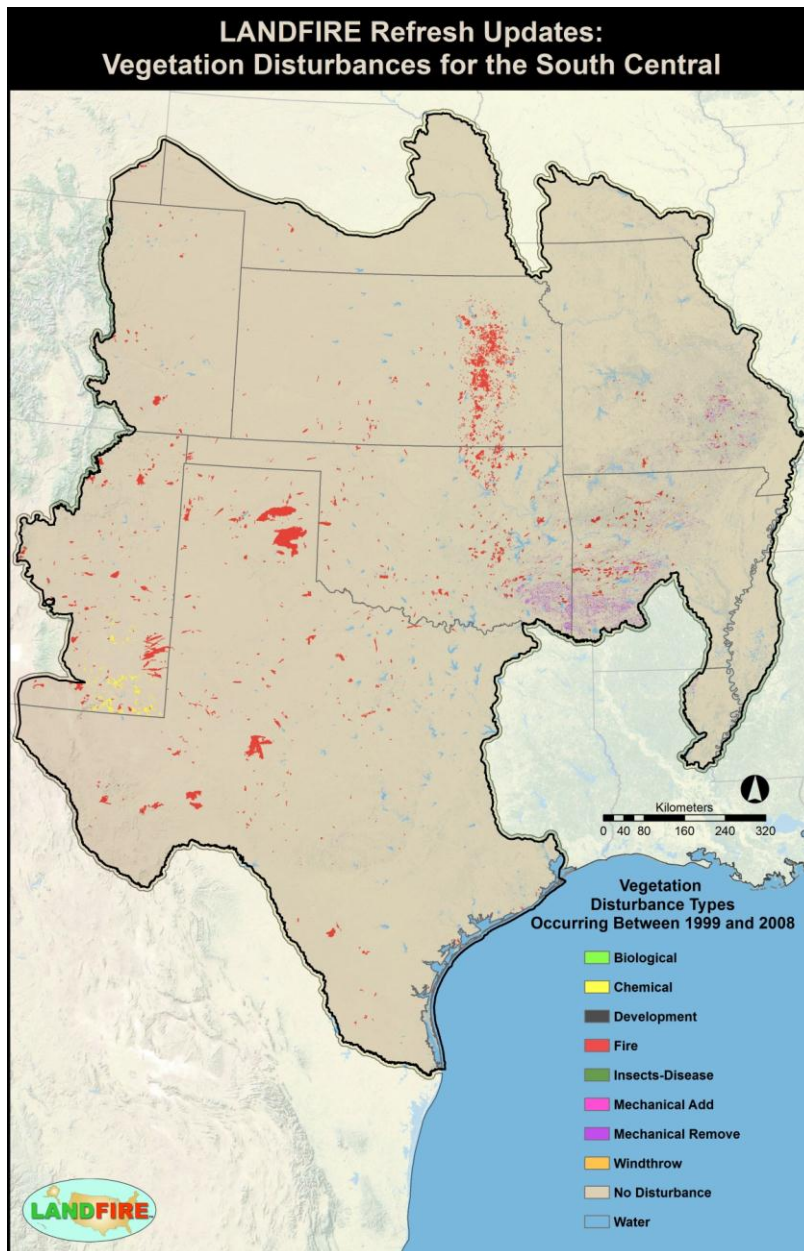
Figure 5 – Map of vegetation disturbance types (fire, mechanical, etc.) mapped for the SC GeoArea from 1999 to 2008.
