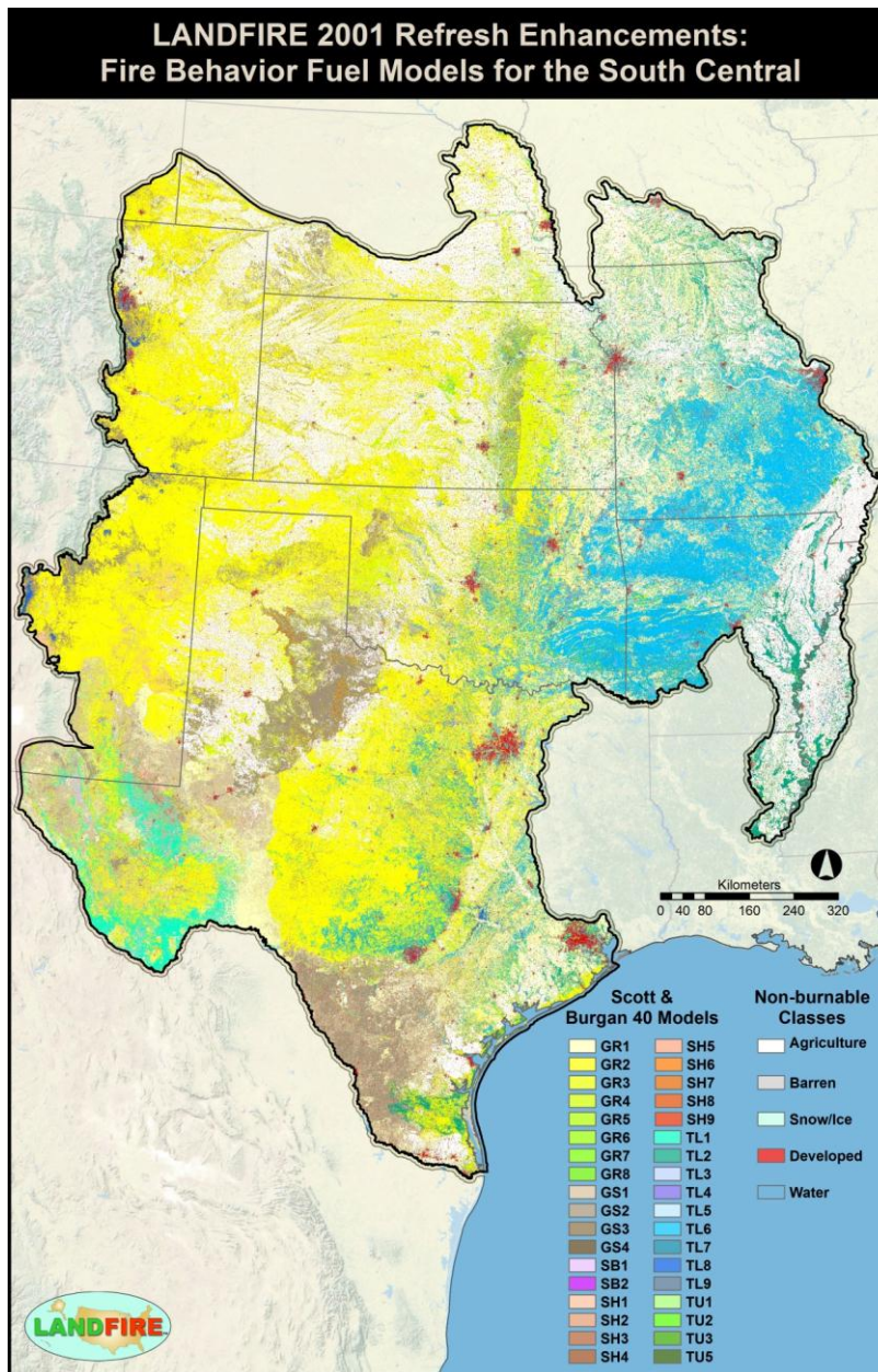
Figure 12 – LF 2001 Fire Behavior Fuel Model 40 for the SC GeoArea
