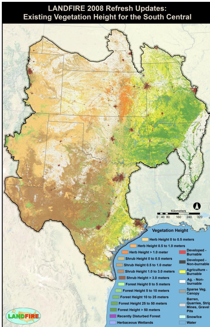
Figure 11 – Map of Existing Vegetation Height for the SC GeoArea accounting for vegetation changes from disturbances for 1999 - 2008.
