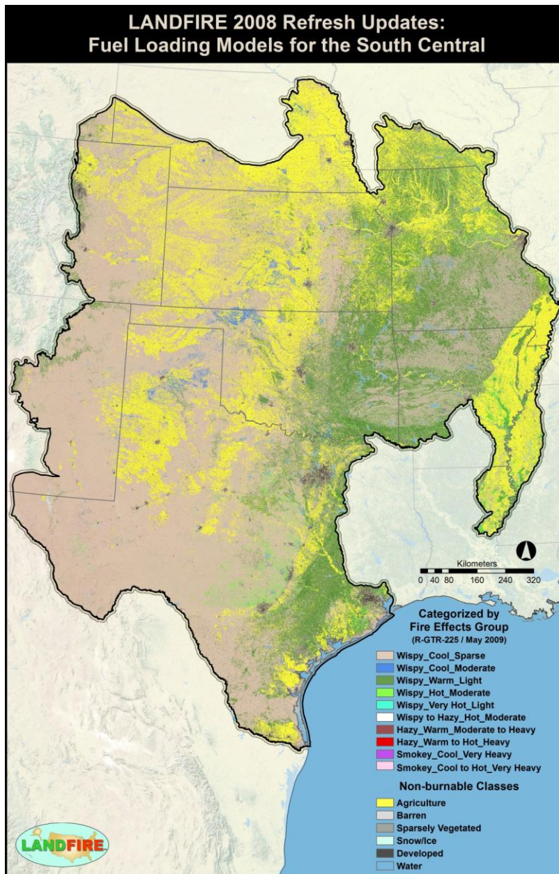
Figure 15 – LF 2008 Fuel Loading Models for the SC GeoArea. Categories are from the Rocky Mountain Research Station General Technical Report 225.
