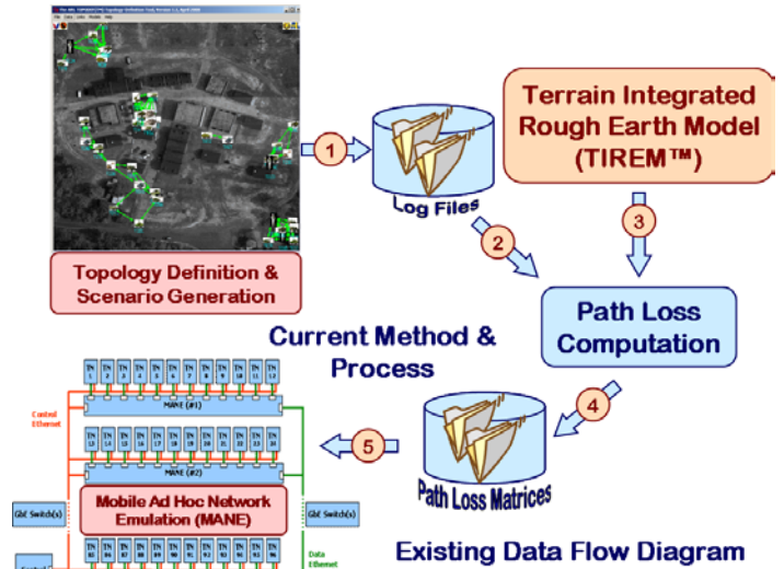
Figure 1. Pre-computation process and the MANE test bed. Executing the MANE software system with the -p option specifies that it should use the pre-computed path-loss matrix file. Conversely, without the specified option, the path-loss matrix is disregarded by the MANE system. Whether the option -p is specified, the MANE system
