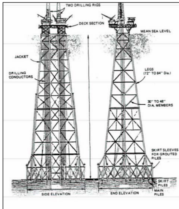
Figure 11.1. Deepwater Platform
