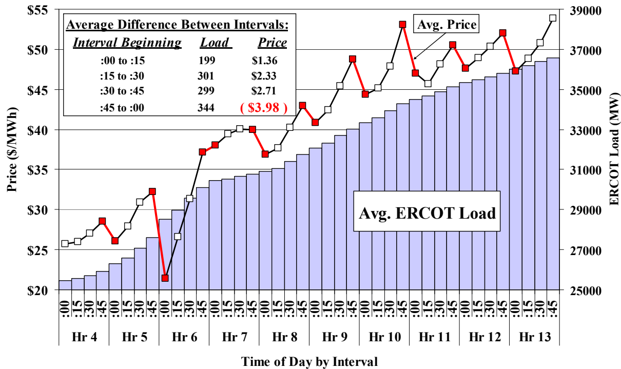
Figure 11: Average Clearing Price and Load by Time of Day Ramping-Up Hours – 2003
