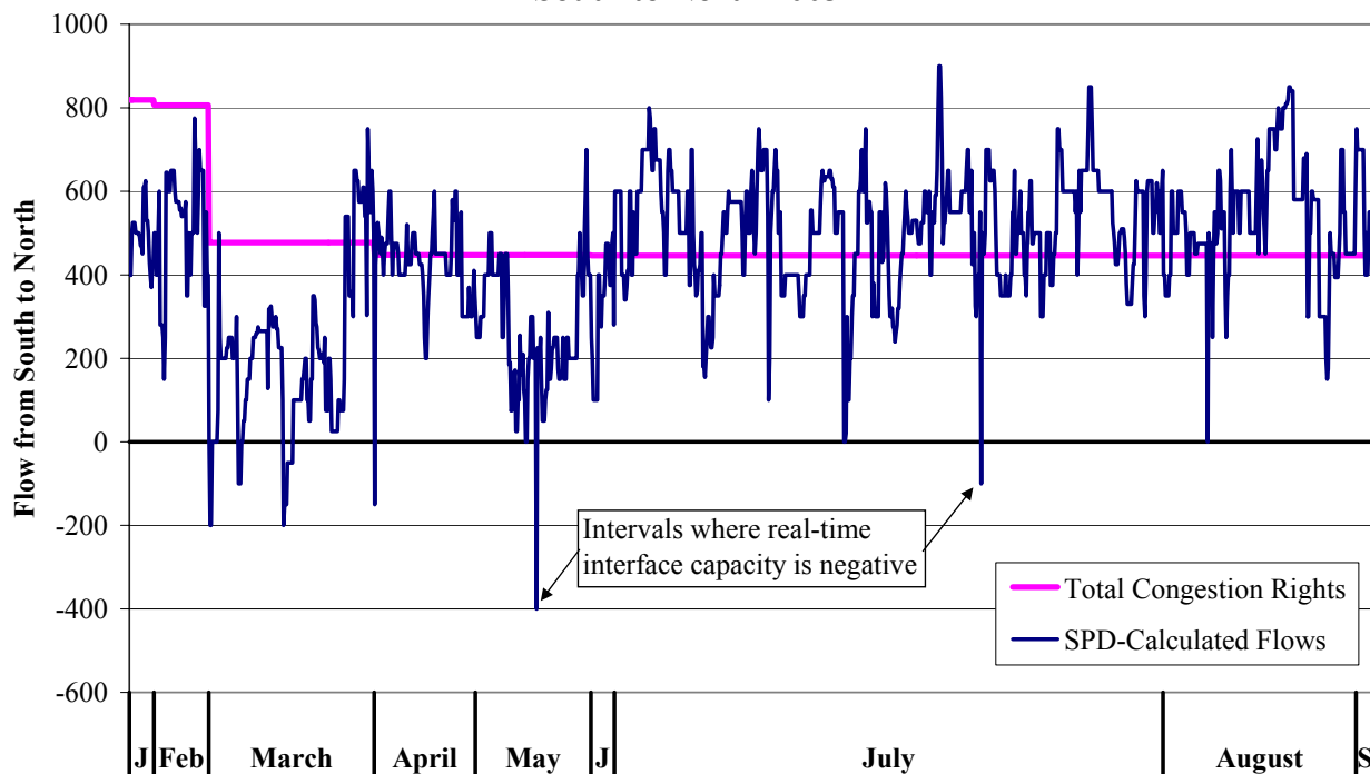
Figure 52: Congestion Rights Allocated vs. SPD Flows during Constrained Intervals South to North 2003
