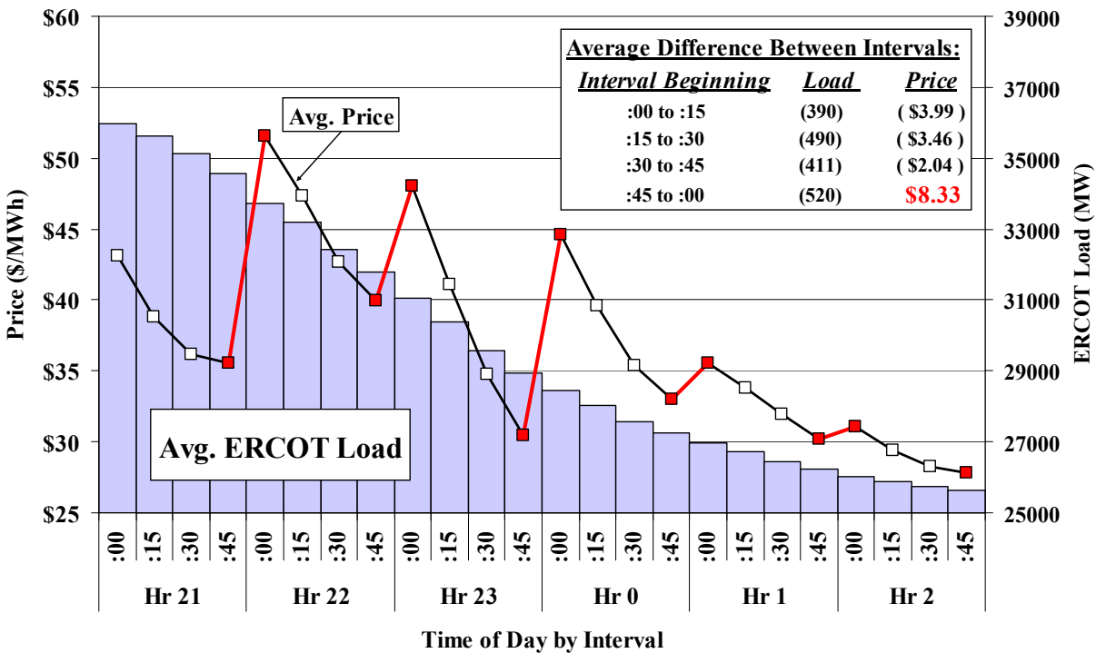
Figure 12: Average Clearing Price and Load by Time of Day Ramping-Down Hours – 2003
