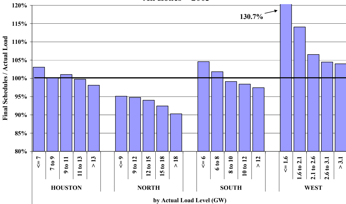
Figure 24: Average Ratio of Final Schedules to Actual Load by Load Level All Zones – 2003
