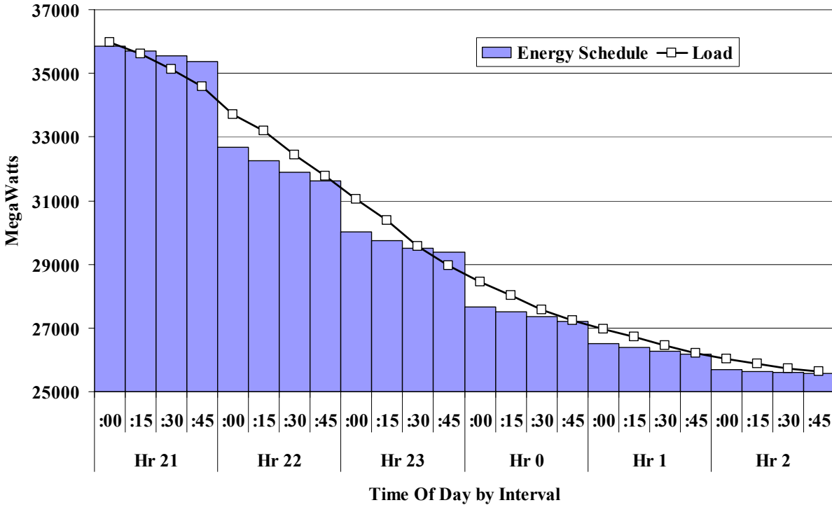
Figure 28: Final Schedules during Ramping-Down Hours 2003
