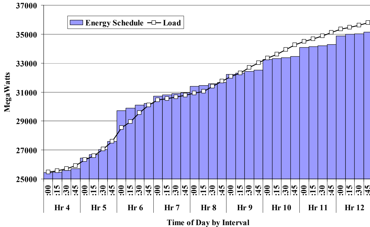
Figure 27: Final Schedules during Ramping-Up Hours 2003
