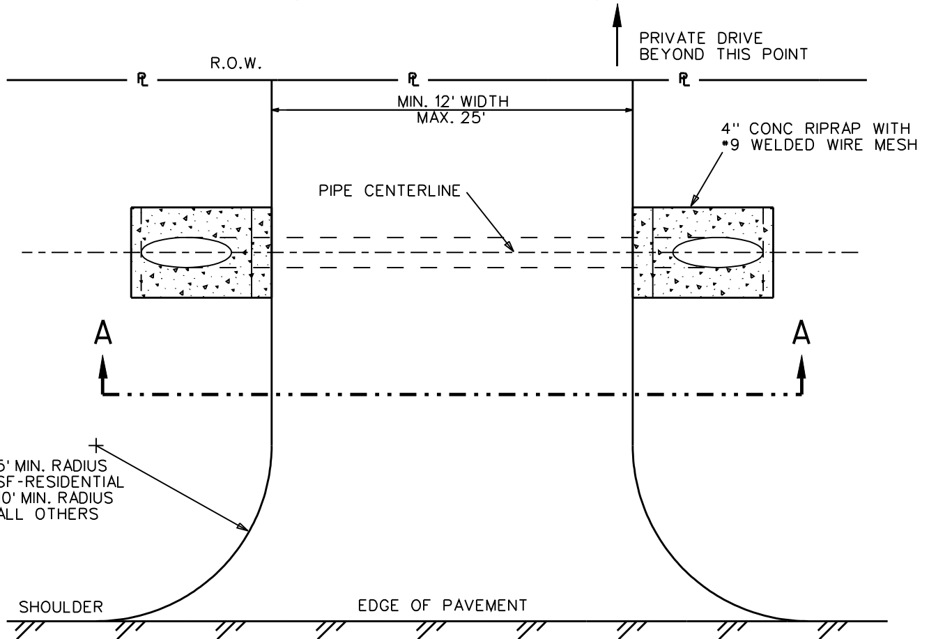
PLAN VIEW
