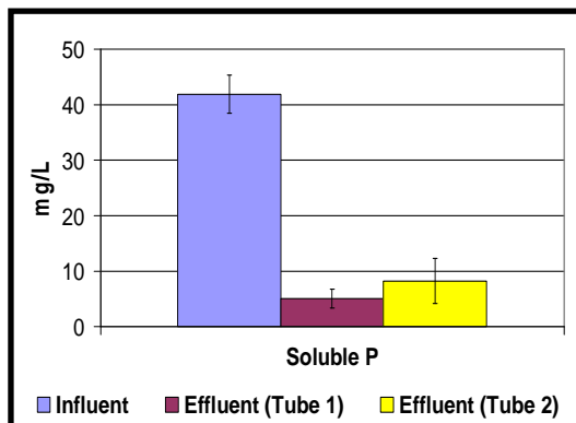
Figure 3.4 Soluble phosphorus reduction following Geotube™ treatment.
