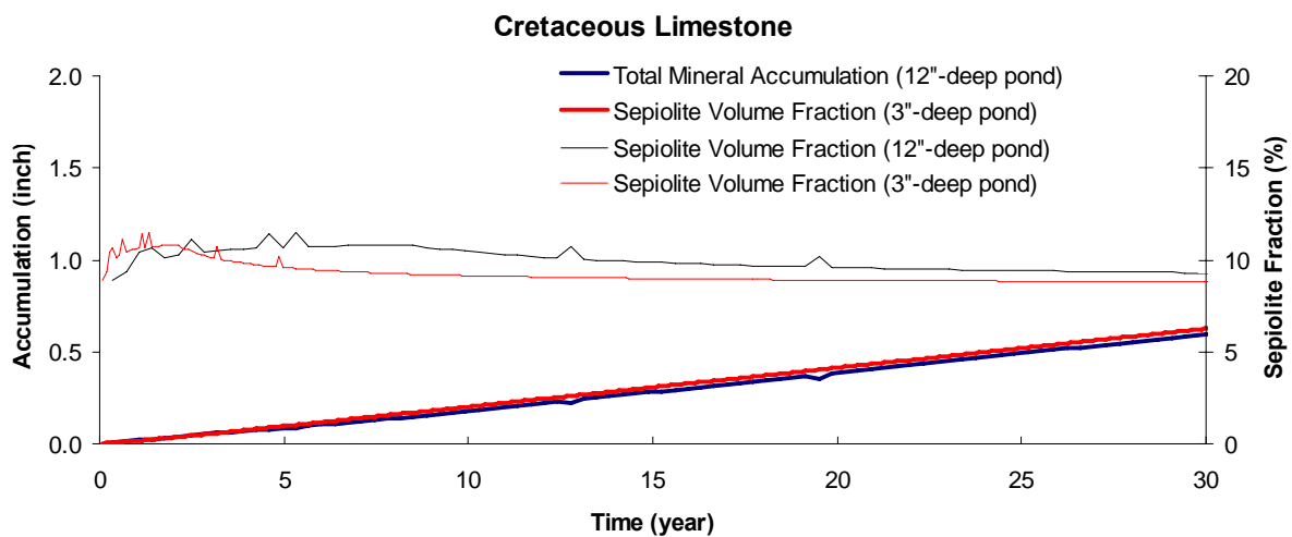
Figure 15-3. Specific accumulation (inches) and sepiolite fraction in accumulation for two pond depths (3 and 12 inches) for all water groups (continued)
