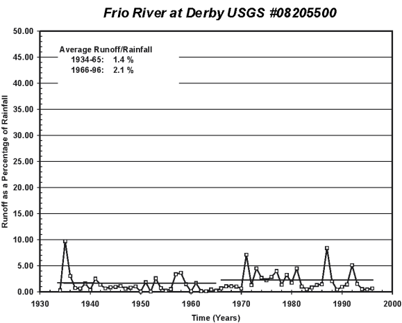
Figure 5-3. Runoff as a Percentage of Rainfall Time Series for Frio River Watershed
