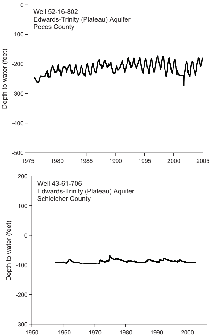
Figure 4-18. Hydrographs for two wells in the Edwards-Trinity (Plateau) Aquifer.
