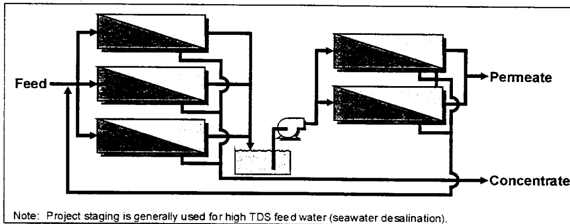
Figure 3-5. Schematic of Product Staging Pressure Vessel
