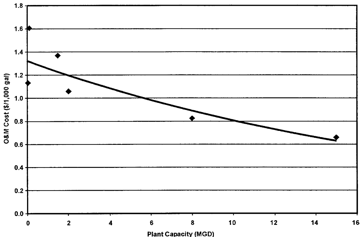
Figure 6-20. Groundwater Desalination O&M Costs
