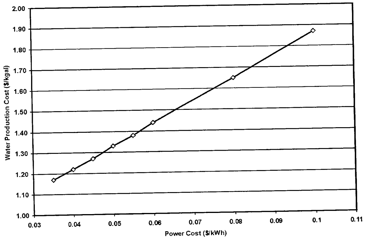
Figure 4-8. Reverse Osmosis Power Cost Impact
