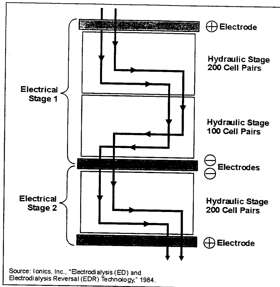
Figure 3-9. Electrodeionization Membrane Stack
