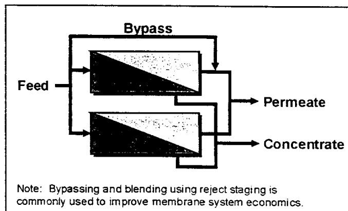
Figure 3-6. Schematic of Bypassing and Blending Pressure Vessel
