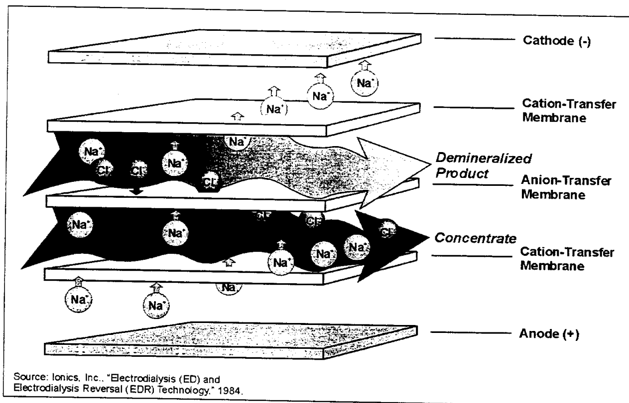
Figure 2-4. Simplified Diagram of an EDR Cell
