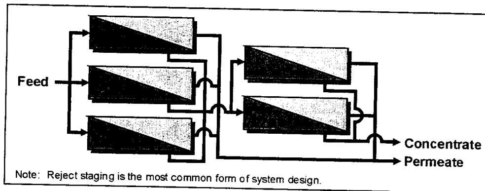
Figure 3-4. Schematic of Reject Staging Pressure Vessel
