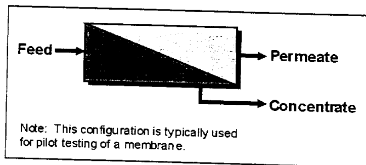
Figure 3-2. Schematic of Single Stage Pressure Vessel
