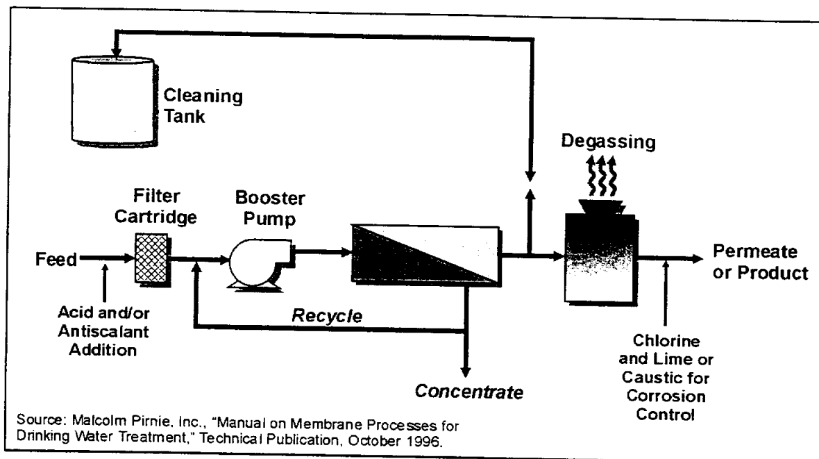
Figure 3-7. Reverse Osmosis Flow Schematic
