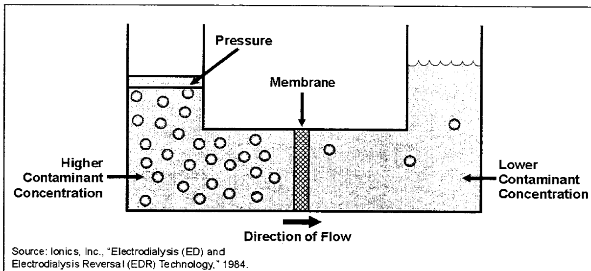
Figure 2-3. Reverse Osmosis Process
