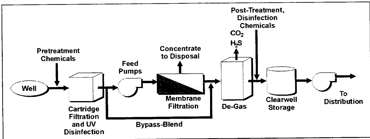
Figure 6-17. Typical Groundwater Desalination Schematic
