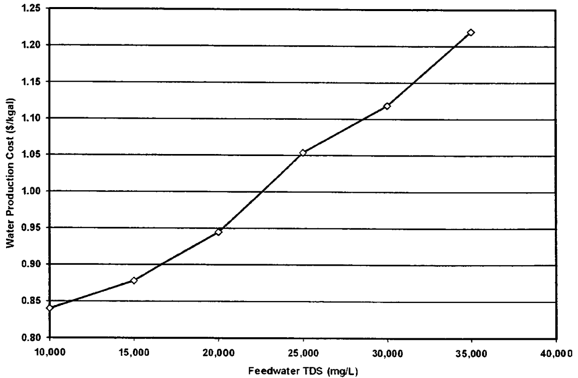
Figure 4-2. Reverse Osmosis Water Production Cost Versus Feedwater TDS
