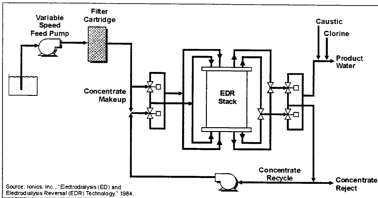
Figure 3-10. Typical EDR Flow Schematic
