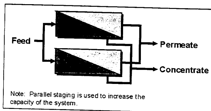
Figure 3-3. Schematic of Parallel Staging Pressure Vessel
