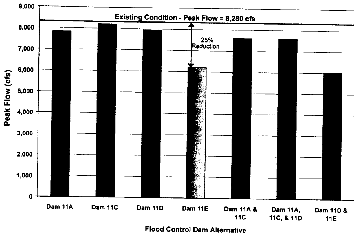
Figure 3.2-8 100-Year Peak Flow Reduction at California Street for Potential Flood Control
