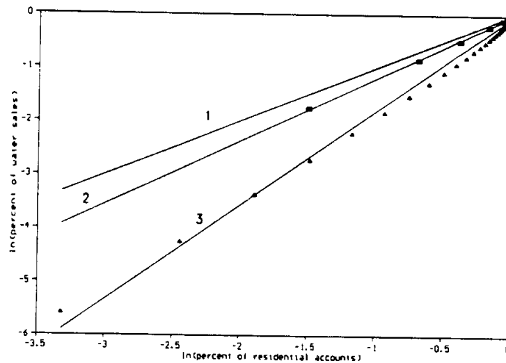
Figure 6.2 Logarithmic Transformation of Equation 4.1
