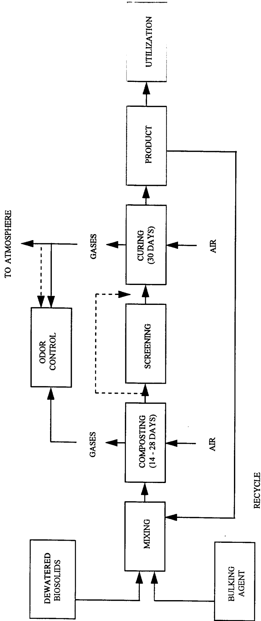
FIGURE 4-1 COMPOSTING GENERALIZED FLOW DIAGRAM
