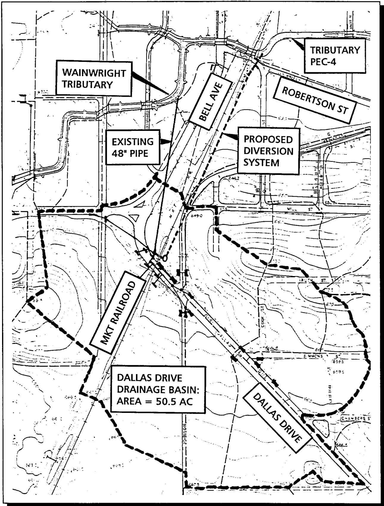
Figure III-18 - Dallas Drive Diversion System
