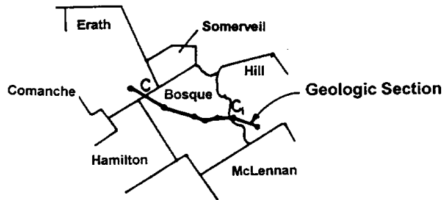
Geologic Section
