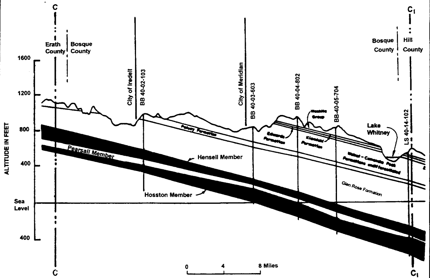
Geologic Section
