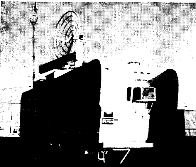
Upper: AI radar trailer and the antenna components for the C-band weather radar system, the main interrogator/transponder antenna for aircraft identification and tracking, and the VHF and UHF antennas for general communications. Center: The radar console, the "nerve center" during cloud seeding operations, and the radar trailer interior showing space for any visitors. Lower: View of the AI mobile weather radar facility at Mathis Field, San Angelo, Texas.
