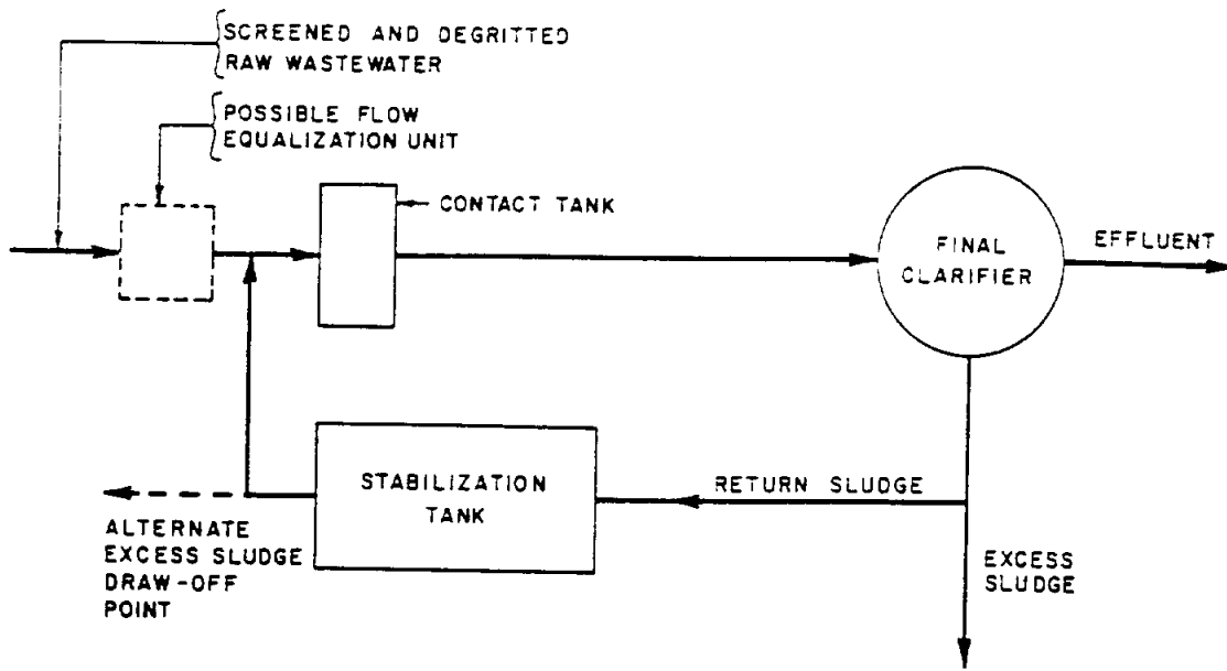
Figure 5-11 Contact-Stabilization Activated Sludge System
