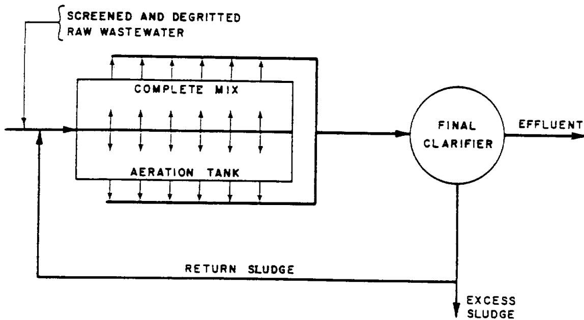
Figure 5-12 Completely Mixed Activated Sludge System
