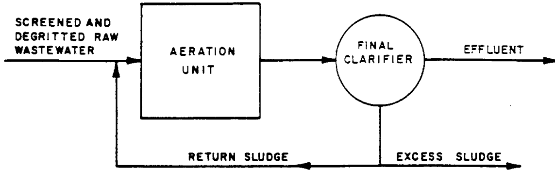
Figure 5-9 Extended Aeration Activated Sludge System
