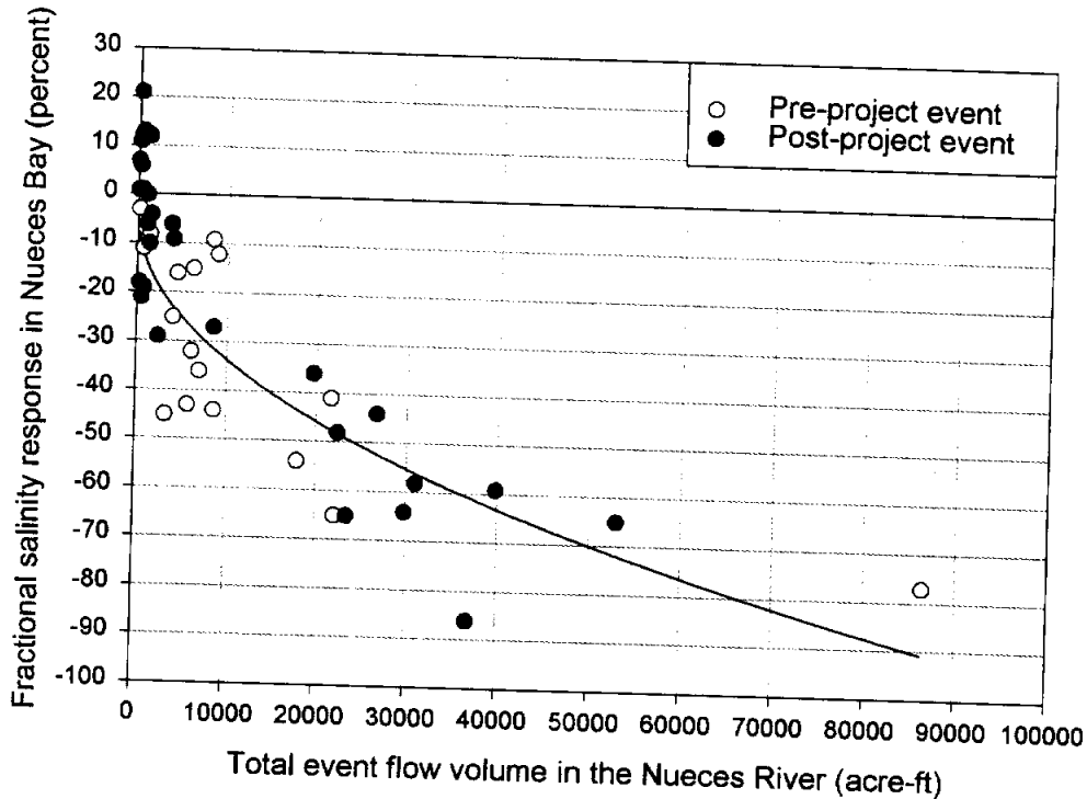
Figure 5: Fractional salinity response versus flow volume in Nueces River (measured at Calallen). Note: 1 acre-ft = 1.2336 \times 10^3 \text{ m}^3
