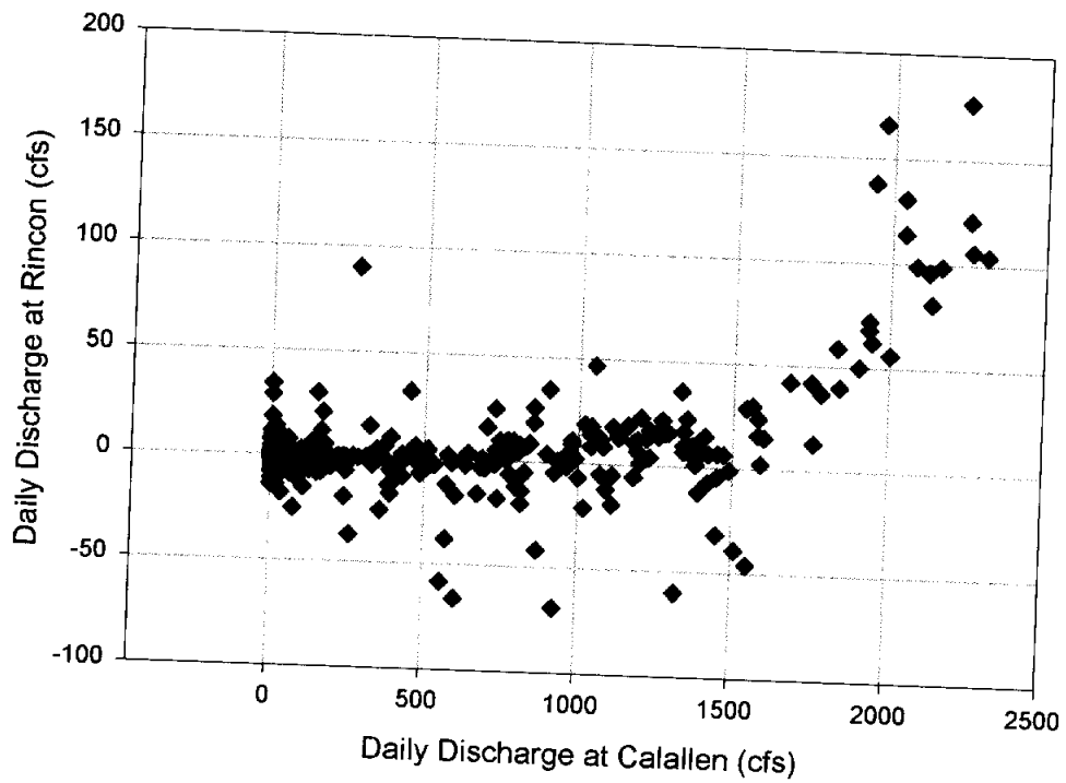
Figure 6: Plot of daily discharge values from the Calallen and Rincon gauges. May 16, 1996, through December 31, 1999. Flow in the Nueces River did not become the dominant factor determining the rate of discharge through the Nueces River Overflow Channel until it exceeded approximately 1,400 cfs.
