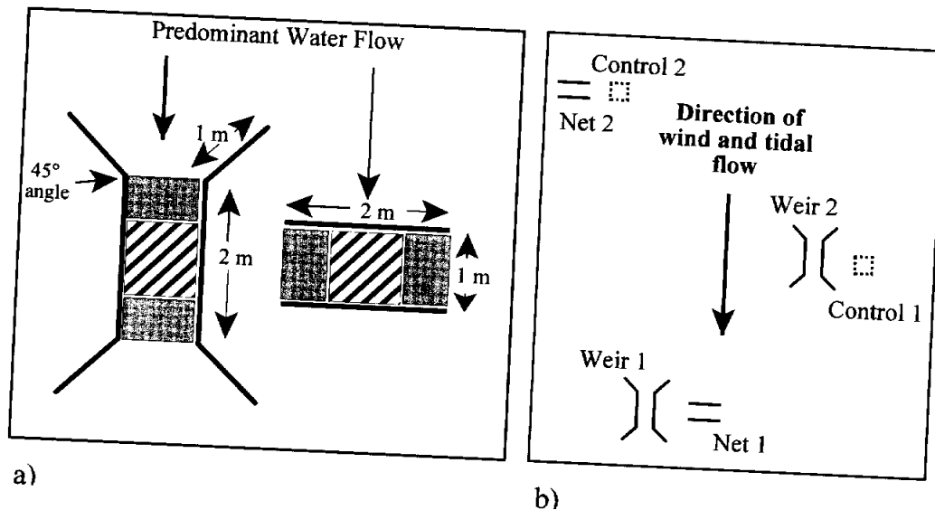
Figure 2: Flow alteration treatments for a) weir and net structure designs and b) field emplacement. Trays of defaunated sediment were randomly placed in hatched center regions. Undisturbed core samples were obtained in the shaded regions. Control plots were defined by corner posts (dotted lines).
