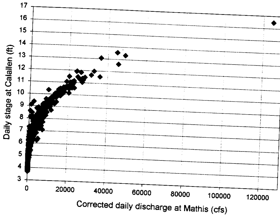
Figure 5: Regression analysis of corrected daily Mathis discharge and daily stage at Calallen.
