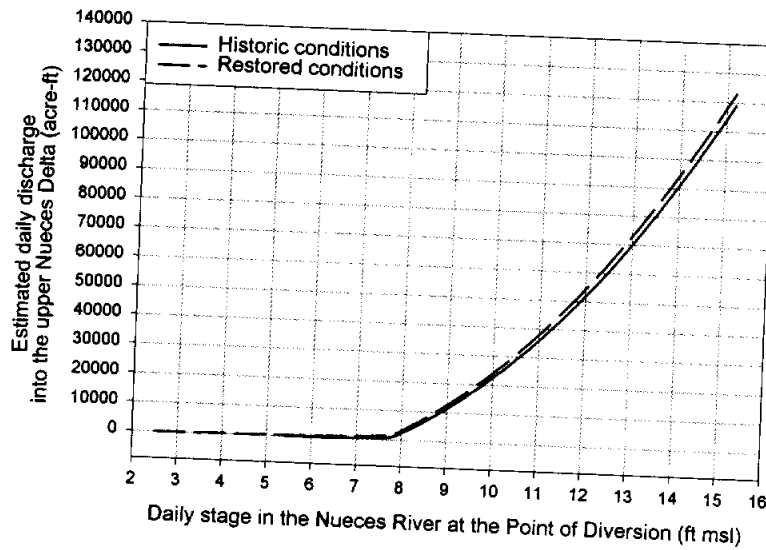
Figure 8: Stage-discharge rating curves for the Nueces River into the upper Nueces Delta, including both historic and restored conditions. Full range of stage values shown.
