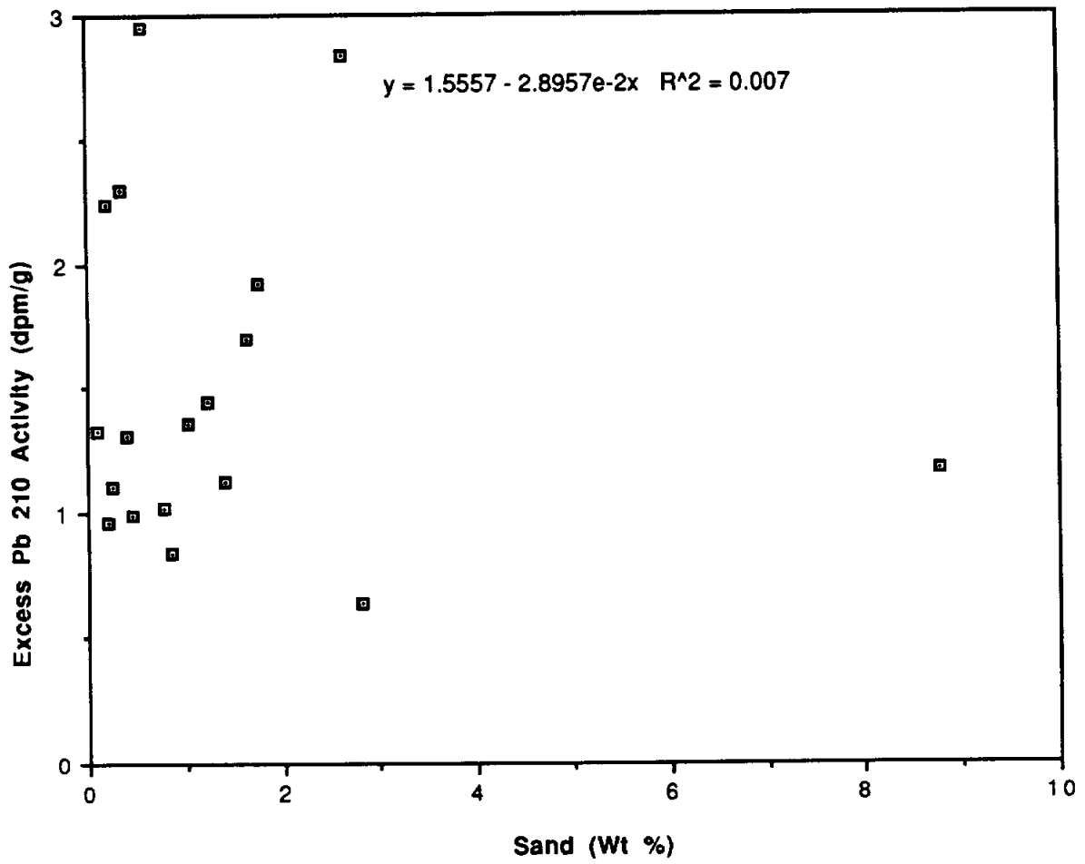
Figure 8. Relationship between sand percent and excess ^{210}\text{Pb} activity in core TR-11.
