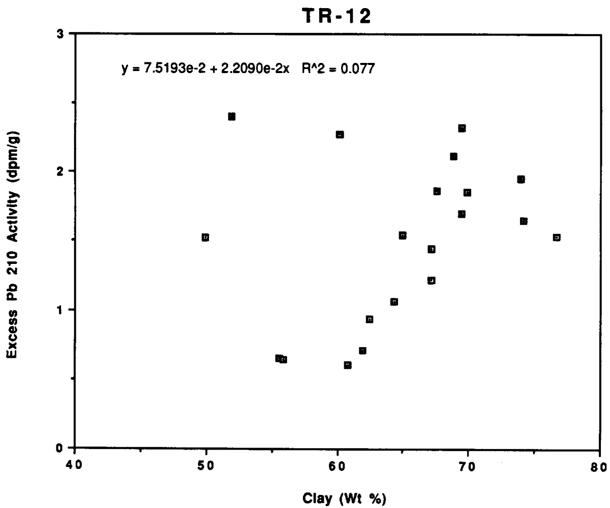
Figure 7. Relationship between clay percent and excess ^{210}\text{Pb} activity in core TR-12.
