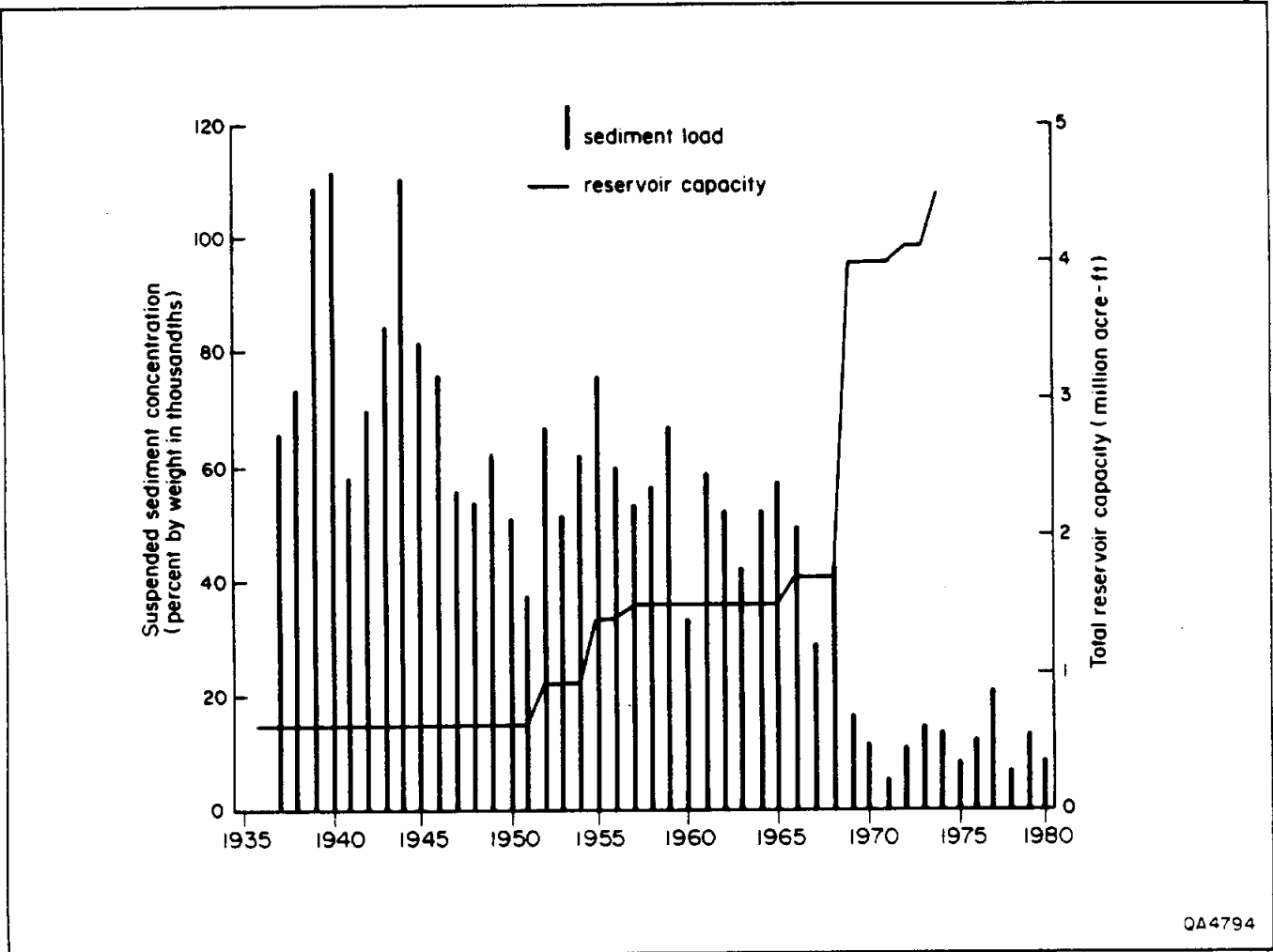
Figure 3. Suspended-sediment load (percent by weight) of the Trinity River at Romayor, and cumulative authorized water storage in reservoirs of the Trinity River basin. From Paine and Morton (1986).
