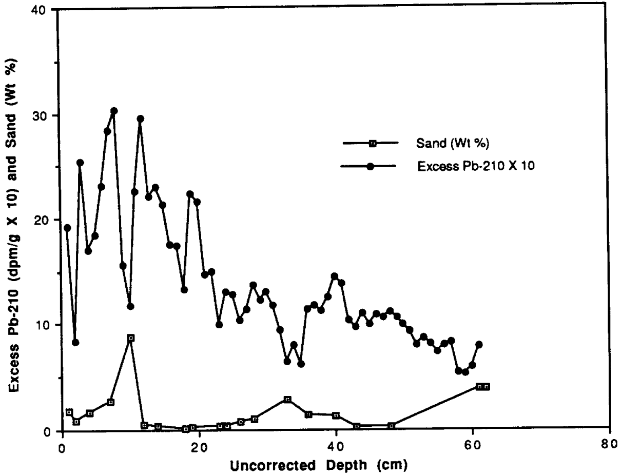
Figure 9. Depth plot of sand percent and excess ^{210}\text{Pb} activity for core TR-11. Note downward deflections in ^{210}\text{Pb} activity profile at 10 and 32 cm where sand percentage increases.
