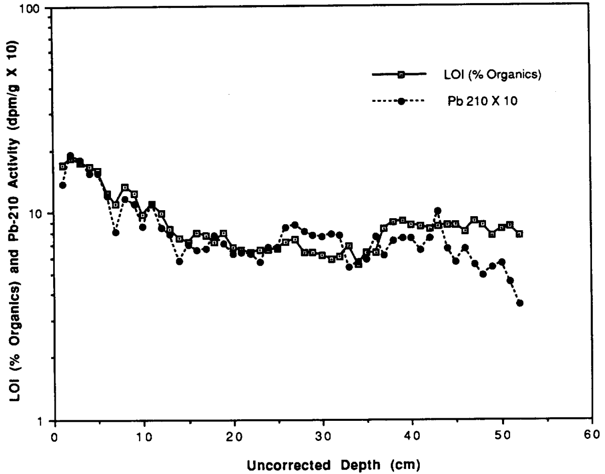
Figure 12. Relationship between organic matter (LOI) and ^{210}\text{Pb} activity profiles in core TR-9X. R^2 for ^{210}\text{Pb} and LOI for this core is only 0.771, but there is a relatively close relationship between the two profiles in some parts of the core.
