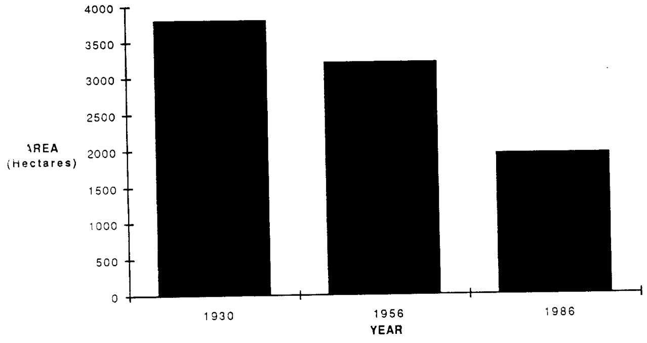
Figure 58. Index map and historical changes in vegetated wetlands, San Jacinto River delta and alluvial valley.
