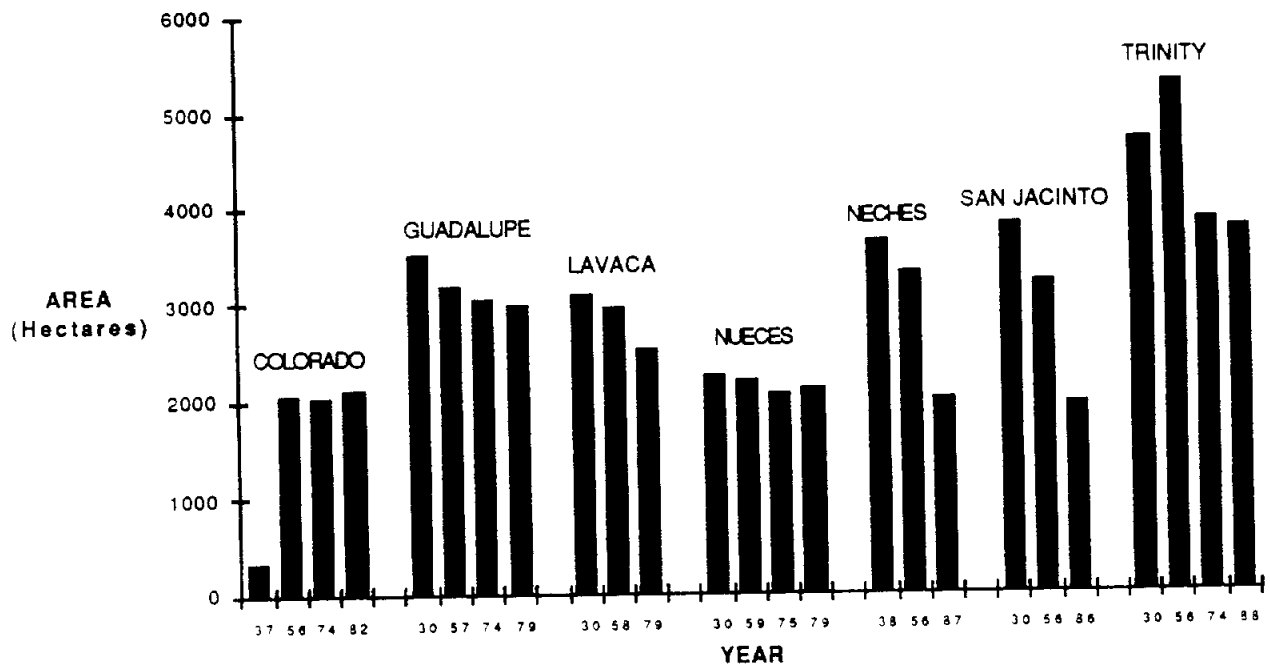
Figure 61. Summary of historical changes in vegetated wetlands in the seven fluvial-deltaic areas investigated.
