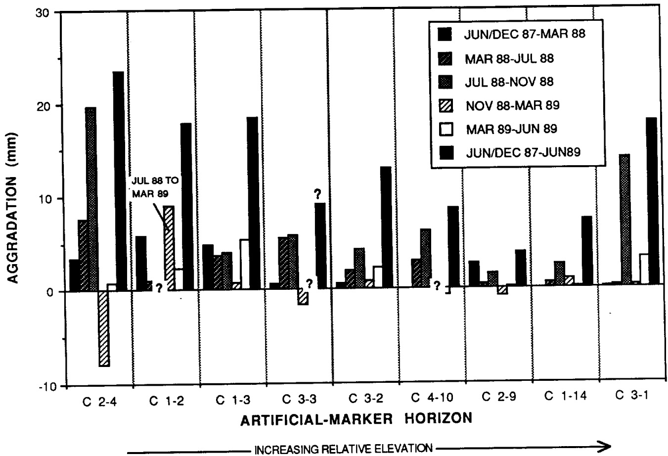
Figure 21. Sediment accumulation (aggradation) above artificial-marker horizons during specified periods, Colorado River delta study area. Marker horizons are arranged according to relative elevations.
