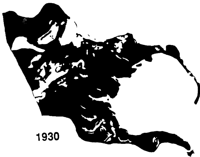
Nueces River delta index map and historical sequence of vegetated areas (in black) for the years 1930, 1959, 1975, and 1979.
