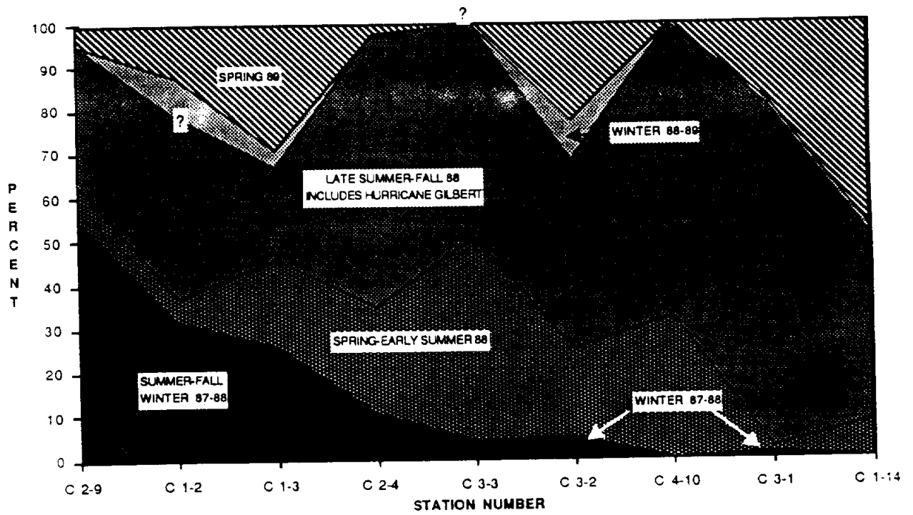
Figure 30. Seasonal aggradation in percent at all marker horizons from June/December 1987 to June 1989, Colorado River delta.
