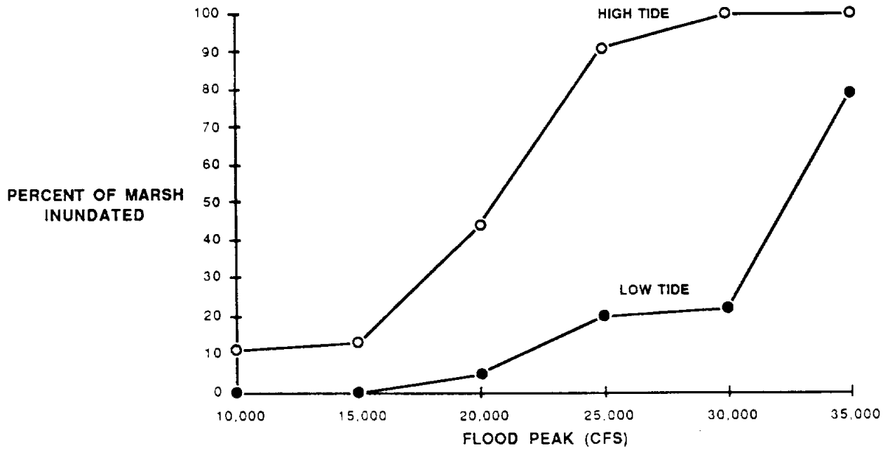
Figure 6. Simulated inundation of the Trinity River delta marsh versus peak discharge of the Trinity River under high and low tidal conditions. (From Texas Department of Water Resources, 1981).
