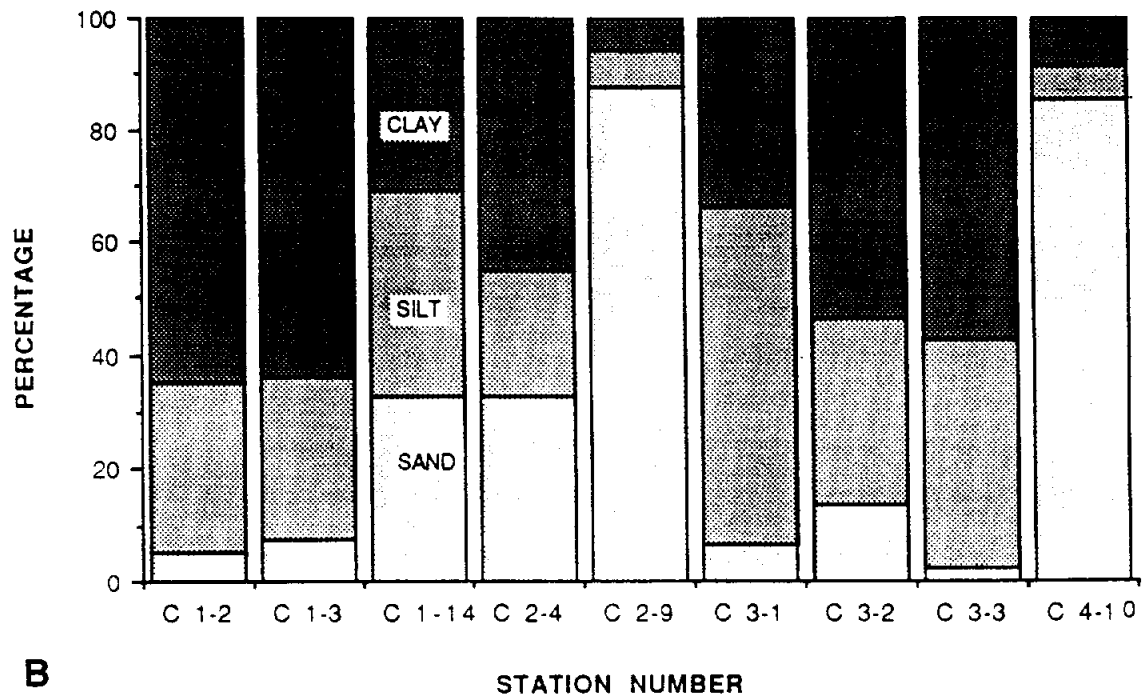
Figure 14. Percentages of sand, silt, and clay in sediments collected near selected stations in the Colorado River delta. Sediments were collected in March 1988 (A), and July 1988 (B).
