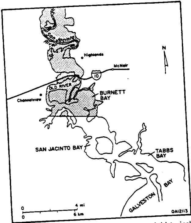
San Jacinto River delta index map and historical sequence of vegetated areas (in black) for the years 1930, 1956, and 1986.
