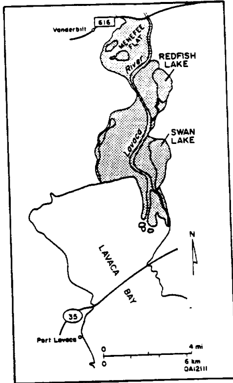
Lavaca River delta index map and historical sequence of vegetated areas (in black) for the years 1930, 1958, and 1979.
