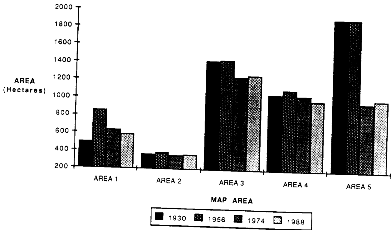
Figure 60. Historical changes in vegetated wetlands in five areas of the Trinity River delta. Refer to the index map in figure 59 for location of map areas.
