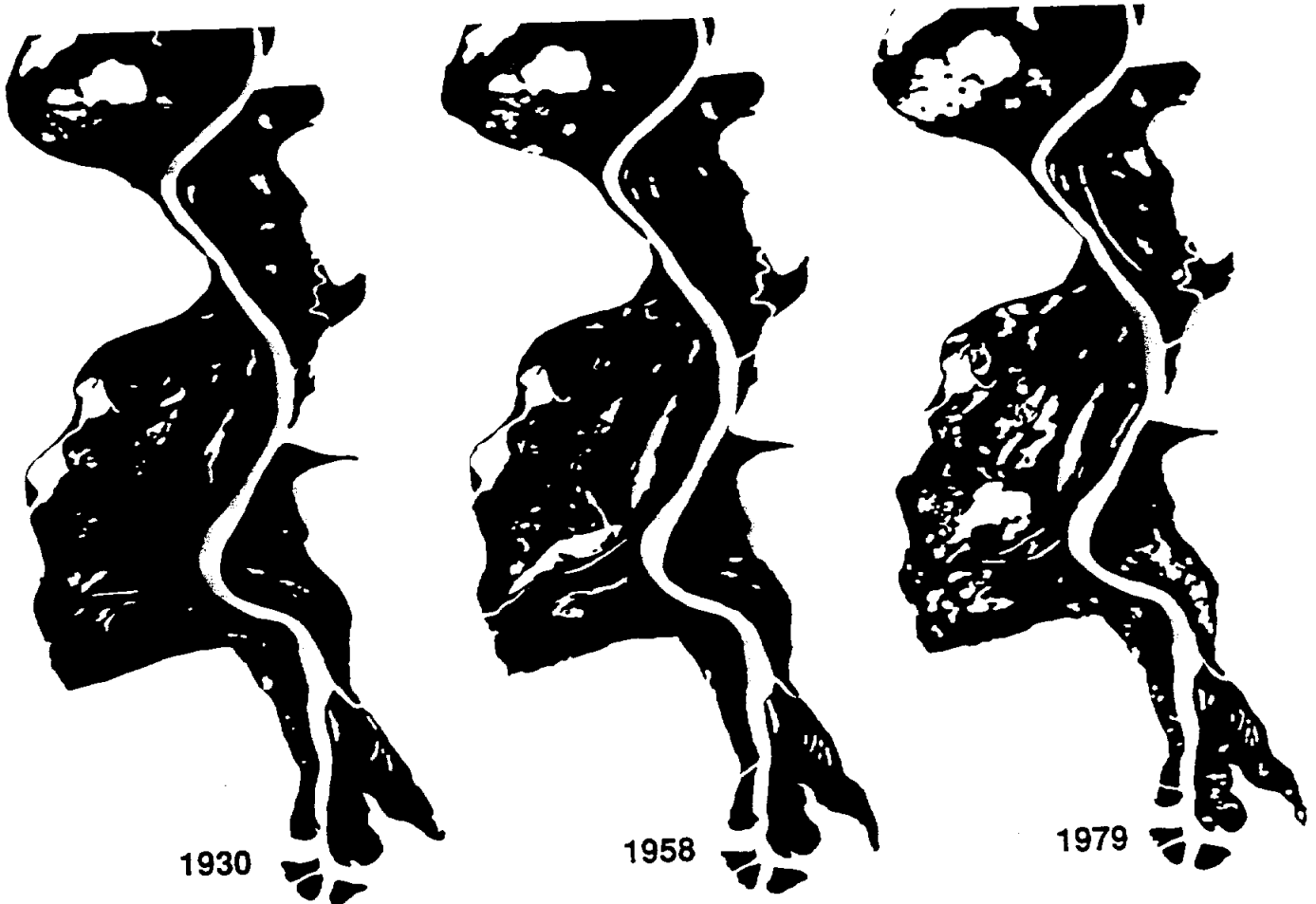
Lavaca River delta index map and historical sequence of vegetated areas (in black) for the years 1930, 1958, and 1979.
