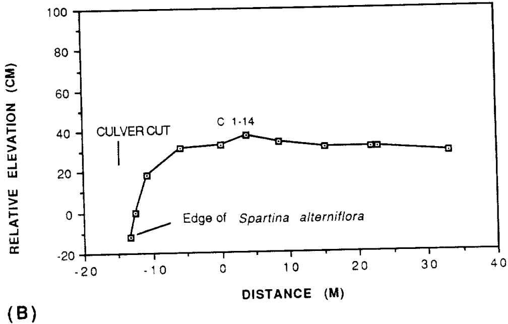
Figure 23. Profiles along marsh transect C 1 near Culver Cut, Colorado River delta. Profile (A) extends from south to north with the south end intercepting a storm berm that borders the marsh boundary along Matagorda Bay; artificial-marker horizons C 1-2 and C 1-3 are located along this profile. Profile (B) extends from the margin of Culver Cut eastward toward the north end of profile A. Marker horizon 1-14 is located on profile B.
