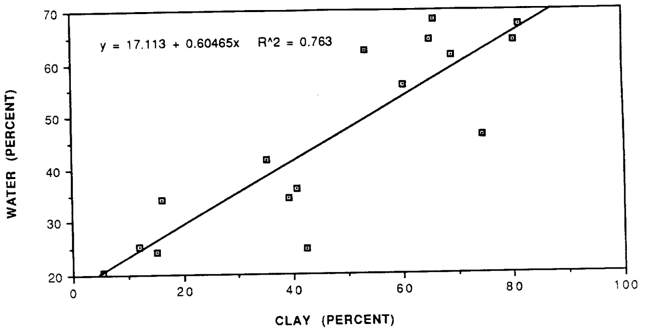
Figure 38. Scattergram and linear regression line for water content and clay in sediment at stations in the Colorado and Trinity River deltas. This high positive correlation is in agreement with numerous previous studies of water-soil relationships.
