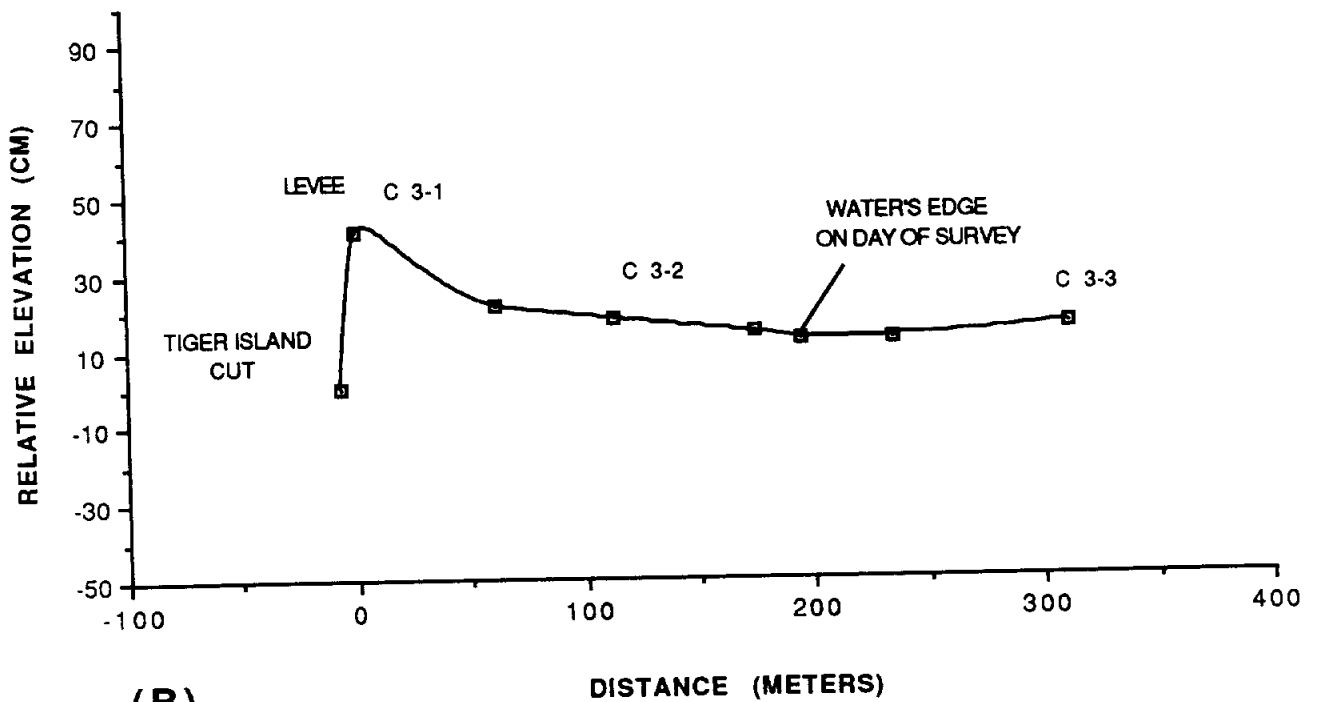
Figure 24. Profiles along marsh transect C 3 near Tiger Island Cut, Colorado River delta. Relative elevations (not adjusted to sea-level datum) determined with profiling rods along the initial 60 m (200 ft) of the transect are shown in (A); elevations based on plane table survey of about 300 m (1000 ft) of the marsh transect are shown in (B).
