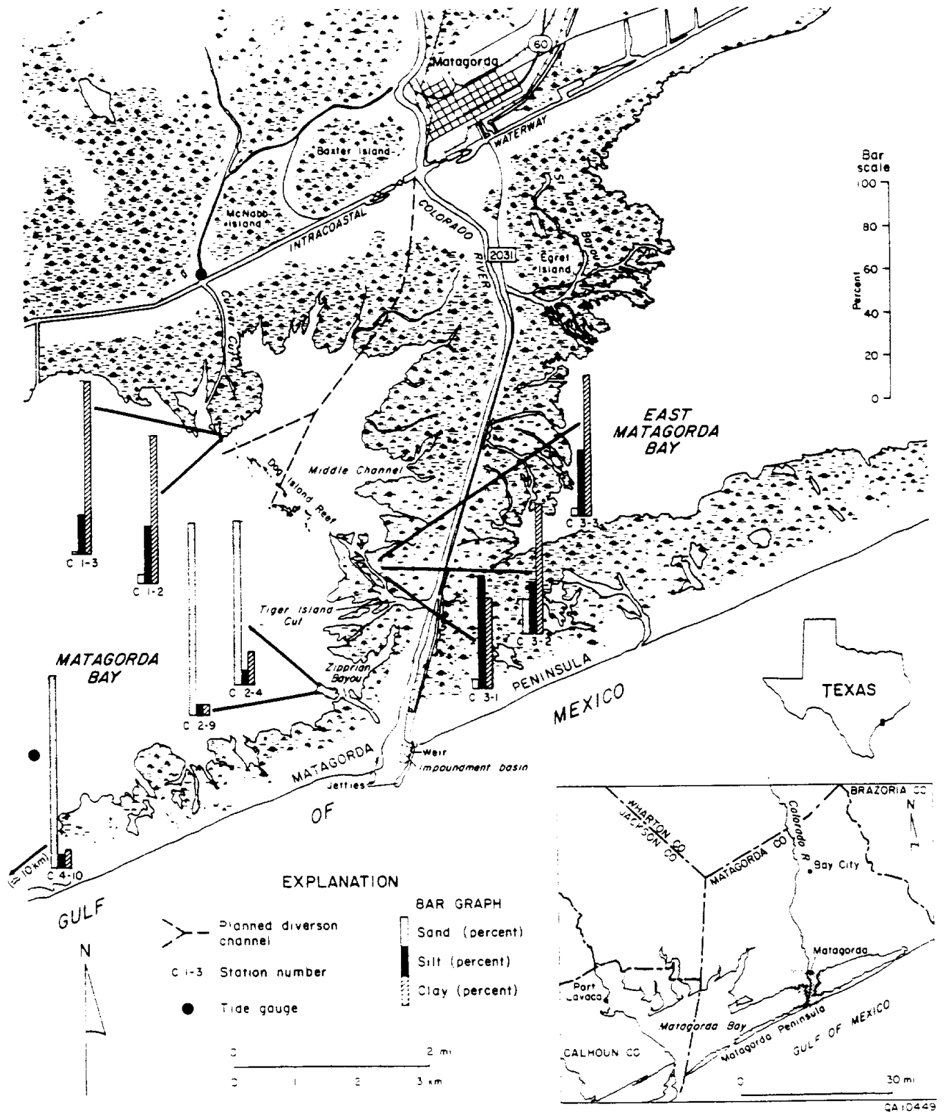
Figure 4. Index map of the Colorado River delta showing locations of profiling and vegetation transects, sediment textural composition, and tide gauge locations. The first number in the station identification code identifies the marsh transect, and the second number the artificial-marker horizon along the transect. Textural data are based on analyses of samples collected in March 1988.
