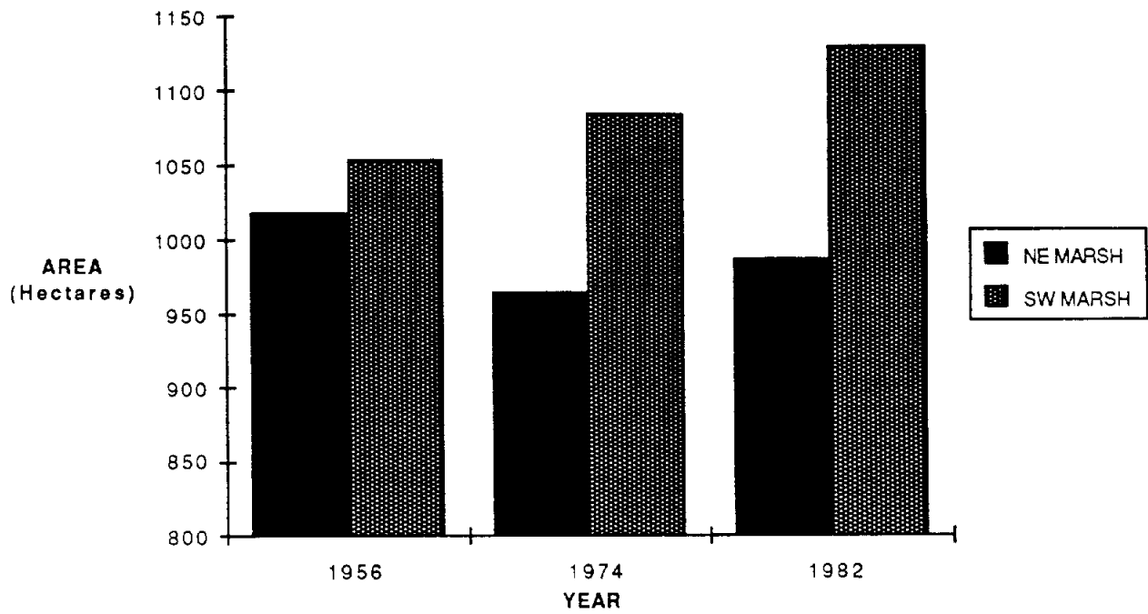
Figure 50. Comparison of historical changes in deltaic marsh areas northeast and southwest of the Colorado River. See index map in figure 49 for marsh areas.
