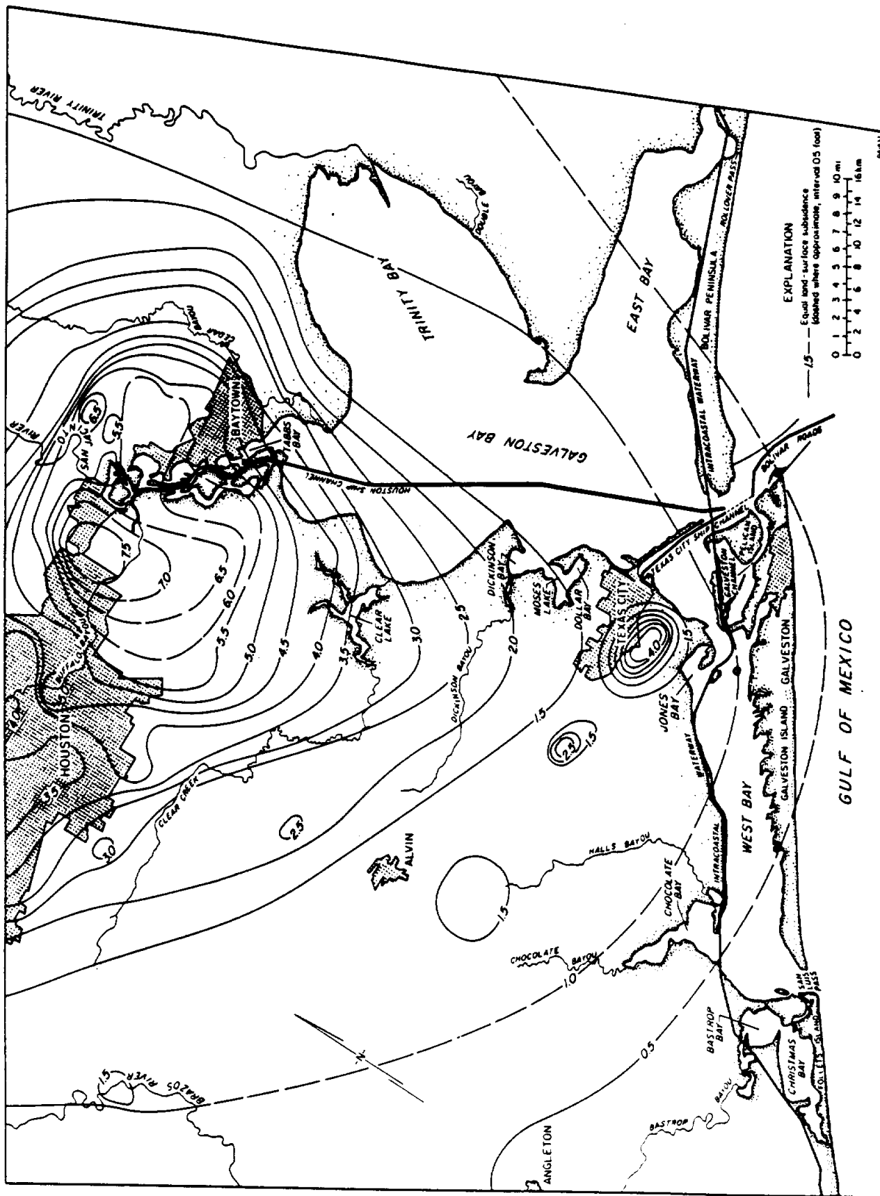
Figure 3. Land-surface subsidence in the Houston-Galveston area, 1943-1973. (From Gabrysch and Bonnet, 1975.)
