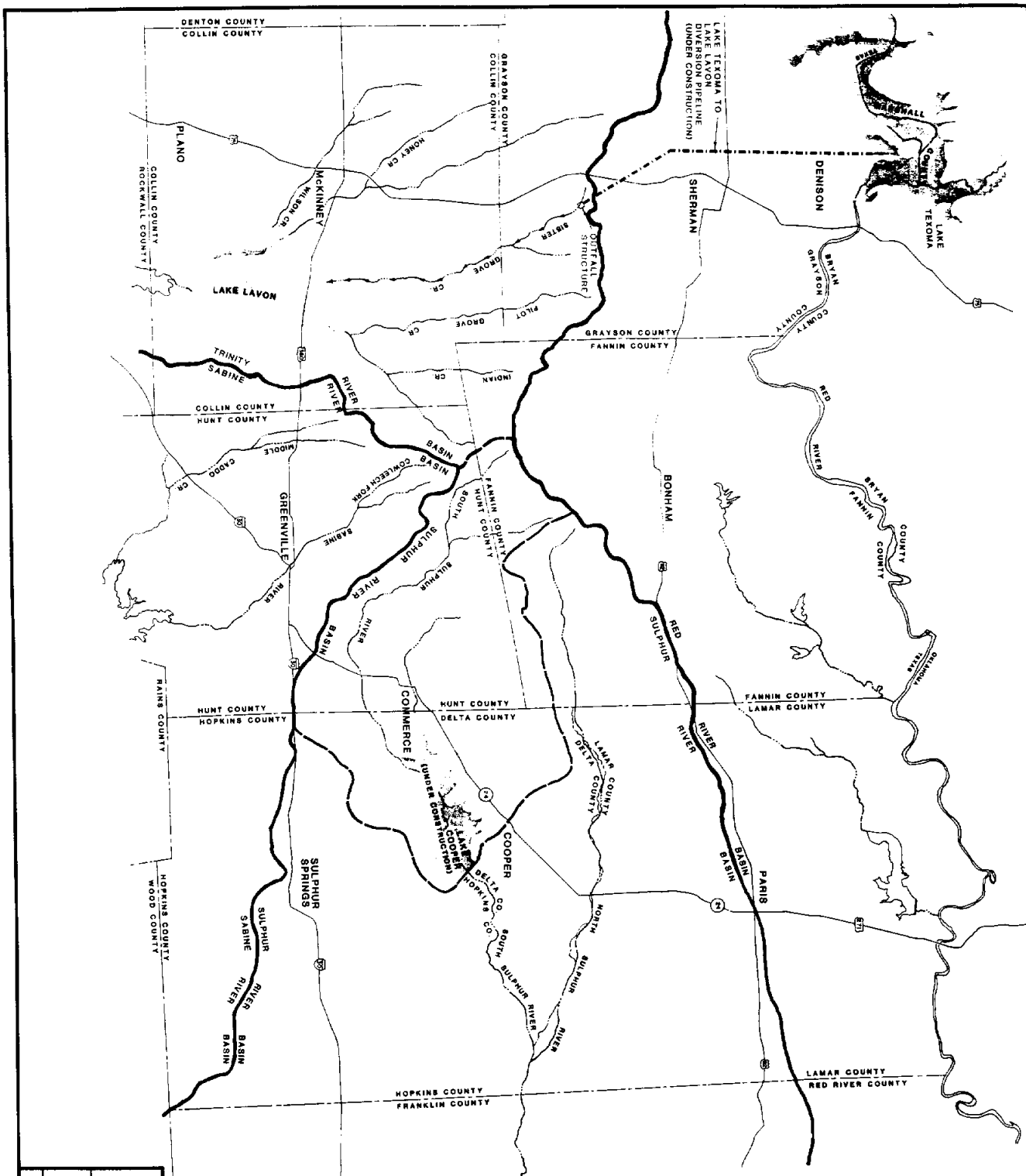
COLLIN COUNTY REGIONAL WATER AND WASTEWATER PLANNING STUDY SURFACE WATER SOURCES FIGURE V-2
