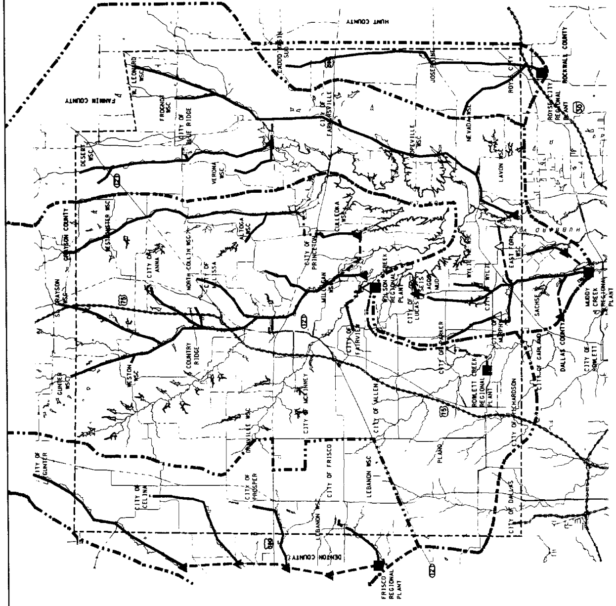
COLLIN COUNTY REGIONAL WATER AND WASTEWATER PLANNING STUDY WASTEWATER SERVICE PLAN OPTION 3 FIGURE XIII-4
