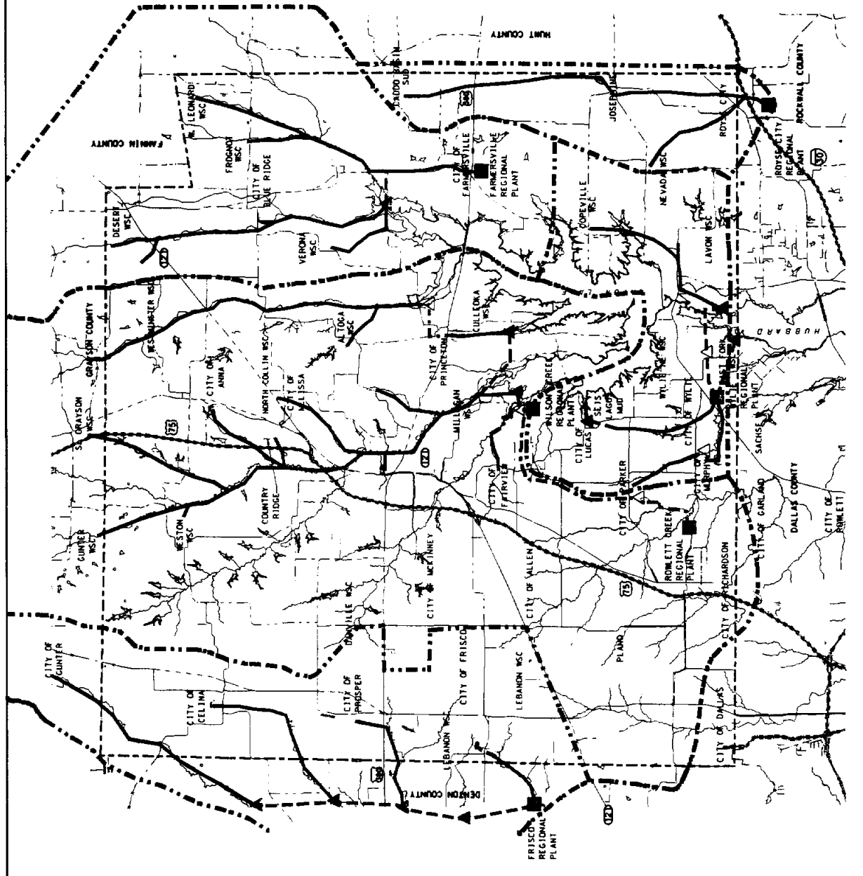
COLLIN COUNTY REGIONAL WATER AND WASTEWATER PLANNING STUDY WASTEWATER SERVICE PLAN OPTION 5 FIGURE XIII-6
