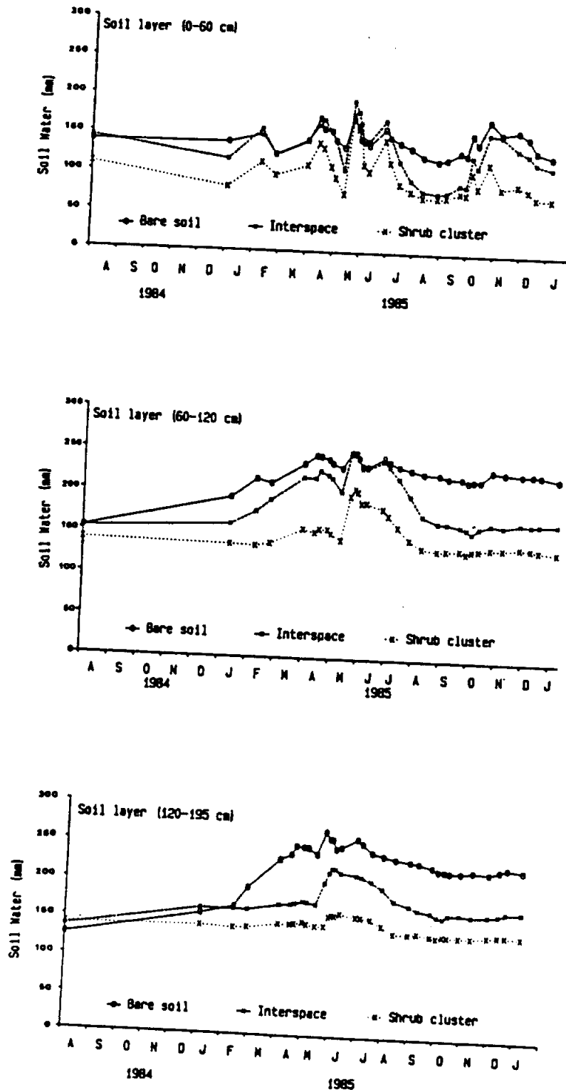
Figure 10. Soil water content for mesquite-dominated shrub clusters, herb-dominated interspaces, and bare soil on a sandy clay loam soil, La Copita Research Area, Alice, Texas.
