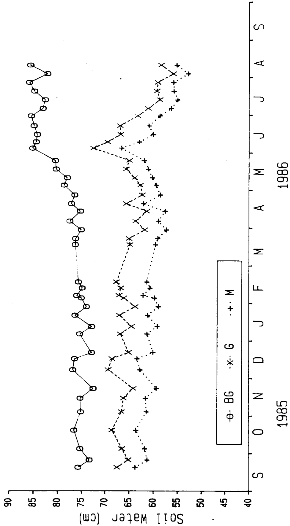
Figure 9. Total water in top 238 cm of the non-weighting lysimeters, Wagon Creek Spade Watershed Research Area.
