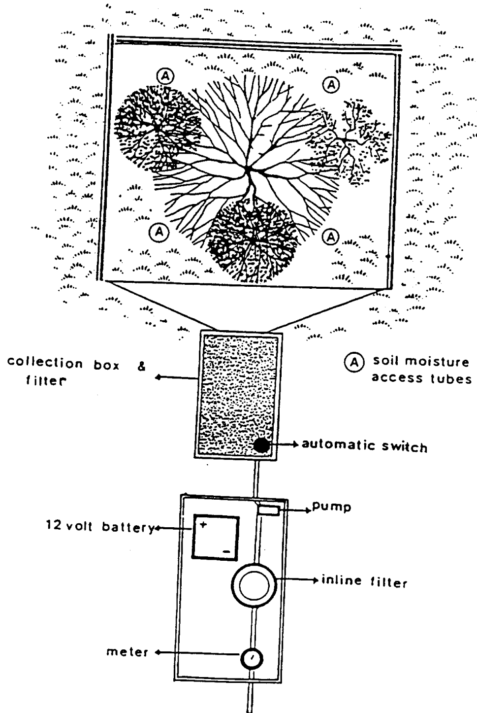
Figure 2. Generalized pland view of the non-weighting lysimeters for determining the water budget from mesquite-dominated shrub clusters, herb-dominated interspaces, and bare soil on the La Copita Research Area, Alice, Texas.
