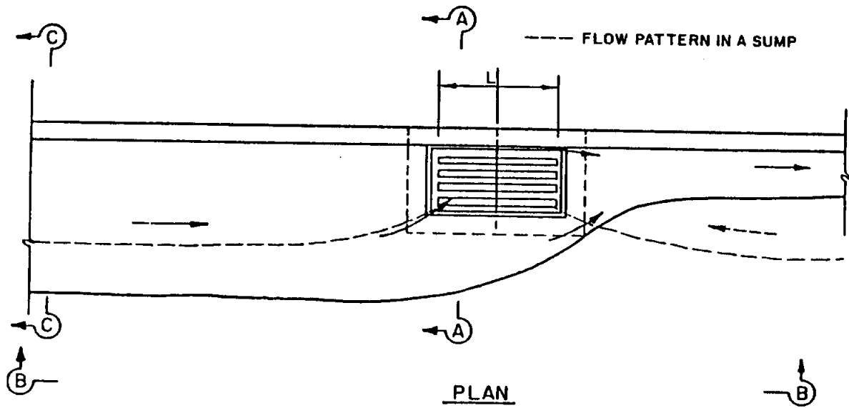
FIGURE 4-7 UNDEPRESSED GRATE INLET
