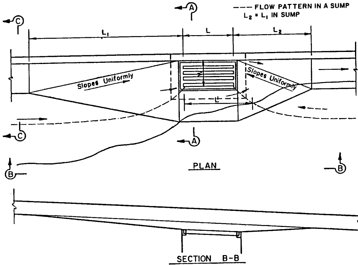
FIGURE 4-3 DEPRESSED GRATE INLET
